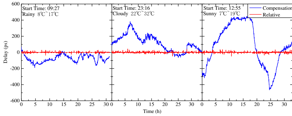
Fig. 2. Typical delay compensation (blue line) and relative delay between the arrival time of photons from Alice and Bob (red line) under different weather conditions. Measured by a TDC with time resolution of 4 ps, the standard deviations of the relative delay in (a), (b), and (c) are 6.7 ps, 6.0 ps, and 6.5 ps, respectively.
