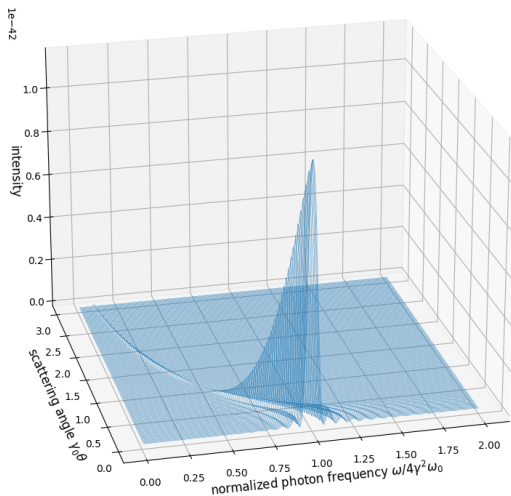
(a) Relative intensity distribution for \lambda = 132 nm
