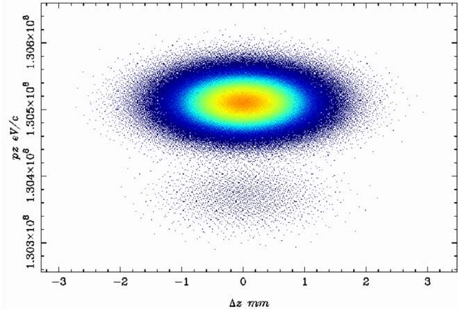
(b) Longitudinal phase space \Delta z/pz for 132 nm
