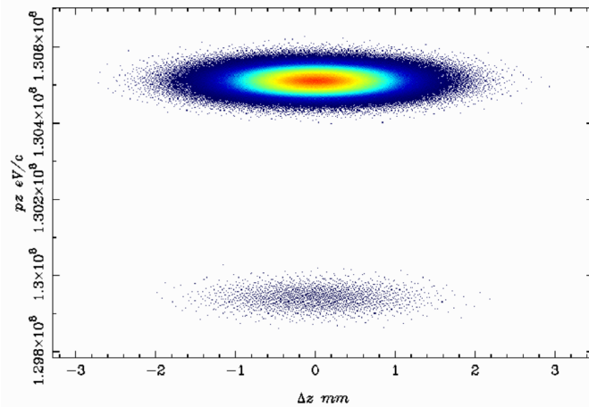
(b) Longitudinal phase space \Delta z/pz for 283 nm
