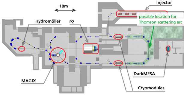
Figure 1: MESA layout as currently proposed. The green hatched area designates the components that would require modifications and areas that are likely candidates for diagnostics and measurement stations due to being currently unassigned. Image is an edited version of Fig. 1.2 in [1].
