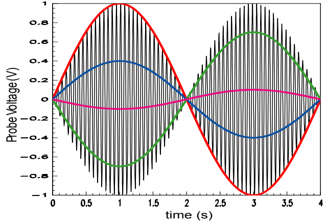
Figure 1: A simulated signal of slow rotating tangential probe (0.25 Hz) from a fast 16 Hz changing dipole field (black line). The color lines corresponds to the points with the same phases of the fast changing dipole field.
