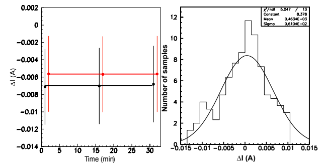
Figure 3: Average PS currents minus requested value versus time is shown on the left plot (long term DC stability). A distribution of the current difference between the measured AC (16 Hz sinus) minus the nominal values is shown in the right plot.
