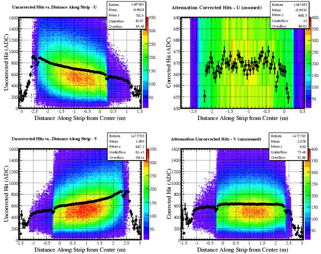
Figure 8.14: The distribution of hits as a function of distance along strip (MC). When there is no attenuation correction applied, the light levels are higher towards the read-out end of the strips. The drop-off at either end is due to the light lost at the end of the scintillator strips (this is cut out of the sample used). After the attenuation correction, the response across the length of the strips is flat (bottom right), even on a zoomed scale there is no residual dependency in this MC sample (top right).
