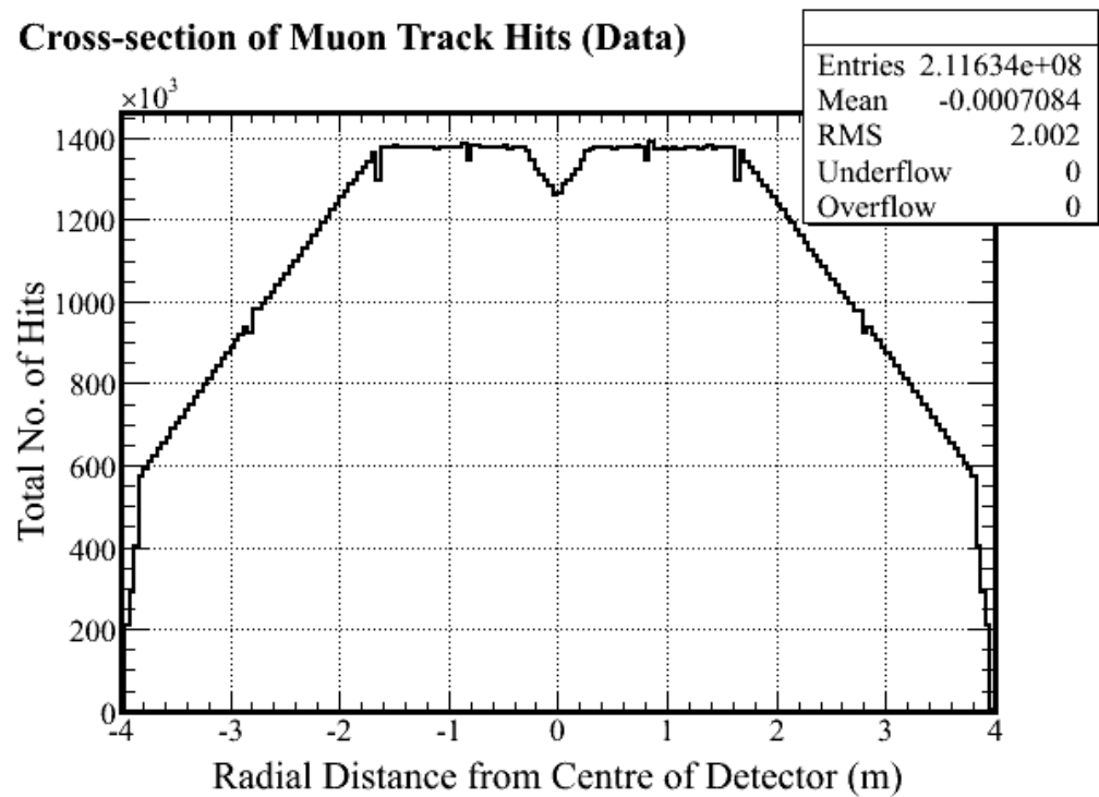
Figure 7.16: The octagonal cross-section of the Far Detector causes this radial pattern in hit locations for data over the whole detector. The dip in the centre is due to the coil hole. The pattern is repeated in MC (figure 7.15).
