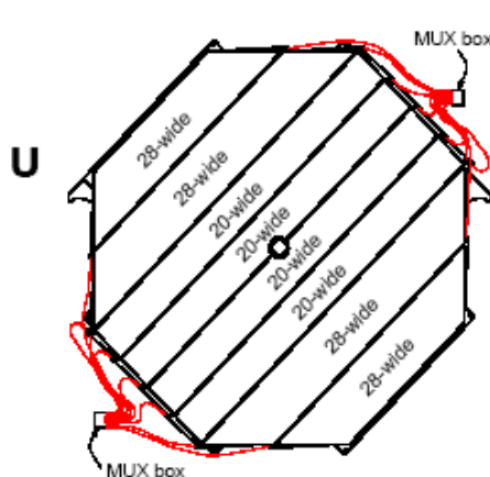
Figure 3.15: Representation of the Far Detector in MINOS software, showing orientation and strip-number starting position in the U-view (left) and V-view (right)
