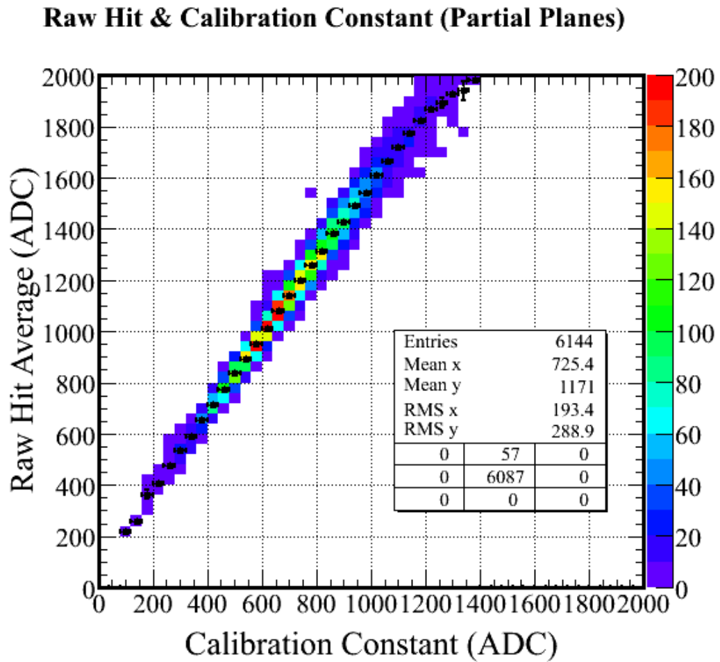
Figure 8.34: When the raw hit average is compared to the fully calculated calibration constant, there is an almost linear relationship, but with some scatter. This scatter and non-linearity proves the necessity for a method more complicated than just using the average raw hit, such as the one used here.
