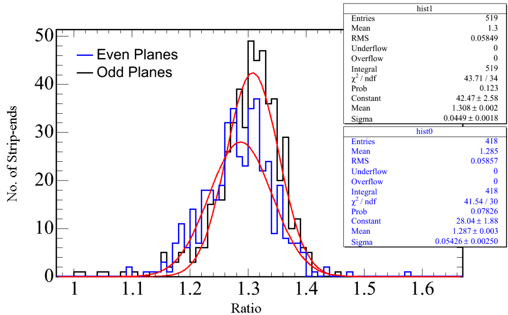
Figure 7.3: Histogram of ratios of peak to mean (optimal convergence values) for all strip-ends at CalDet from horizontal PS muons. The ratio is different for horizontal and vertical strips (odd and even planes) [81].
