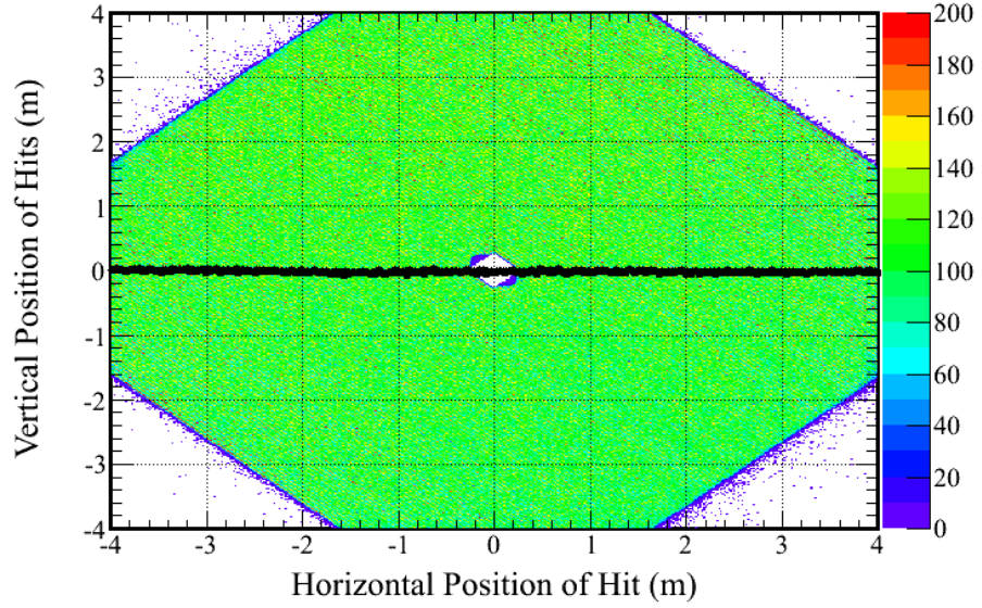
Cross-section of Hit Locations - U-strips, SM1
