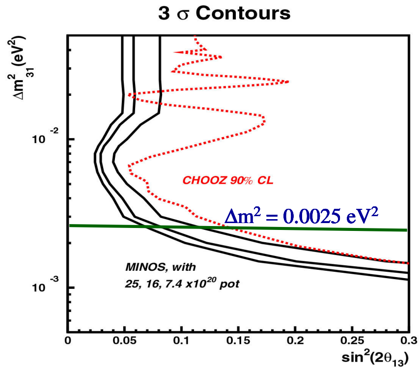
Figure 4.27: MINOS sensitivity to the reactor sector oscillation parameters with different numbers of protons on target compared to the Chooz limit. The plot assumes minimal mixing, below the MINOS limits.
