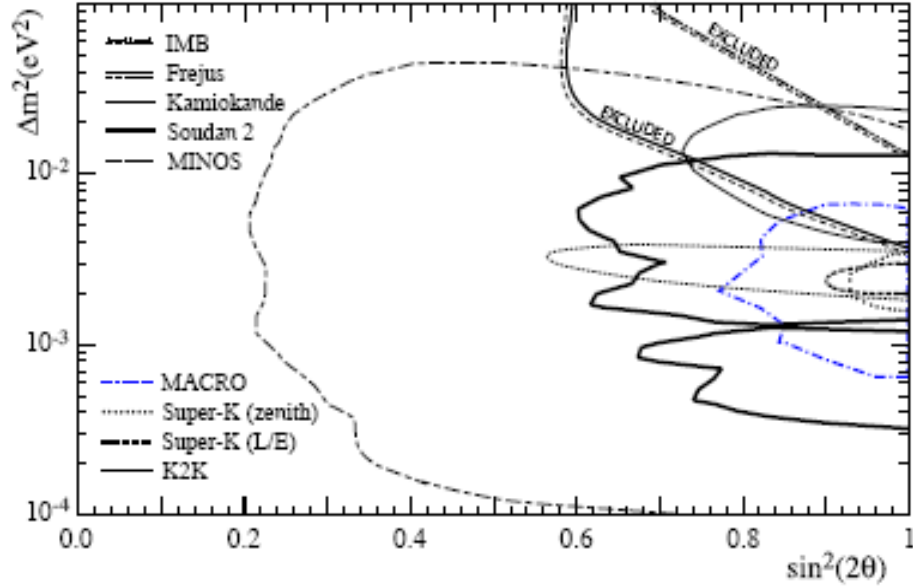
Figure 4.1: The MINOS parameter space shows the parameters measured with 77 neutrinos from the MINOS atmospheric neutrino analysis. The results are consistent with the other experiments shown. [A. Mann]
