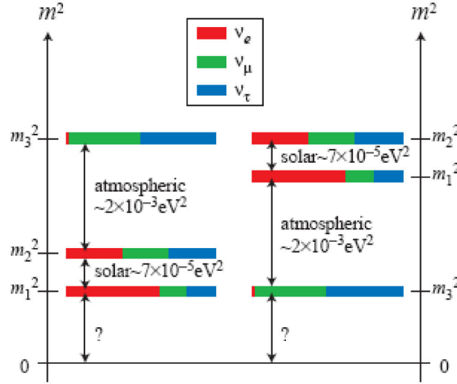
Figure 2.16: Neutrino mass hierarchy in the normal (left) and inverted (right) scenarios with the mixings also shown [6].
