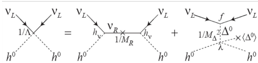
Figure 2.17: Exchange of GUT-scale particles in the see-saw mechanism to explain small left-handed neutrino mass [6].
