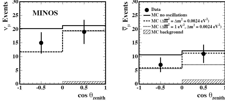
Figure 4.2: Upward- and downward-going \nu (left) and \bar{\nu} (right) atmospheric events at FarDet. The oscillation parameters do not differ between the two samples, with the current statistics.
