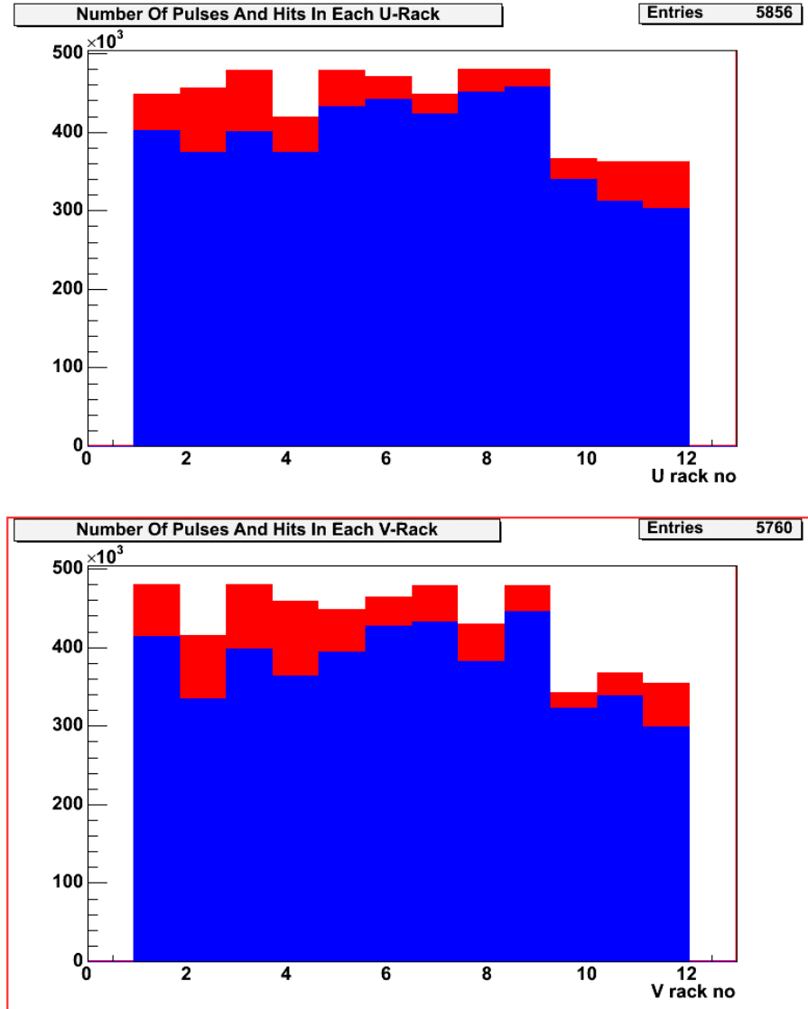
Figure 6.44: The number of LI pulses (red) and the number of correlated LI hits (blue) for each U and V electronics rack at NearDet from run 3612.
