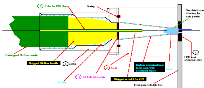
Figure 6.3: Diagram showing the cone assembly in which the LED shines on the LI fibres running to the PMTs and PIN photodiodes [65].
