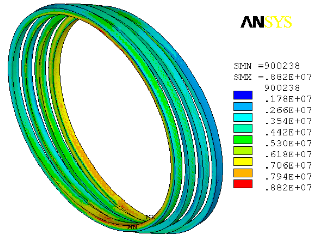
Figure 2: Coils stress at the peak current 14 kA.
