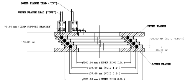
Figure 4: The model cross section.
