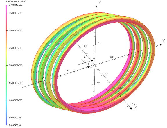
Figure 1: 4-Coil geometry and flux density.
