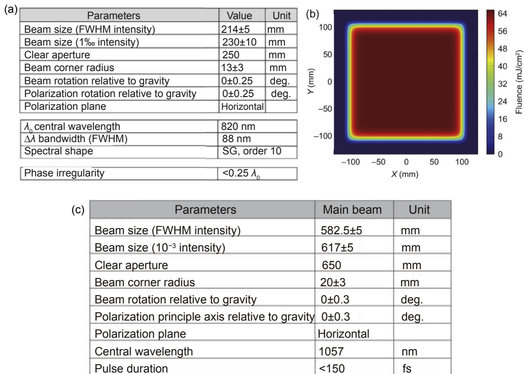
Fig. 20. (a) The basic parameters of the L3 laser beam. (b) The spatial profile of the square beam. The intensity follows I = \exp \left[ -2 \left( \frac{x}{w} \right)^G + \left( \frac{y}{w} \right)^G \right] with G = 20 , w = \left( \frac{2}{\ln 2} \right)^{1/G} \times \text{FWHM} and \text{FWHM} = 214 mm. (c) The basic parameters of the L4 laser beam.
