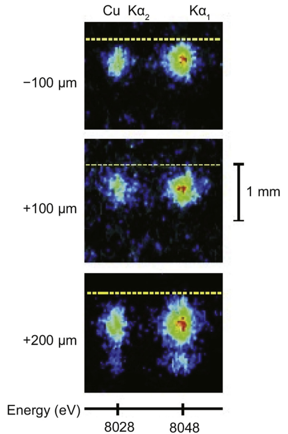
Fig. 36. Hot electron induced Cu K_{\alpha} emission observed at wedge-shaped massive copper targets. The focusing of the laser beam at variable distances above (negative value) and below (positive values) the target surface (yellow line) affects strongly the interaction conditions and the electron transport [168].
