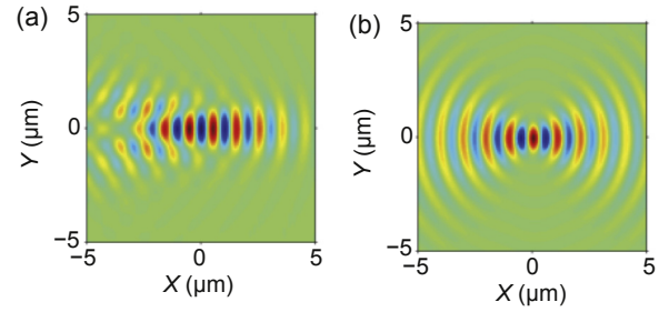
Fig. 30. A particle-in-cell simulation of a laser pulse focused down to a spotsize of 1 \mu\text{m} . (a) Using the paraxial approximation and (b) using the correct tight focusing approach. The time reversability of the Maxwell equations is violated in the paraxial approximation. Describing correctly tight focusing requires substantial modifications of the boundary conditions in kinetic simulation codes.
