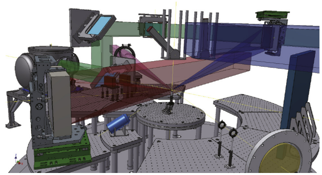
Fig. 24. A schematic of a potential layout for a sophisticated experiment to study WDM. A long pulse beam (ns duration) is used to drive a shockwave in a planar sample, while another ps-beam irradiates a thin foil from above producing X-rays for radiography which are detected transversally by a film pack below the target. The kJ short pulse beam is used to drive a K_\alpha source for simultaneous collective and non-collective XRTS detected by two curved crystals mounted from the upper breadboard inside the chamber. The shock velocity and self emission of the shockwave is recorded by VISAR and SOP diagnostics setup on an optical table outside the chamber (not shown in the diagram). Additional betatron diagnostic using a 30-fs beam focused inside an external chamber is also shown.
