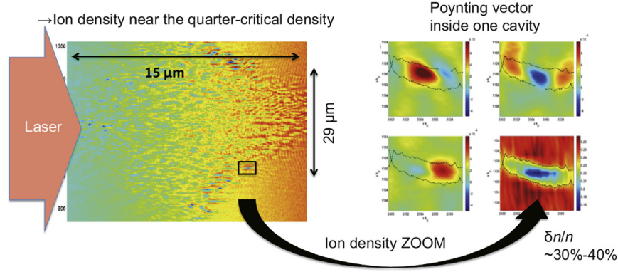
Fig. 27. An example of the complexity of the absorption process in the vicinity of the quarter-critical density. An intricate interplay of many parametric instabilities determines the absorption of the laser beam and the production of hot electrons. Even solitonic structures of limited lifetime play a role. The important conclusion is that for SI a substantial amount of the incident laser energy can be absorbed in the plasma corona rather than at the critical density. This affects the shock generated.
