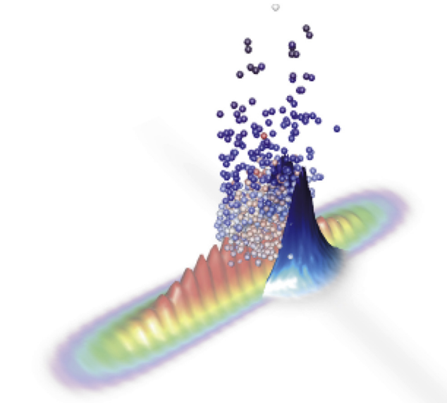
Fig. 34. Pair creation in laser-electron beam scattering. The blue surface represents the interacting electron beam density, while the newly generated pairs are shown as individual particles.
