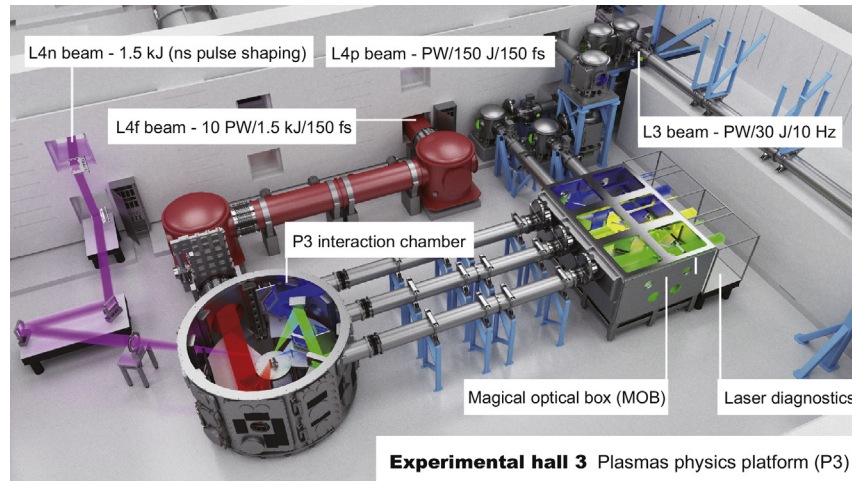
Fig. 15. Design picture of the expected final layout of the experimental hall E3. The details of the beam transport will probably change due to constructional constraints.
