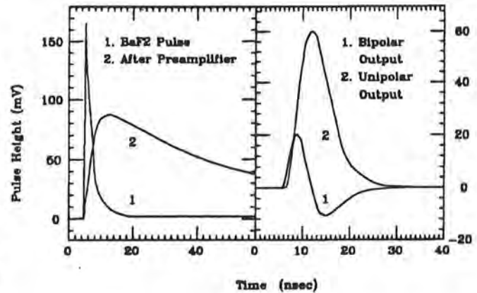
Fig. VI.3. BaF 2 readout pulse shape simulated with a PSPICE program: (a) input and after preamplifier, and (b) outputs.
