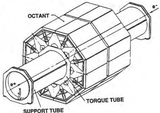
Fig. IV.3. The L3 muon detector contains 80 multisampling drift chambers in 16 independent modules. The total weight is 160 tons.
