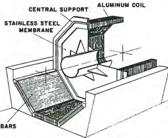
Fig.III.5. Mounting sequence of the aluminum coil.
