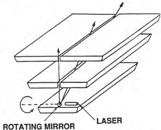
Fig. IV.10. The rotating laser beacon measures parallelism of the two octant centerlines to within 25 microradians.
