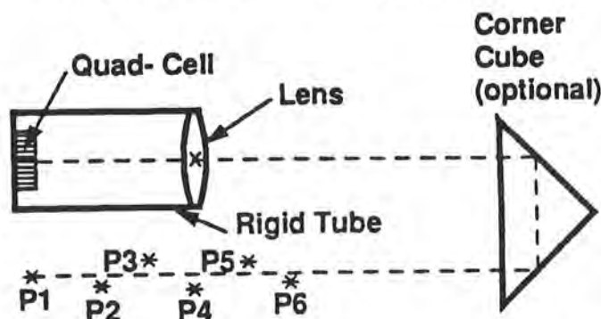
Fig. IV.23. Multipoint ( P_1 \dots P_6 ) alignment system, schematic.
