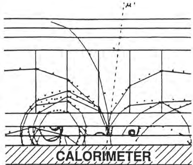
Fig. IV.1. Muon track with shower fragments. Calculation for 500-GeV muons using L3 GEANT 3.11 program of Ref. IV.1.
