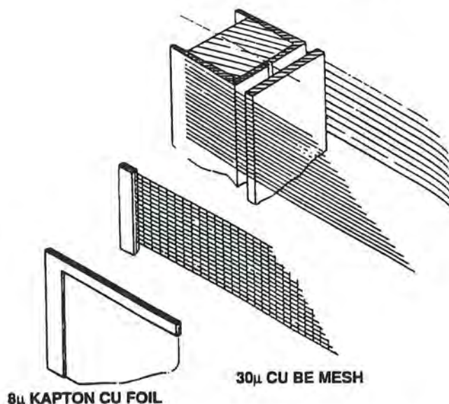
Fig. IV.19. Detail of wire attachment to the precision glass bridges showing a signal plane and a wire cathode plane. Replacement of the wire cathode plane by thin (8- to 30- \mu m) foil or mesh planes (R&D program) will increase chamber reliability.
