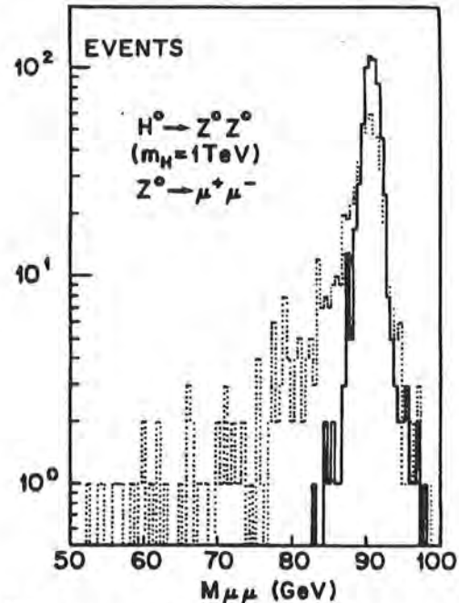
Fig.V.1. An example of deterioration of Z \rightarrow 2\mu mass resolution due to fluctuations of muon energy loss in the 12\lambda hadron calorimeter (dotted line). Correction for these fluctuations will be made by calorimeter sampling measurements (solid line). The reaction is pp \rightarrow H^0 (1 \text{ TeV}) \rightarrow ZZ \rightarrow 4\mu .
