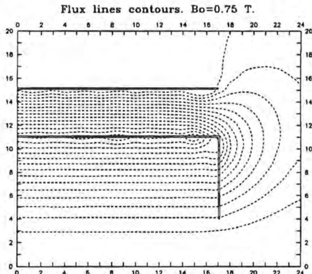
Fig.III.17. Map of the magnetic field for the superconductive coil with superconductive shield.
