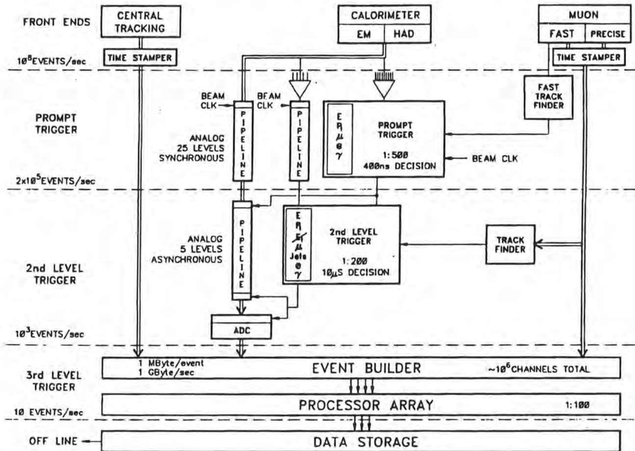
Fig. IX.3. Trigger architecture.
