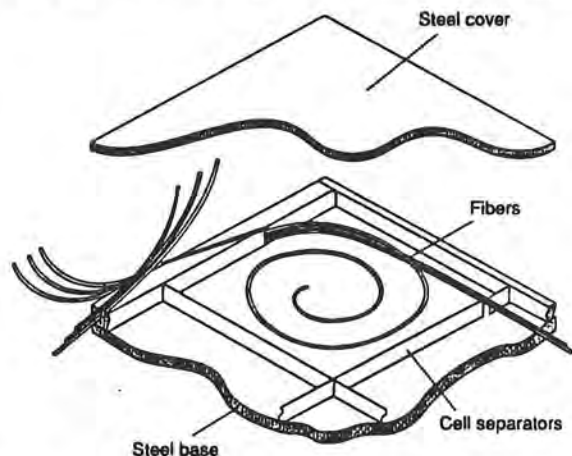
Fig. V.8. A cell of liquid scintillating calorimeter with WLS fiber readout.
