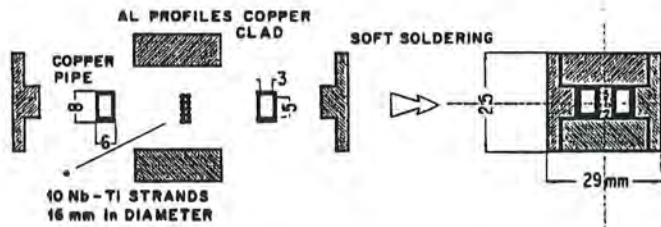
Fig.III.11. The conductor and its components.
