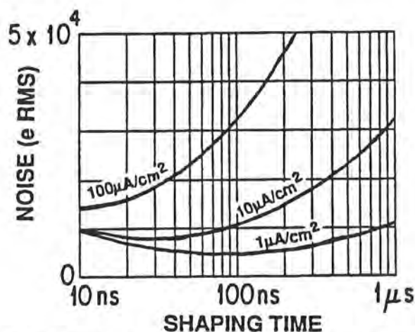
Fig. V.2. Amplifier noise vs shaping time and leakage current for bipolar preamplifier. Calculations are made for 500\text{ }\mu thick silicon detector with an area of 3 \times 3\text{ cm}^2 ; input capacitance 180\text{ pF} at full depletion.
