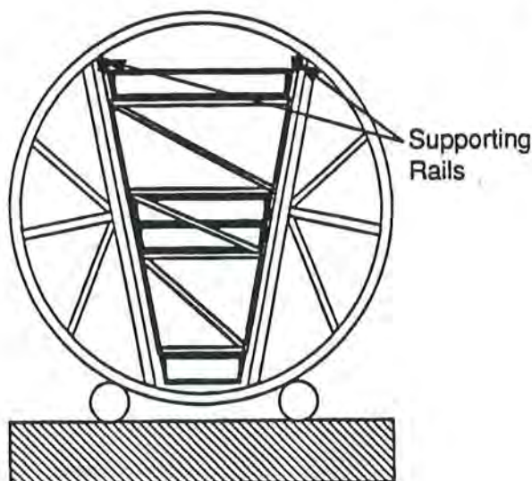
Fig. IV.26. Central region rotation and transport fixture.
