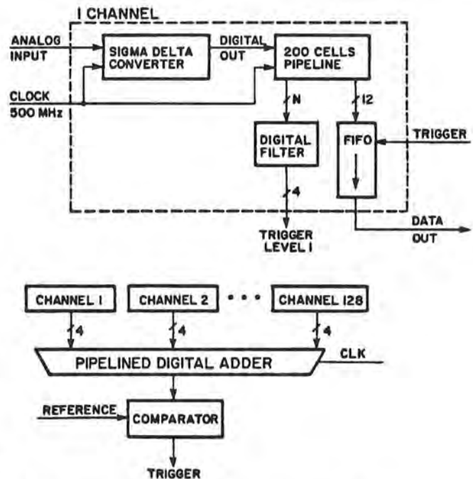
Fig. IX.2. Possible calorimeter level 1 trigger solution.
