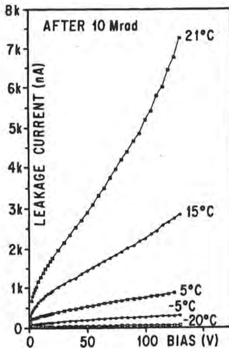
Fig. VII.6. Leakage current in silicon detectors after a 10 Mrad exposure to 800 MeV/c protons, as a function of detector temperature.
