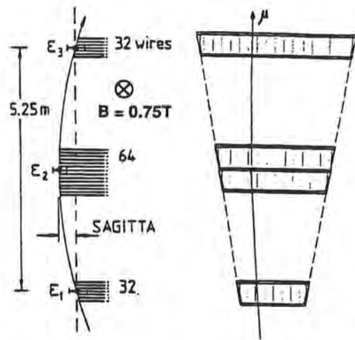
Fig. IV.15. Sagitta measurement in one radial module of the central detector ( B = magnetic field).
