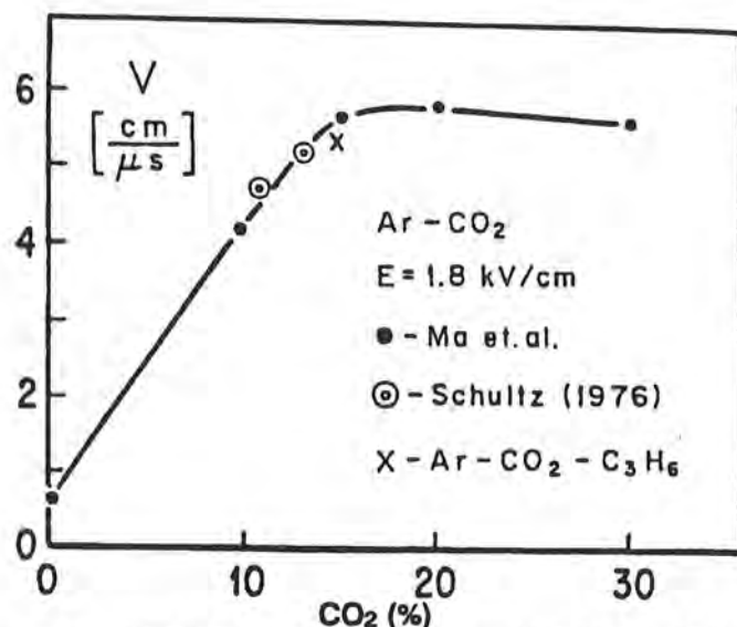
Fig. IV.22. Drift velocity ( v ) vs \text{CO}_2 concentration. The electric field E is 1.8 kV/cm.
