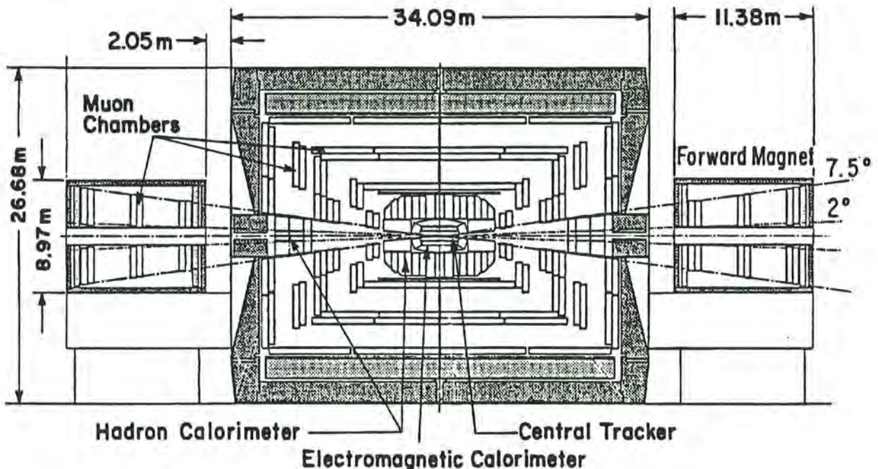
Fig. II.1. Side view of L*.
