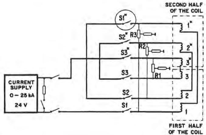
Fig.III.14. Energy dumping circuit.
