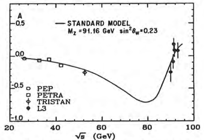
Fig. II.9 The measured forward-backward charge asymmetry A from L3 as well as from other groups at lower energies.
