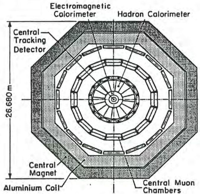
Fig. II.2. Middle section view of L*.
