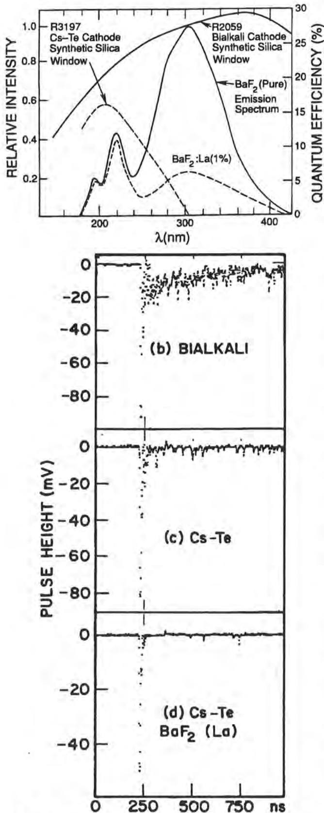
Fig. VI.1. (a) BaF 2 scintillation spectrum. (b,c,d) BaF 2 scintillation pulses observed with a digital scope with (b) bi-alkali photocathode, (c) Cs-Te photocathode, and (d) Cs-Te photocathode and La-doped BaF 2 crystal. The rise time for the fast signal is 3 ns.
