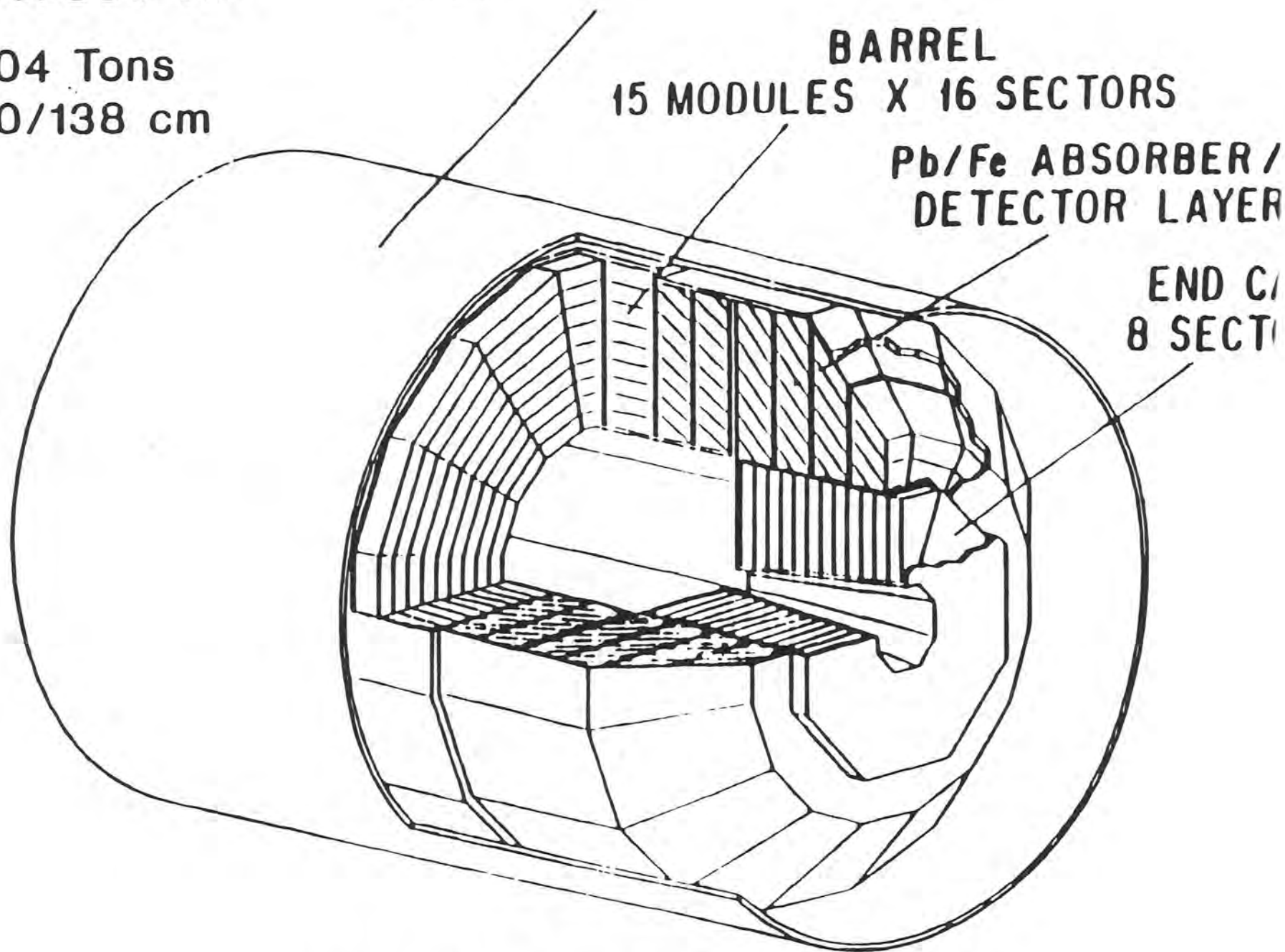
HADRON CALORIMETER
