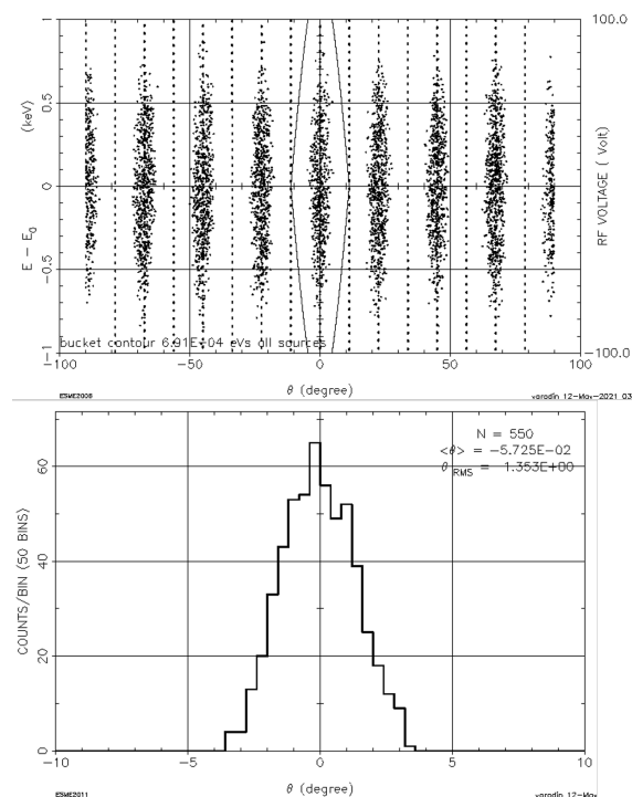
Figure 8: (Top) Longitudinal distribution of 5000 macro particles after the re-bunching process. (Bottom) Phase distribution of particles within selection contour.
