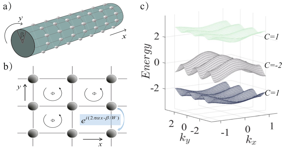
Fig. 1 Nearest-neighbor hopping of atoms in a square lattice with a uniform magnetic field. a Nearest-neighbor hopping on a two-dimensional square lattice with the periodic boundary conditions along the y -direction. b A partial view of the system. c The energy bands of the Harper-Hofstadter model in momentum space, where the Chern numbers of three bands are 1, -2 , 1. The parameters are N = 30 , a_x = a_y = t = 1 , W = 9 , and \beta = 0.2\pi
