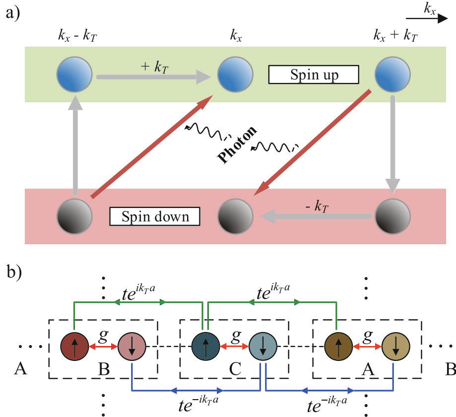
Fig. 2 a Schematic diagram of the coupling between the field (photon) and the system (atoms in the lattice). The blue and gray spheres represent atoms of spin up and spin down, respectively. b Schematic diagram of the coupling of pseudospins defined by \hat{H}_{total} at \alpha = 1/3 . The dashed rectangular box represents the coupling (red lines) between the pseudospins inside the lattice. The solid green and blue lines indicate the couplings of spin up and down between different lattices, respectively
