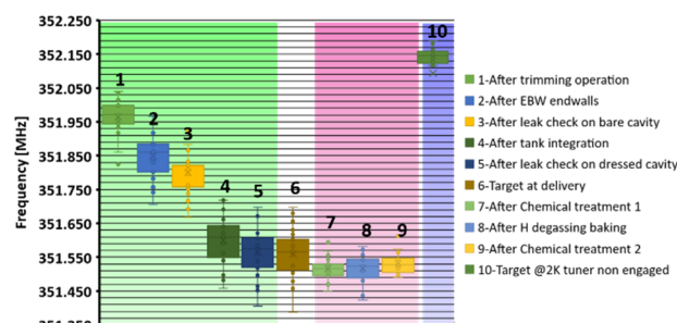
Figure 1: Evolution of the RF frequency during the ESS cavities lifecycle.
