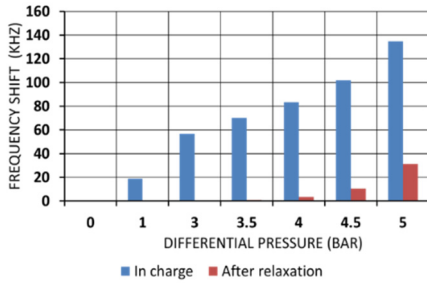
Figure 5: Frequency shifts of a ESS double Spoke cavity computed for the application and removal of differential pressures.
