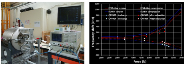
Figure 6: (Left) Experimental setup for the RF tuning by a push/pull action on a MYRRHA Spoke cavity prototype. (Right) Frequency shift measured on the two MYRRHA cavity prototypes with a push/pull action.
