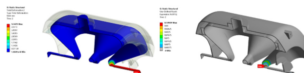
Figure 3: Deformation and plastic strains after applying a tensile force of 7000N on the MYRRHA cavity.
