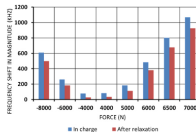
Figure 2: Frequency shifts obtained by the simulation of the push/pull action on the MYRRHA cavity.
