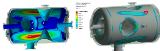
Figure 4: Deformation and plastic strains after applying a differential pressure of 5bars on the ESS cavity.
