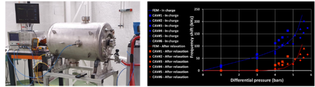
Figure 7: (Left) Experimental setup for the RF tuning of the ESS cavity by pneumatic pressurization. (Right) Frequency shift induced by pneumatic pressurization of the ESS Spoke cavities (Right) Frequency shift induced by pneumatic pressurization of the ESS Spoke cavities.
