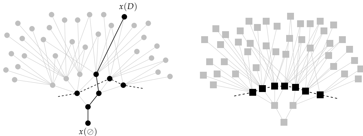
Figure 8. Portion of \mathcal{M}(\mathbb{S}_{PS}) illustrating the permeability problem; corresponding portion of \mathcal{R}(\mathcal{M}(\mathbb{S}_{PS})) showing an impermeable maximal antichain.
