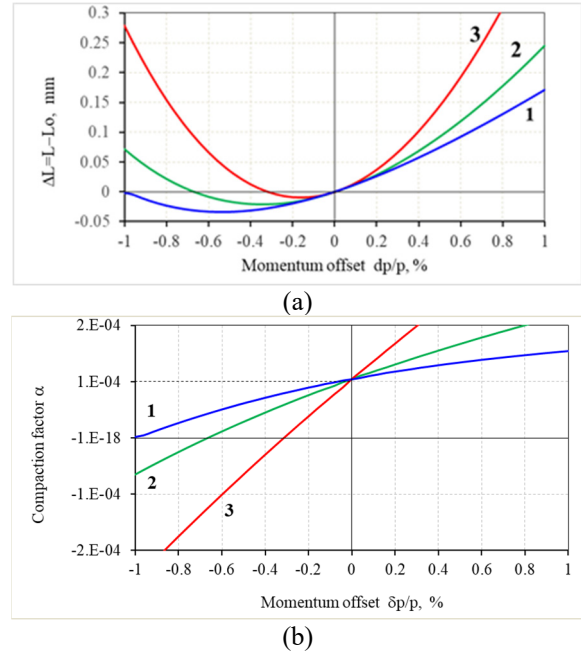
Figure 1: Reduction of the momentum offset of \alpha -buckets with respect to the energy of the reference orbit at low- \alpha mode with \alpha_1 = +1 \cdot 10^{-4} by variation of second term of momentum compaction factor: (a) orbit lengthening as a function of momentum offset; (b) compaction factor vs energy deviation. Curve 1 (blue) corresponds to second term \alpha_2 = +7.13 \cdot 10^{-3} , curve 2 (green) – \alpha_2 = +1.37 \cdot 10^{-2} and curve 3 (red) – \alpha_2 = +3.26 \cdot 10^{-2} .
