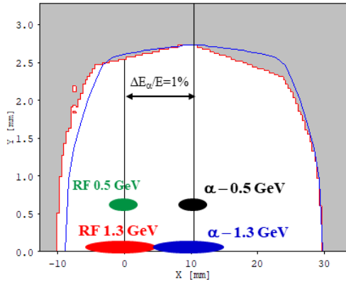
Figure 2: Expected images of RF and \alpha -buckets to be simultaneously stored at KARA during low- \alpha operation where the first term of momentum compaction factor is \alpha_1=+1\cdot10^{-4} . Bunches at 0.5 and 1.3 GeV are split in the vertical plane for clarity. Dispersion D\approx-1 m at observation point. It was assumed that momentum offset between RF and \alpha -buckets is \sim 1\% .
