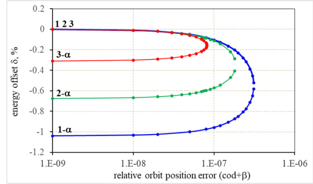
Figure 3: Energy offsets of \alpha -buckets in the presence of momentum independent coherent orbit errors ( \chi ). Positive low- \alpha optics of the KARA storage ring with first term \alpha_1=+1\cdot10^{-4} was chosen as an example. Curves marked in blue represent RF (1) and \alpha -buckets (1- \alpha ) with second term \alpha_2=+7.13\cdot10^{-3} , curves marked in green – RF (2) and \alpha -buckets (2- \alpha ) with \alpha_2=+1.37\cdot10^{-2} and curves marked in red – RF (3) and \alpha -buckets (3- \alpha ) with \alpha_2=+3.26\cdot10^{-2} .
