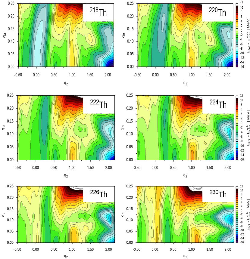
Fig. 1. Potential energy (relative to the spherical LSD energy) landscapes on the (q_2, q_3) plane for 6 even–even isotopes between ^{218}\text{Th} – ^{230}\text{Th} minimised with respect to hexadecapole q_4 and non-axial deformation parameter \eta .
