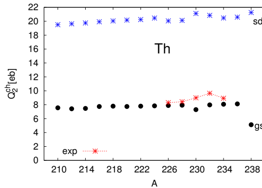
Fig. 2. Electric quadrupole moments Q_2^{\text{ch}} for the ground state (gs) and superdeformed (sd) isomeric minima along the Th isotopic chain. Experimental data for the ground state are shown [9].
