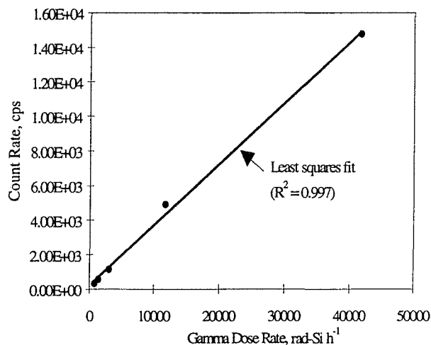
Figure 11. Response of a SiC Schottky detector to gamma-ray intensity. Detector counting rate is proportional to gamma dose rate over the range studied.
