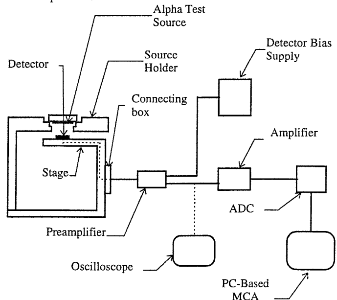
Figure 2. Experimental setup used for SiC detector testing.
