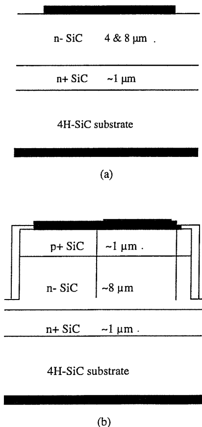
Figure 1. Schematic diagram of (a) Schottky and (b) p-n junction diodes.
