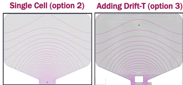
Figure 2: APEX2 cavity design options (2) and (3).
