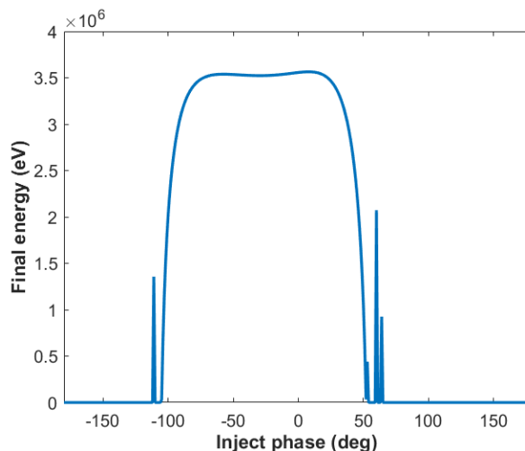
Figure 5: The final energy of electrons injected at different phase of the 8 cells standing-wave accelerator.
