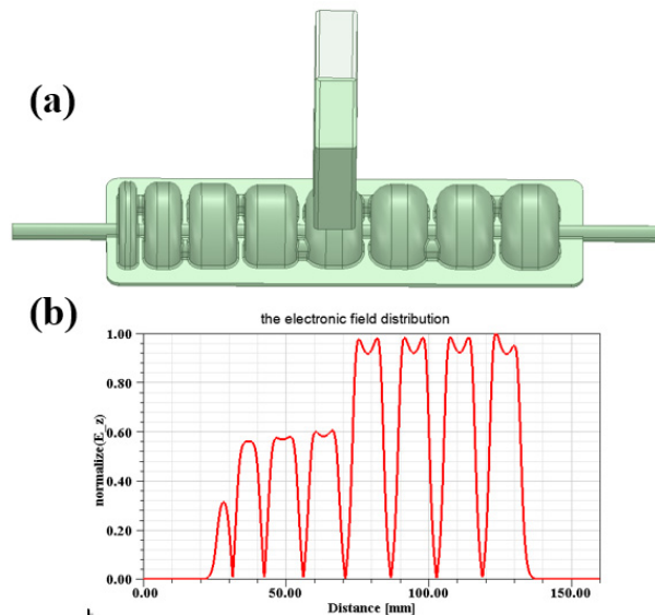
Figure 4: (a) The HFSS model and (b) simulated electronic field distribution of the 8 cells standing-wave accelerator.
