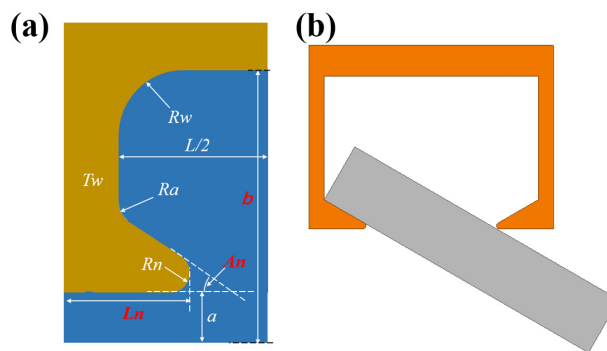
Figure 1: (a) The diagram of single accelerating cell; (b) The tangent relation of the milling cutter (grey) and the copper cell (orange) on the vertical symmetry plane.
