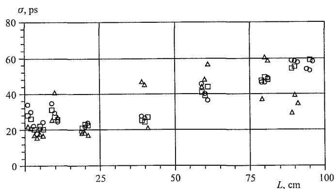
Fig. 5. Spatial resolution along one half of a straw for registering gammas from ^{55}\text{Fe} gamma-ray source. The gas mixture pressure is 1 bar and the gas gain is \sim 7 \cdot 10^4 . T_t and T_b levels are 0.2 and 0.7 (open circles), 0.05 and 0.8 (open triangles), and 0.1 and 0.6 (open squares), respectively
