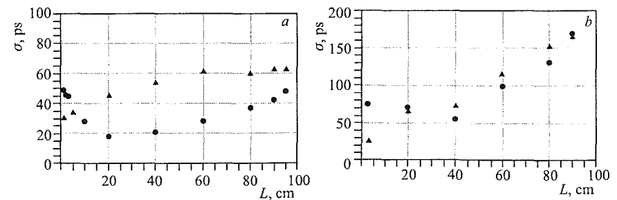
Fig. 4. Accuracy (r.m.s.) of the determination of the longitudinal coordinate along a 2 m long straw for incomplete matching. Filled circles — the gas mixture pressure is 1 bar and gas gain is \sim 7 \cdot 10^4 (anode voltage is 1.95 kV). Filled triangle — the gas pressure is 3 bar and the anode voltage is 3.05 kV. The matching impedance for each straw end is 300 \Omega . a ) ^{55}\text{Fe} source; b ) ^{106}\text{Ru} source
