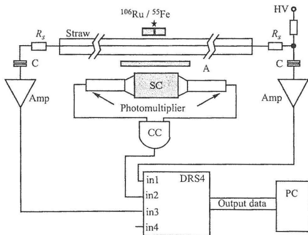
Fig. 1. Schematic layout of the setup. A — absorber, SC — scintillation counter, Amp — amplifier, CC — coincidence circuit, DRS4 — Domino Ring Sampler
