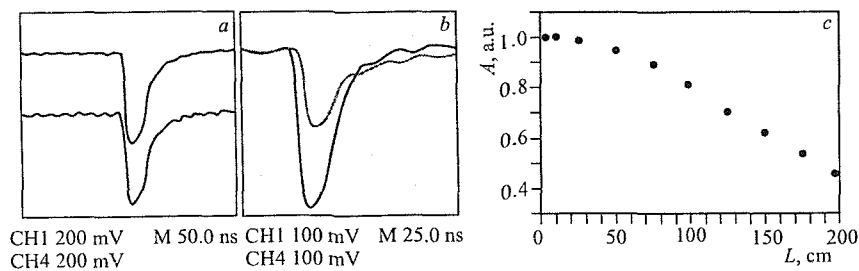
Fig. 2. a ) Signal registered at the ends of the anode when a collimated ^{55}\text{Fe} source is located at the middle of the straw. b ) Typical signals registered by an amplifier when a collimated ^{55}\text{Fe} source is located near the ends of a straw. c ) Signal attenuation as a function of the distance from the straw end. The gas mixture pressure is 1 bar; gas gain is \sim 7 \cdot 10^4
