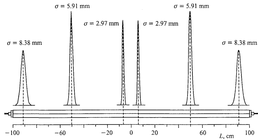
Fig. 7. Results of the measurements of the spatial accuracy as function of the source position with respect to the middle of 2 m long straw indicated as zero. The straws were irradiated by electrons from ^{106}\text{Ru} source, the gas mixture pressure is 1 bar and the gas gain is \sim 7 \cdot 10^4
