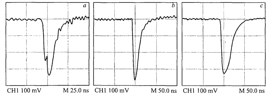
Fig. 3. a ) Typical signals obtained in the absence of a 180 \Omega series resistors R_s ; b ) for an option with R_s = 180 \Omega ; c ) for an option with R_s = 240 \Omega . The gas mixture pressure is 1 bar; gas gain is \sim 7 \cdot 10^4
