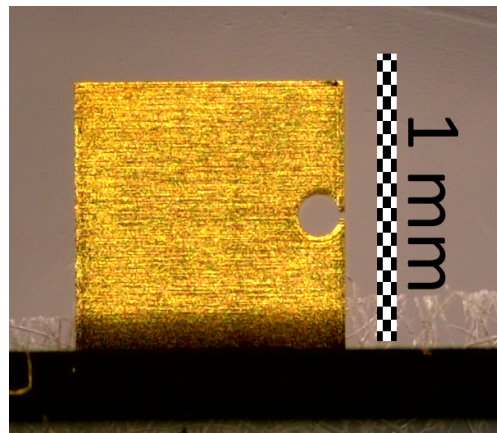
Figure 1: Image of the split-ring resonator device. The streaking EM field is located in the split of the ring with a size of 20\text{ }\mu\text{m} by 20\text{ }\mu\text{m} .
