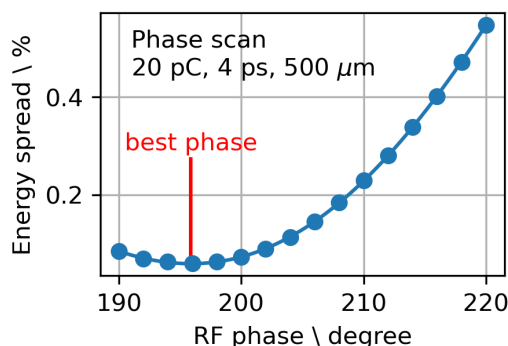
Figure 3: Automated phase scan for an example bunch. After tracking from the cathode half a metre, the particle distributions are evaluated for their absolute energy spread. The plot shows the data results, a fit with a fourth polynomial and the result of the best phase for a minimum in energy spread.
