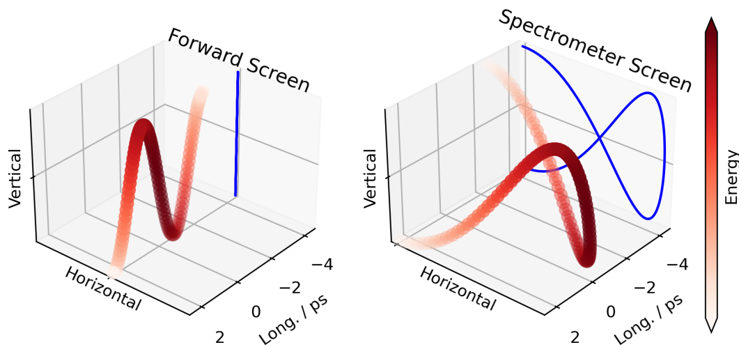
Figure 2: Sketched screen image. Electron bunch with symmetric energy distribution. Projection visible on beam screen in blue. a) Forward screen without dispersion, overlapping screen image prevents diagnosis of the full bunch length. b) Dispersive screen after spectrometer shows bunch vertical sorting by energy resulting in loop shaped image and unravels the whole bunch length on the screen.
