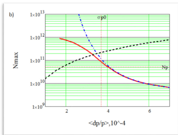
Figure 2: Dependence of the number of stored ions on the momentum spread at the ion energy of 3 GeV/n. Read line: with ion space charge effects, blue line: without ion space charge effects.
