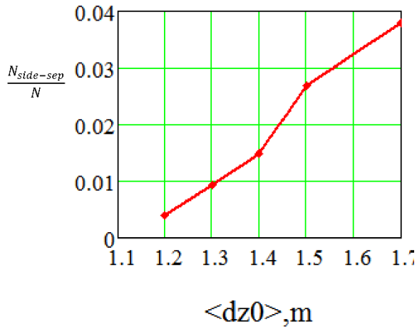
Figure 6: Dependence of the ratio of the number of captured ions in the side parasitic separatrix to the total number of bunch ions on the rms bunch length after the RF2 bunching.
