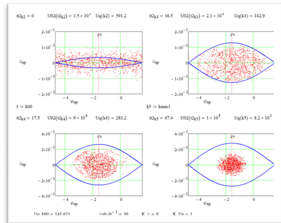
Figure 3: Bunching of the ion beam by the RF2 system at the ^{197}\text{Au}^{79+} ion energy of 3 GeV/n (initial RF2 voltage 1.5 kV, final voltage 100 kV, RF2 frequency variation 10 half bends/s, and cooling time 100 s).
