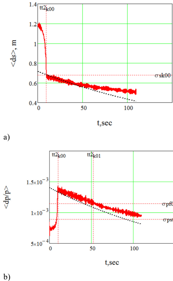
Figure 7: Dependence of the rms bunch length (a) and the momentum spread (b) on the time at the ion energy of 3 GeV/n (cooling time 100 s and bunch length of 1.2 m after RF2 bunching).
