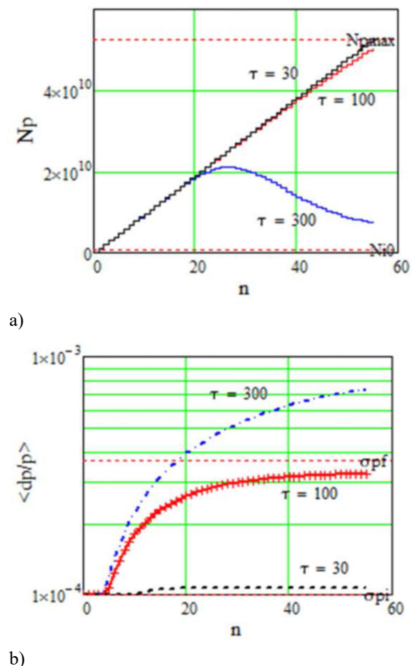
Figure 1: Dependence of the number of stored ions (a) and the momentum spread (b) on the number of injection cycles at different cooling times.
