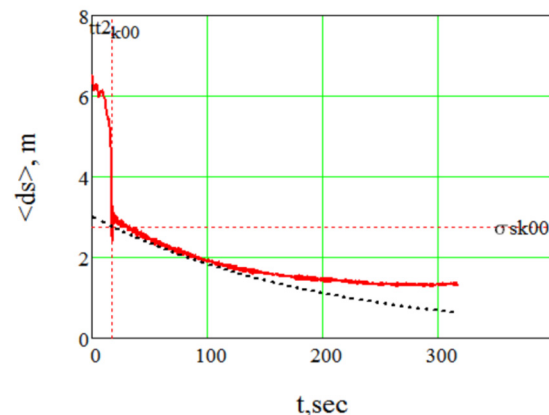
Figure 4: Dependence of the rms bunch length on time at the ion energy of 3 GeV/n (cooling time 100 s).
