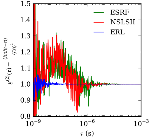
Figure 5. Intensity correlations as a function of delay time \tau for different sources. For studies of dynamics at timescales less than 1 \mu\text{s} , the time structure of existing sources (used to mitigate ion trapping) becomes a significant contribution to noise. The ERL is expected to be quasi-continuous down to the 10 ns level.
