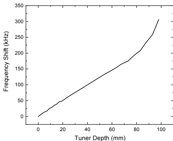
Figure 7: Tuning Range of the movable tuners.
