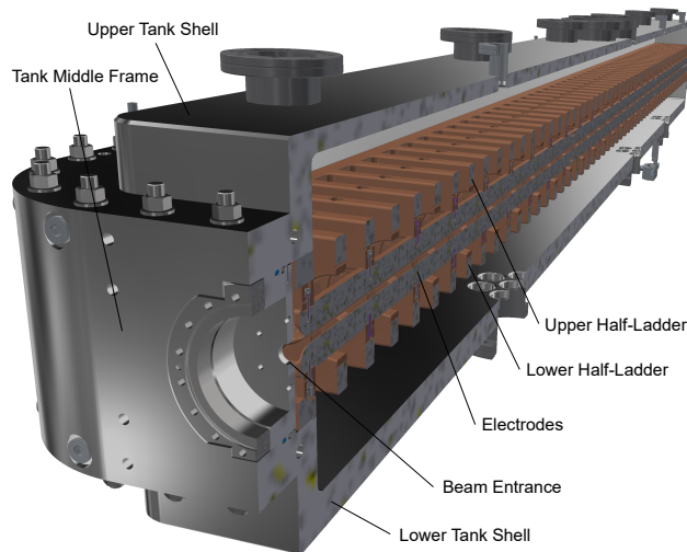
Figure 1: Isometric view of the 3.3 m modulated Ladder-RFQ. Solid copper carrier-rings guarantee the electrode positioning as well as the RF contact. The ladder structure consists of bulk copper components. Any brazing or welding processes were avoided for the assembly of the main components.
