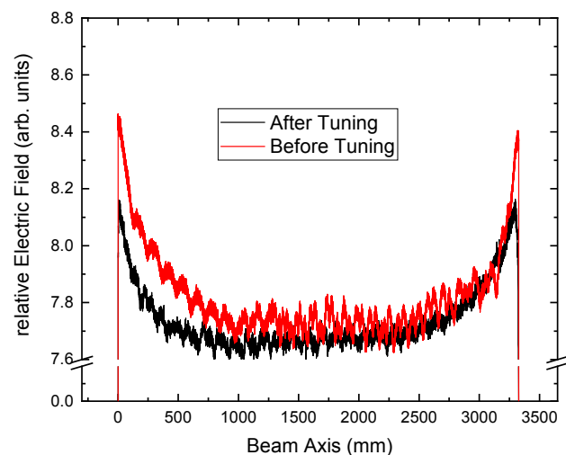
Figure 5: Detailed comparison of the flatness before and after tuning.
