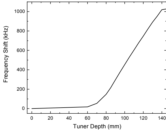
Figure 6: Tuning Range of the static tuners.
