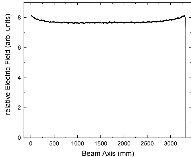
Figure 4: Flatness after tuning. The relative on-axis flatness is 1%.
