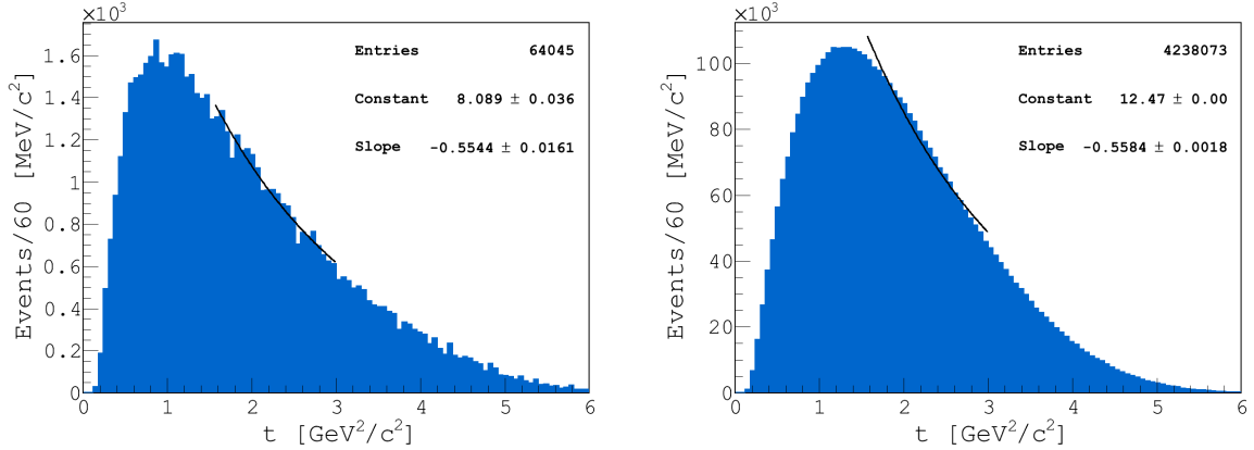
(a) The momentum transfer |t| distribution of the data. (b) The momentum transfer |t| distribution of the accepted MC.
