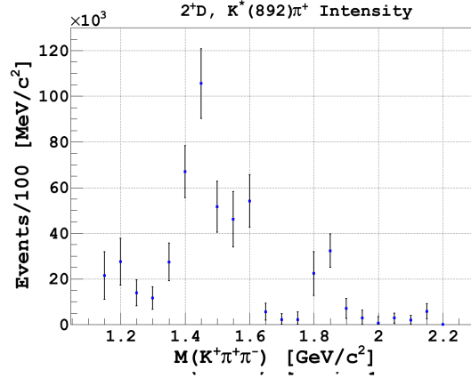
(b) The 2^+D, K^*(892)\pi^+ wave intensity.
