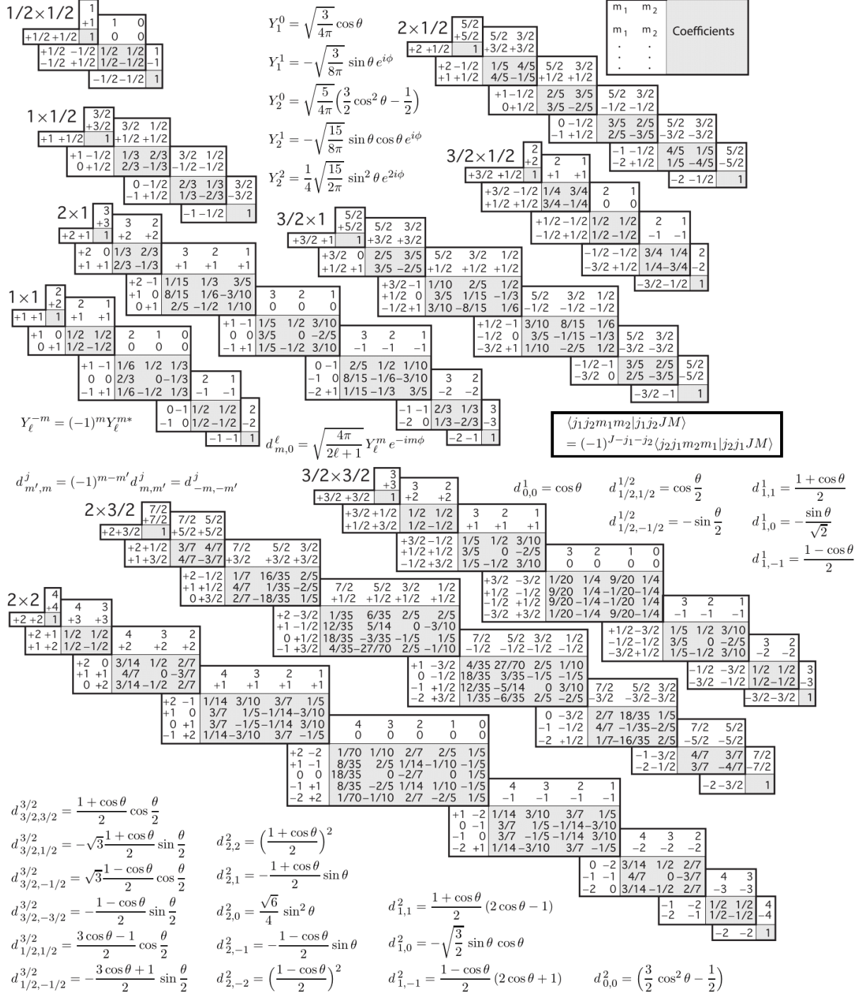
Figure F.1: The Clebsch-Gordan coefficients table with the Wigner-d functions and the spherical harmonics Y_l^m . Image source [16].
