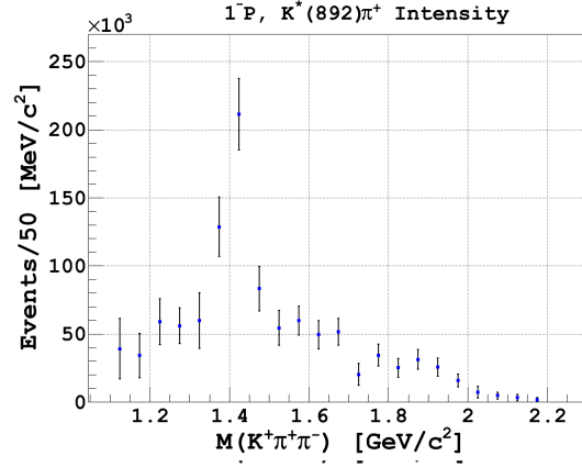
(b) The 1^-P, K^*(892)\pi^+ wave intensity.
