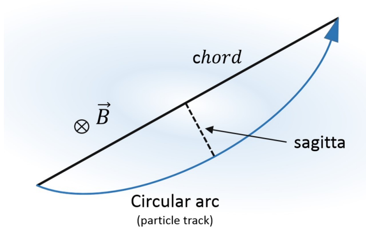
Figure 2.16: The path of a charged particle going through a magnetic field. When the radius of curvature is large when compared with the sagitta, the radius of curvature can be approximated by r \approx \frac{l^2}{2s} .
