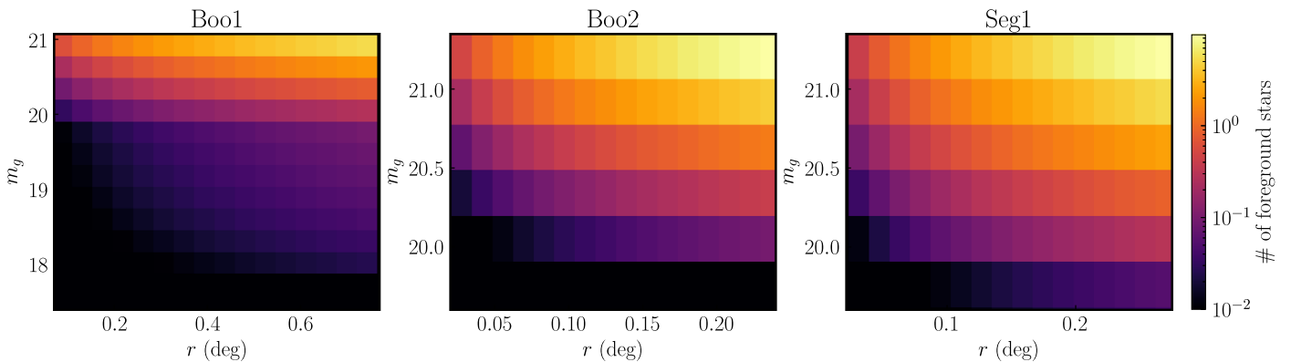
Figure 10. A 2D histogram displaying the estimated number of MW foreground stars for Boo1, Boo2, and Seg1 as a function of radius (in degrees) and m_g . The number of MW foreground stars increases as the magnitude becomes fainter and the radius grows larger.
