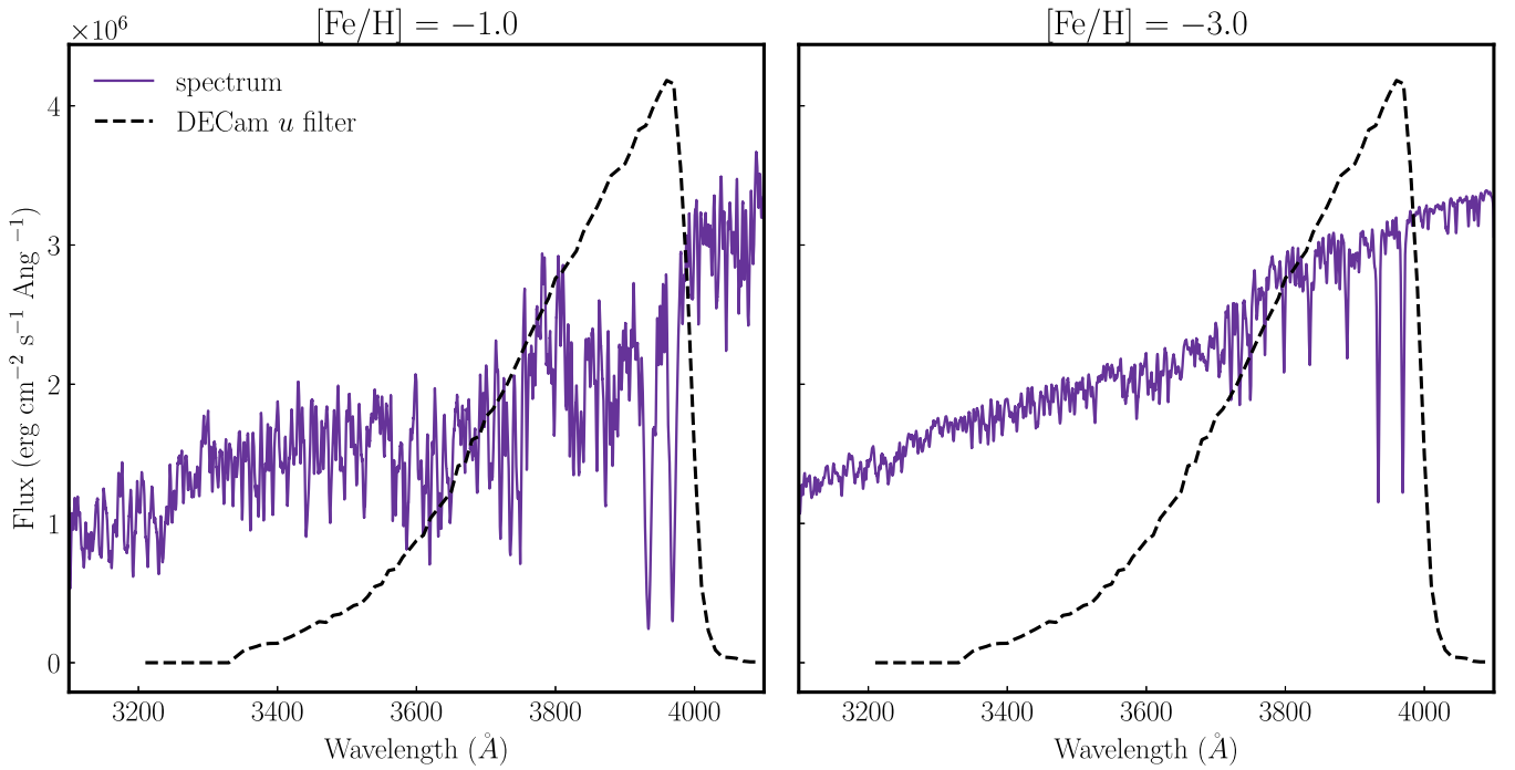
Figure 3. An illustration of why the DEC a m u -band is sensitive to metallicity. Left: a synthetic spectrum generated by Turbospectrum (R. Alvarez & B. Plez 1998; B. Plez 2012) for a sample cool red giant star with metallicity [\text{Fe}/\text{H}] = -1 overlaid with the bandpass of the DEC a m u filter. Right: the synthetic spectrum for a sample star with the same surface gravity and surface temperature but with metallicity [\text{Fe}/\text{H}] = -3 . The Ca II K metal absorption lines are more prominent for more metal-rich stars (left), and the DEC a m u -band filter completely covers this feature. Therefore, the more metal-rich a star is, the dimmer it appears in the DEC a m u band. This correlation provides a way to associate the DEC a m u -band magnitude of a star with its metallicity, as shown in Figure 4.
