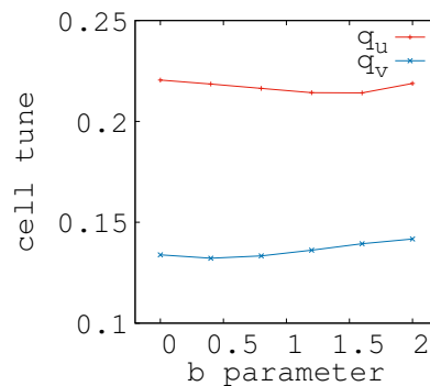
Figure 6: Cell tune shift as a function of relative excitation b parameter of the horizontal orbit control scheme in the double coil design. Figure published in [6].
