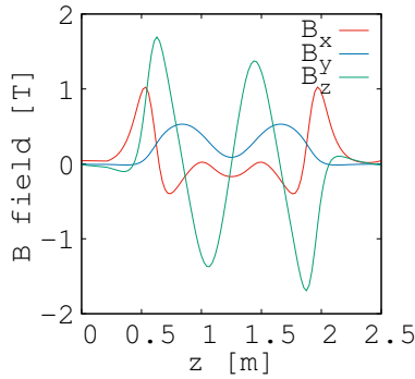
Figure 2: The magnetic fields along the orbit in a cell for 12 MeV beam energy in the FDF lattice. Figure published in [6].
