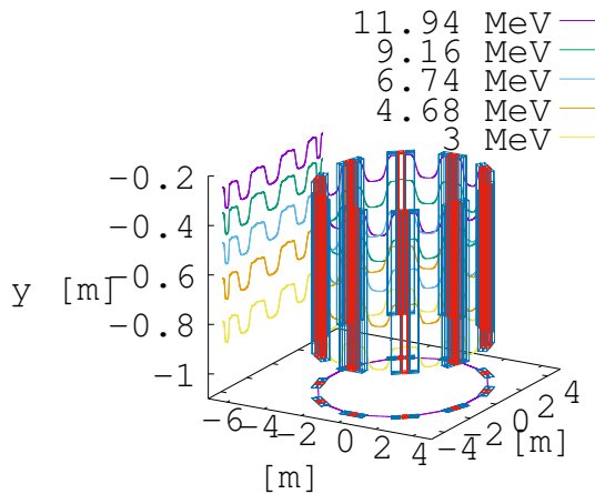
Figure 3: Closed orbits for different momenta in the FDF triplet lattice. The locations of the Bd and Bf magnets are indicated by red and blue boxes respectively. Figure published in [6].
