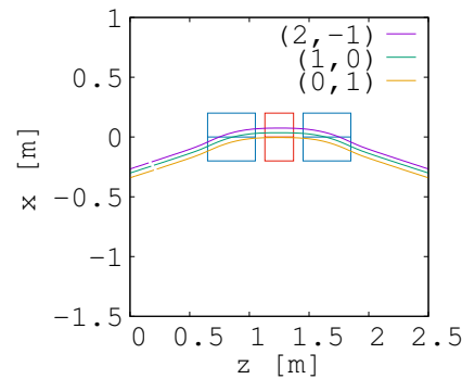
Figure 5: Orbit shift controlled by a double coil design in the FDF triplet lattice. A bracket (b, 1 - b) indicates the relative excitation of outer coil b to inner coil 1 - b . The total excitation is kept at unity. Figure published in [6].
