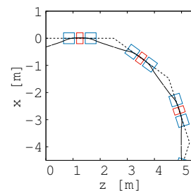
Figure 1: Closed orbits for FDF lattice. The dashed line indicates the polygon with 10 sides. Figure published in [6].
