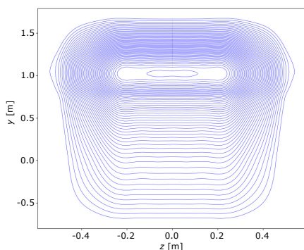
Figure 7: Representation of the coil configuration for the first prototype. The good field region is between y = 0 m and y = 0.6 m.
