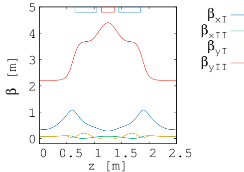
Figure 4: Beta functions \beta_{xI} , \beta_{xII} , \beta_{yI} , \beta_{yII} according to the procedure by Willeke-Ripken [7]. The magnet positioning is shown at the top, the red box corresponding to the Bd magnet and the blue box to the Bf magnet. Figure published in [6].
