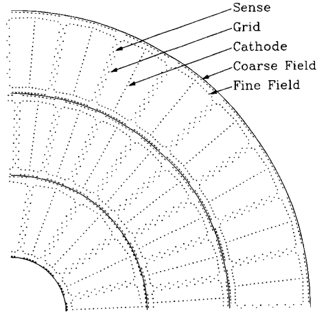
Figure 2.4: End view of one quadrant of the VTX chamber.
