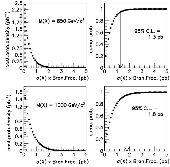
Figure 7.15: The posterior probability density and the cumulative probability vs. \sigma_X B for M_X = 850 and 1000 \text{ GeV}/c^2 . The arrow shows the 95% confidence level upper limit on \sigma_X B .
