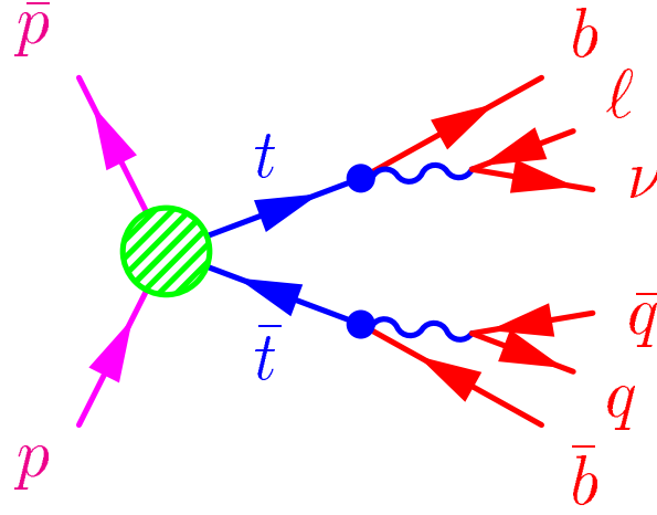
Figure 4.1: A t\bar{t} \rightarrow l + \text{jets} decay.
