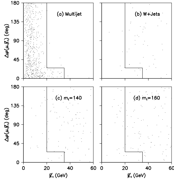
Figure 4.4: Distribution of \Delta\phi(\cancel{E}_T, \mu) vs. \cancel{E}_T for e + \text{jets}/\mu events for (a) multijet background sample; (b) W + \text{jets} sample (VECBOS Monte Carlo); (c) Standard Model (SM) t\bar{t} Monte Carlo (ISAJET, m_t = 140 \text{ GeV}/c^2 ); (d) SM t\bar{t} Monte Carlo (ISAJET, m_t = 160 \text{ GeV}/c^2 ). The contour shows the cut values.
