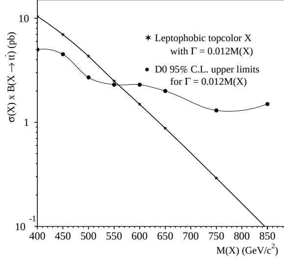
Figure 2: The DØ Run I 95% confidence level upper limits on \sigma_X B as a function of resonance mass M_X . Included for reference are the predicted topcolor assisted technicolor cross sections for a width \Gamma_X = 1.2\% M_X .
