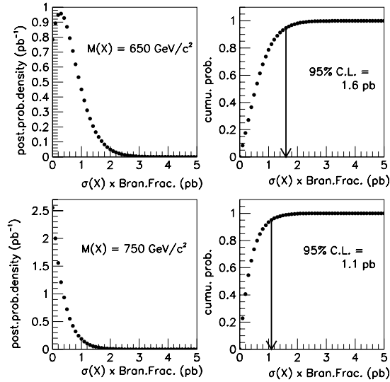
Figure 7.14: The posterior probability density and the cumulative probability vs. \sigma_X B for M_X = 650 and 750 \text{ GeV}/c^2 . The arrow shows the 95% confidence level upper limit on \sigma_X B .
