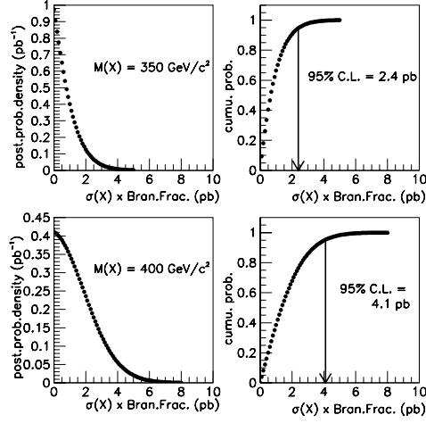
Figure 7.11: The posterior probability density and the cumulative probability vs. \sigma_X B for M_X = 350 and 400 \text{ GeV}/c^2 . The arrow shows the 95% confidence level upper limit on \sigma_X B .
