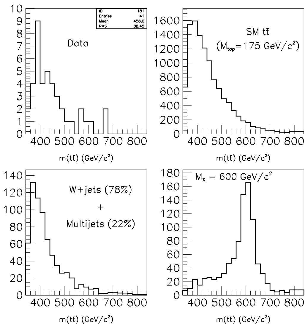
Figure 6.1: Distributions of m_{t\bar{t}} for DØ Run I lepton plus jets data, Standard Model t\bar{t} production, W + jets and multijets combined in the ratio 0.78:0.22, and signal ( X \rightarrow t\bar{t} ) for M_X = 600 \text{ GeV}/c^2 . The histograms are not normalized.
