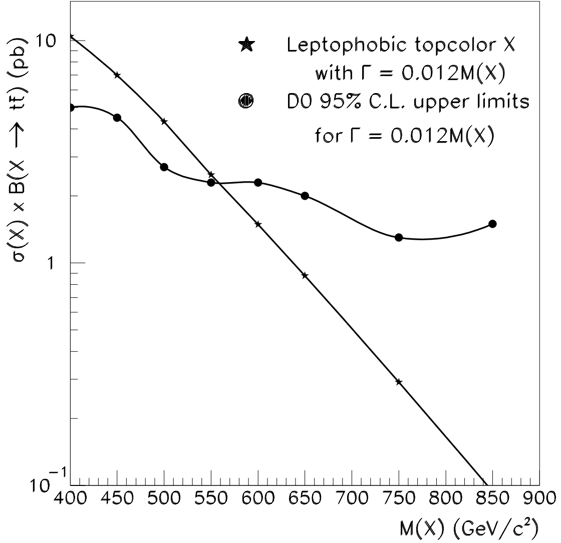
Figure 8.1: The DØ Run I 95% confidence level upper limits on \sigma_X B as a function of resonance mass M_X . W +jets and multijets are combined in the ratio 0.78:0.22. The error on \sum_i A_i \mathcal{L}_i is included as a Gaussian in the expression for the posterior probability density for \sigma_X B . Included for reference are the predicted topcolor assisted technicolor cross sections for a width, \Gamma_X = 1.2\% M_X .
