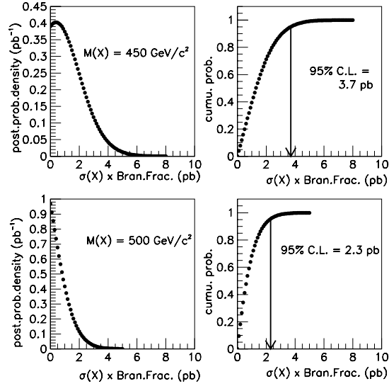
Figure 7.12: The posterior probability density and the cumulative probability vs. \sigma_X B for M_X = 450 and 500 \text{ GeV}/c^2 . The arrow shows the 95% confidence level upper limit on \sigma_X B .
