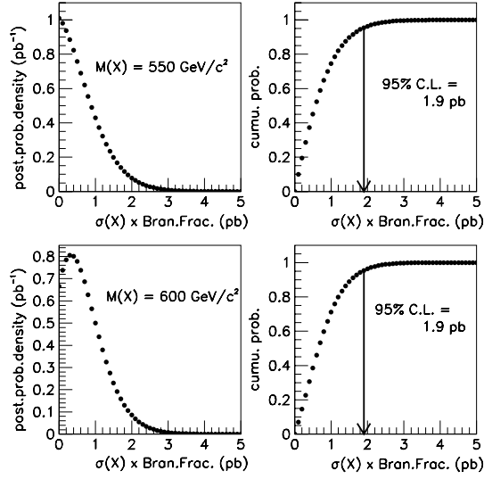
Figure 7.13: The posterior probability density and the cumulative probability vs. \sigma_X B for M_X = 550 and 600 \text{ GeV}/c^2 . The arrow shows the 95% confidence level upper limit on \sigma_X B .
