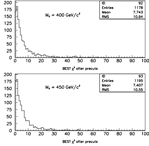
Figure 5.4: \chi^2 distribution for X \rightarrow t\bar{t} at M_X = 400 \text{ GeV}/c^2 and 450 \text{ GeV}/c^2 . Pre-selections are applied and the contents in all four channels ( ej , ej/\mu , \mu j , \mu j/\mu ) are added.
