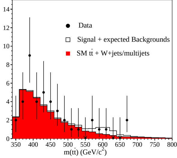
Figure 1: Normalized distributions of m_{t\bar{t}} for sum of all Standard Model backgrounds (shaded) and sum of signal ( X \rightarrow t\bar{t} ) and Standard Model backgrounds (unshaded) for M_X = 600 \text{ GeV}/c^2 . The data m_{t\bar{t}} distribution is shown by dots.
