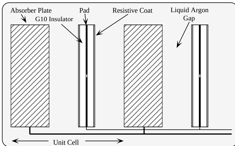
Figure 2.9: Schematic view of a calorimeter cell.
