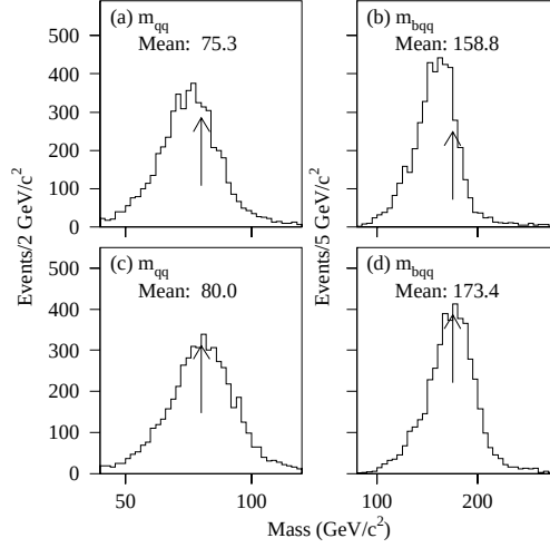
Figure 3.6: Masses of W \rightarrow q\bar{q} and t \rightarrow b\bar{q}\bar{q} in standard t\bar{t} Monte Carlo with m_t = 175 \text{ GeV}/c^2 , both (a), (b) with standard corrections only and (c), (d) with all jet corrections. The arrows locate the input W boson and top quark masses.
