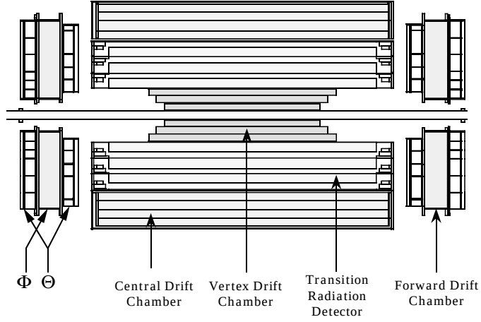
Figure 2.3: Side view of the DØ central detector.
