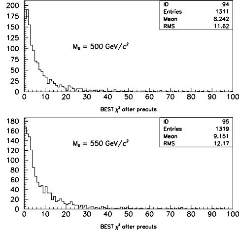
Figure 5.5: \chi^2 distribution for X \rightarrow t\bar{t} at M_X = 500 \text{ GeV}/c^2 and 550 \text{ GeV}/c^2 . Pre-selections are applied and the contents in all four channels ( ej , ej/\mu , \mu j , \mu j/\mu ) are added.
