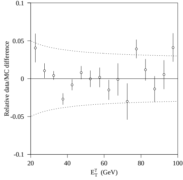
Figure 3.4: The relative energy scale difference between data and Monte Carlo as a function of photon E_T after all jet corrections are applied. The curves indicate an error band of \pm(2.5\% + 0.5 \text{ GeV}) of the jet energy.
