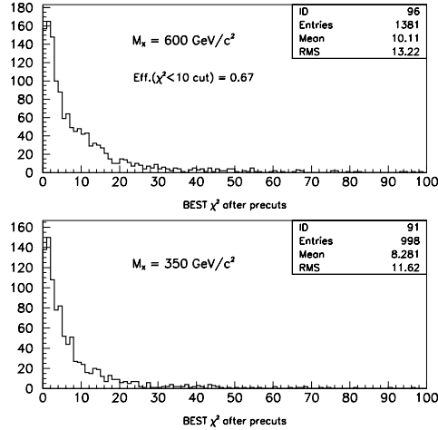
Figure 5.3: \chi^2 distribution for X \rightarrow t\bar{t} at M_X = 600 \text{ GeV}/c^2 and 350 \text{ GeV}/c^2 . Preselections are applied and the contents in all four channels ( ej , ej/\mu , \mu j , \mu j/\mu ) are added.
