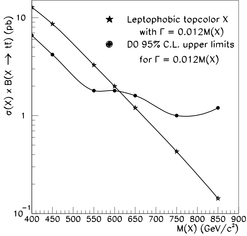
Figure E.4: The DØ Run I 95% confidence level upper limits on \sigma_X B as a function of resonance mass M_X . While maximizing the likelihood, no constraint is applied on the parameters \alpha and \beta in MINUIT. Included for reference are the predicted topcolor assisted technicolor cross sections for a width, \Gamma_X = 1.2\% M_X .
