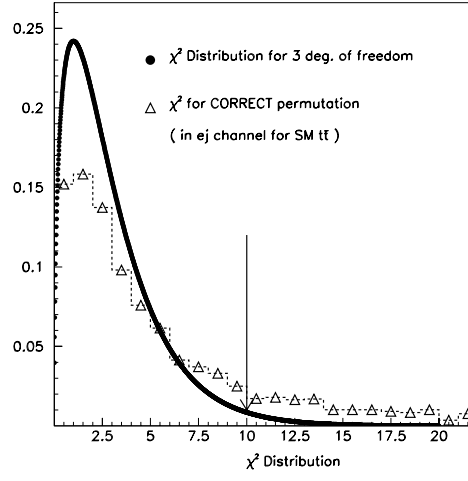
Figure 5.1: \chi^2 distribution for 3 degrees of freedom and the \chi^2 distribution (normalized to unity after preselections) for the correct jet-parton permutation in the e + jets channel for Standard Model t\bar{t} production. It can be seen that there are very few events beyond \chi^2 = 10 indicated by the arrow.
