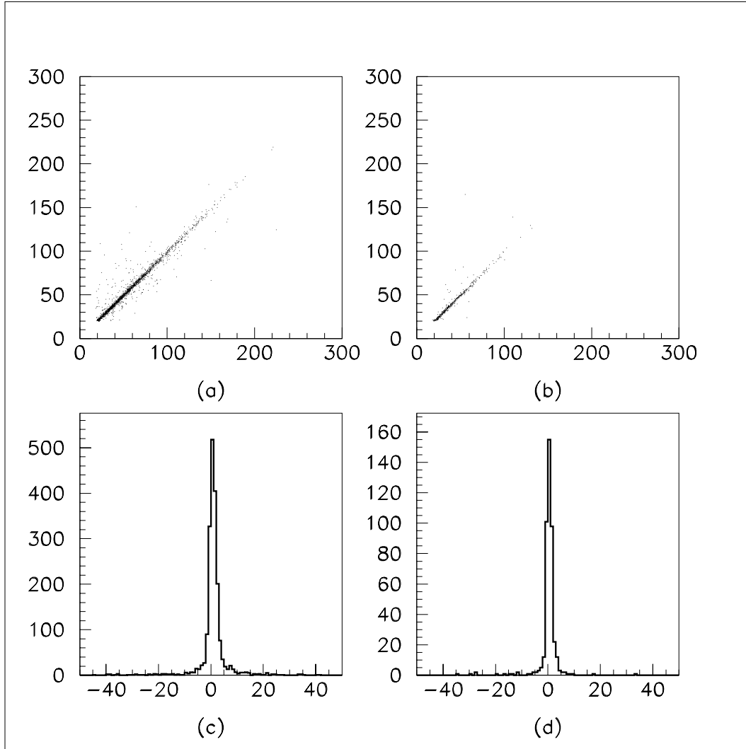
Figure C.2: Plots (a) and (b) show the p_T of the matched reconstructed electron versus the p_T of the leading electron at generator-level, in the CC and EC respectively, for a sample of Standard Model t\bar{t} production generated using Pythia. Plots (c) and (d) show the histograms for the difference between the p_T of the matched reconstructed electron and that of the leading electron at generator-level, in the CC and EC respectively.
