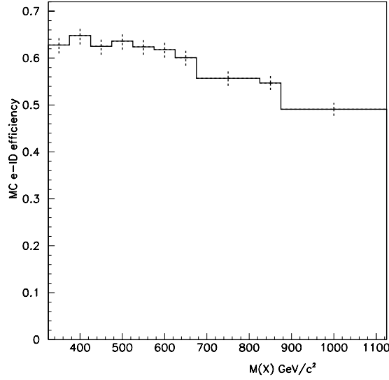
Figure C.3: The Monte Carlo electron identification efficiency in the CC versus M_X . The errors shown are statistical.
