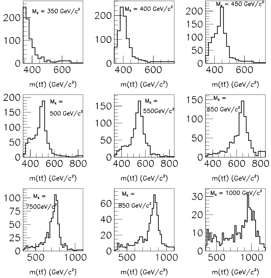
Figure 6.2: Distributions of m_{t\bar{t}} for signal ( X \rightarrow t\bar{t} ) for M_X = 350\text{-}1000 \text{ GeV}/c^2 . The histograms are not normalized. The bin size is different for different M_X , and also non-uniform in m_{t\bar{t}} .
