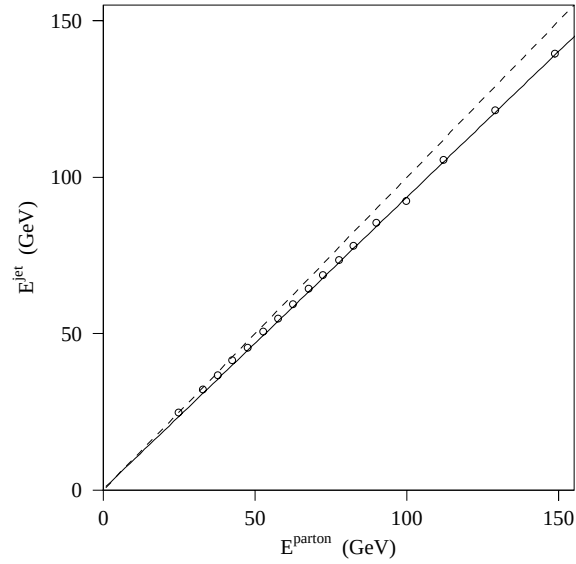
Figure 3.2: The measured jet energies for quarks from W \rightarrow q\bar{q} in t\bar{t} Monte Carlo events are plotted against the corresponding parton energies. Radiation outside the jet cone causes the measured jet energy to be lower than the energy at the parton level. The dashed line is drawn along the diagonal, and the solid line is a linear fit to the points. This plot is based on HERWIG fragmentation with |\eta_{det}^{\text{jet}}| < 0.2 .
