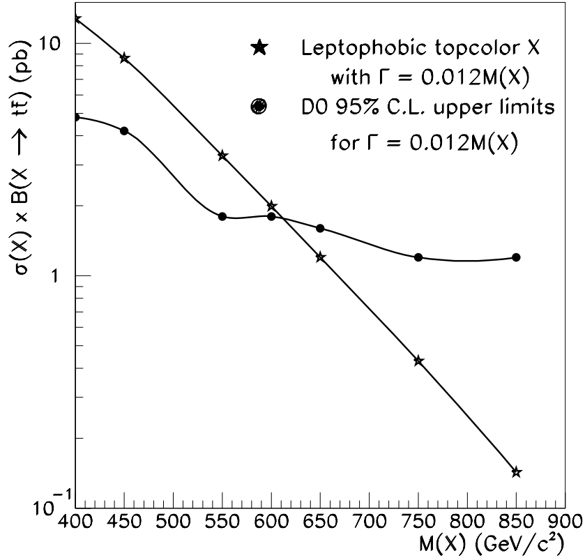
Figure E.2: The DØ Run I 95% confidence level upper limits on \sigma_X B as a function of resonance mass M_X . While maximizing the likelihood, the parameters \alpha and \beta are constrained to be > 0 in MINUIT. Included for reference are the predicted topcolor assisted technicolor cross sections for a width, \Gamma_X = 1.2\% M_X .
