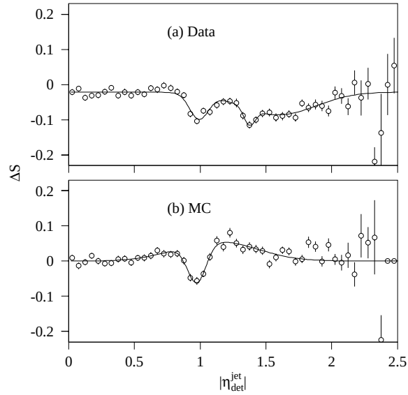
Figure 3.3: The energy scale deviation \Delta S as a function of \eta_{det}^j for (a) data and (b) Monte Carlo (MC). The curves are empirical multi-Gaussian fits to the points.
