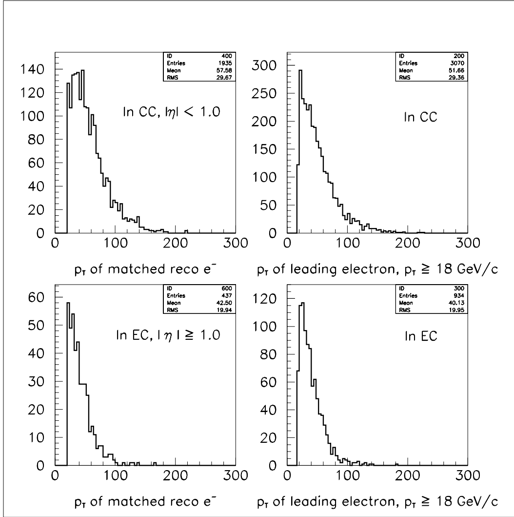
Figure C.1: The transverse momentum, p_T , of the matched reconstructed electron and the leading electron at generator-level with p_T > 18 GeV/c, in the CC and the EC , for a sample of Standard Model t\bar{t} production generated using Pythia.
