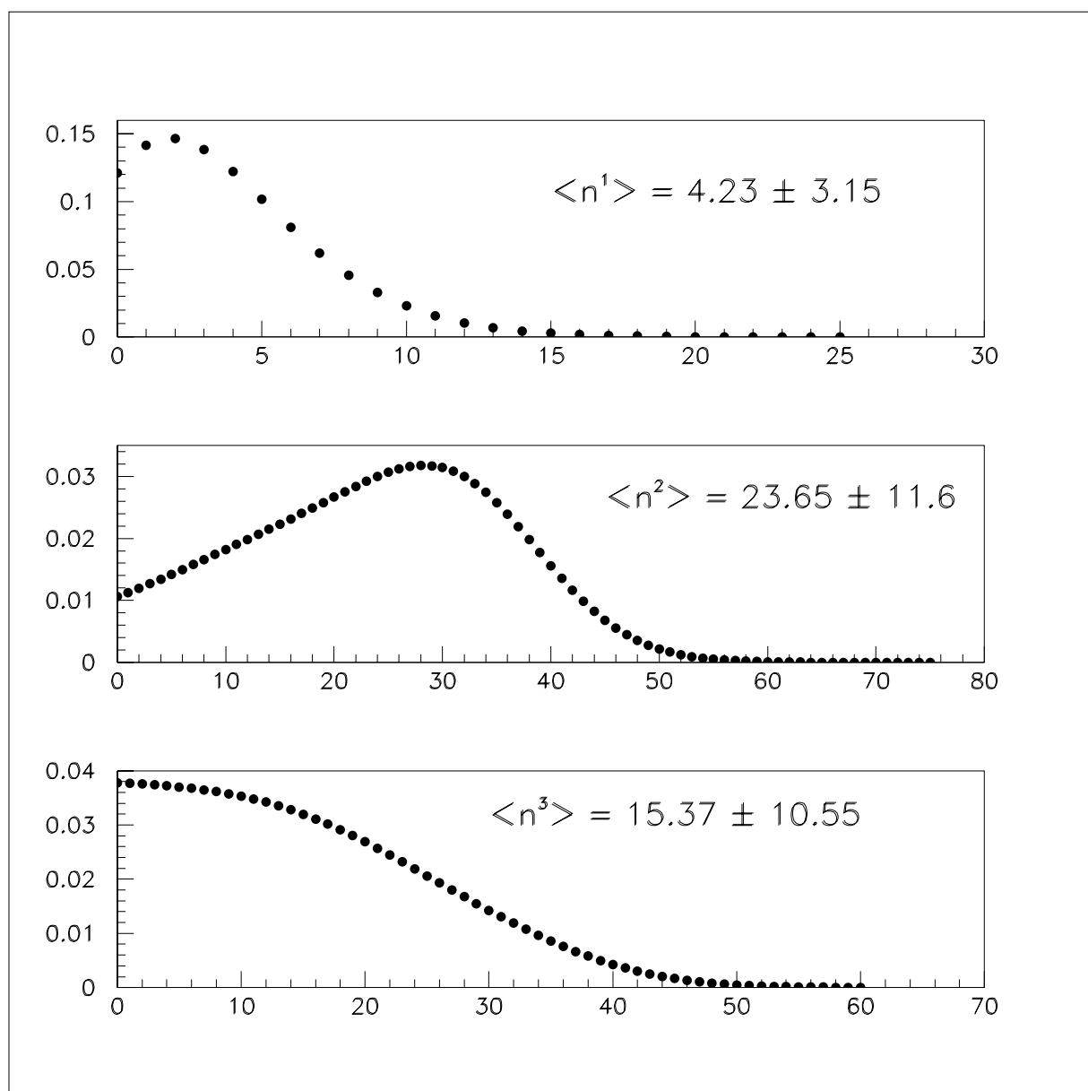
Figure 7.1: P(n_1|D, M_X) , P(n_2|D, M_X) and P(n_3|D, M_X) versus n_1 , n_2 and n_3 respectively for M_X = 600 \text{ GeV}/c^2 .
