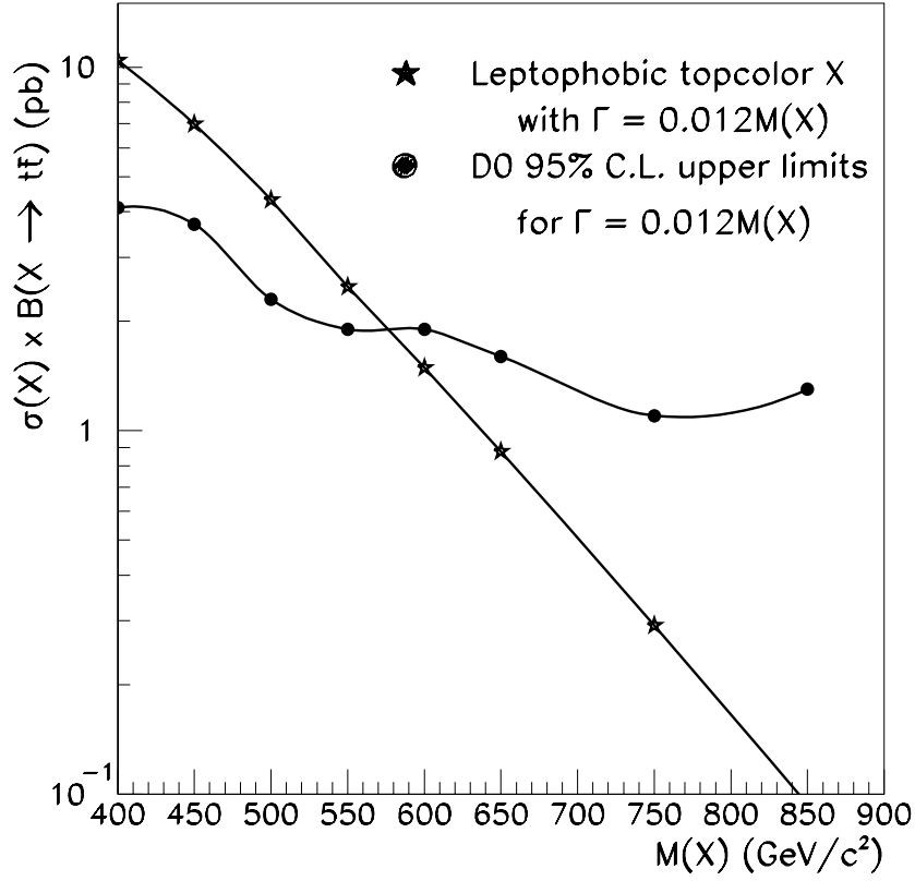
Figure 7.16: The DØ Run I 95% confidence level upper limits on \sigma_X B as a function of resonance mass M_X . W +jets and multijets are combined in the ratio 0.78:0.22. Included for reference are the predicted topcolor assisted technicolor cross sections for a width, \Gamma_X = 1.2\% M_X .
