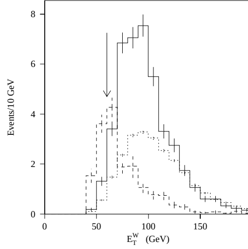
Figure 4.2: E_T^W distribution for Monte Carlo W +jets events (solid histogram), QCD multijet background data (dashed histogram), and t\bar{t} signal with m_t = 175 \text{ GeV}/c^2 (dotted histogram) [33]. All preselections are applied except for the E_T^W cut. The arrow shows the cut value.
