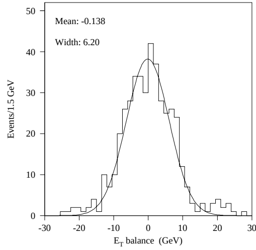
Figure 3.5: Transverse energy balance for (Z \rightarrow ee) + \text{jets} events. All jet corrections are applied. The curve is a Gaussian fit to the histogram.
