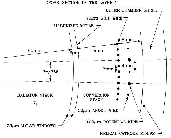
Figure 2.5: A cross section of a TRD layer.
