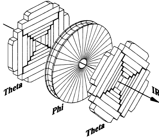
Figure 2.7: Exploded view of one of the FDCs.
