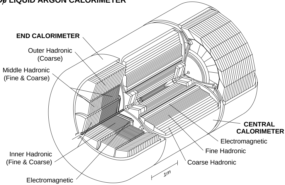
Figure 2.8: The DØ calorimeter.
