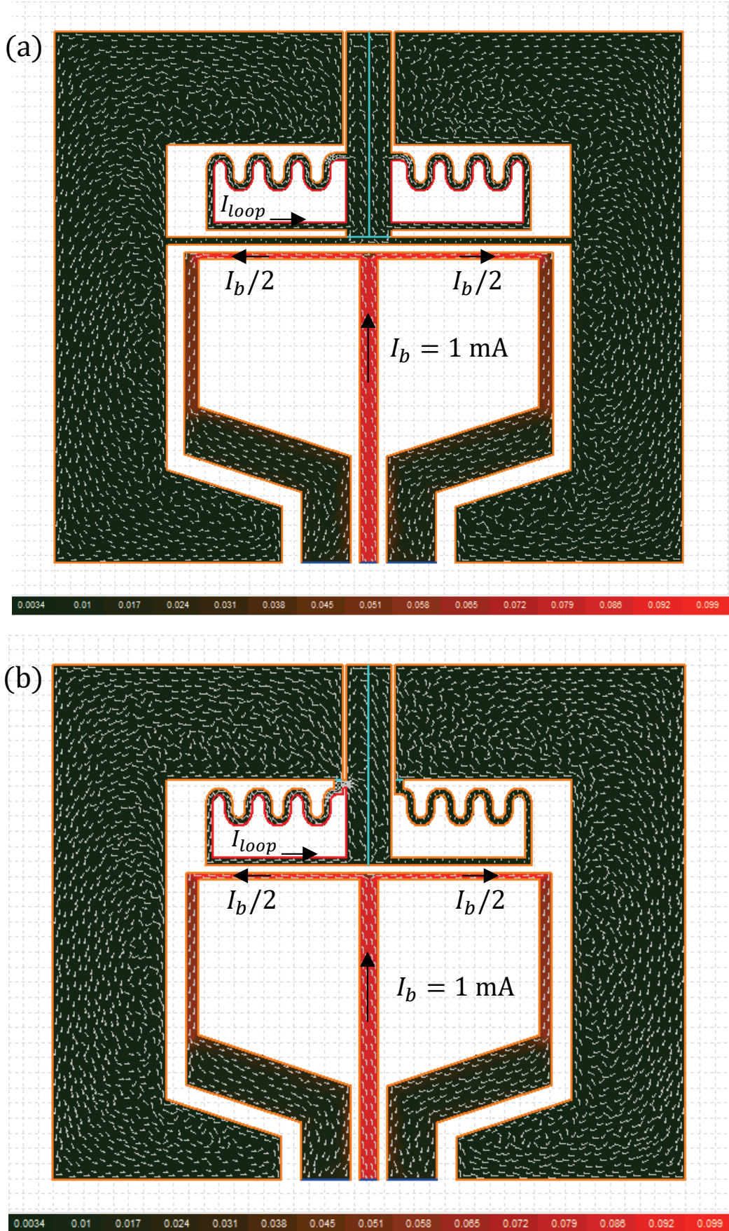
Figure J.3: Current distribution in the gradiometric (a) and standard (b) designs when a DC current bias of I_b = 1 \text{ mA} is applied to the flux line (the differences between the two designs are more visible in Figure J.5, note that in (b) the right loop is not closed). Data was simulated using the 3D-MLSI software for inductance extraction. The direction of the current flow is shown with white arrows and the magnitude of the current density is encoded in colorscale in mA/μm.
