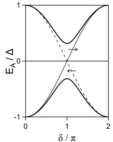
Figure 2.4: Energy spectrum E_A(\delta) of Andreev states in a short Josephson weak link as a function of the superconducting phase difference \delta in the single-particle picture. Thin lines correspond to a junction transparency \tau = 1 (full line is for right-moving electrons, dashed line for left-moving electrons). Thick lines describe the case \tau = 0.9 .
