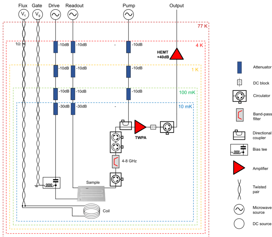
The wiring of the BlueFors fridge was very similar, see Figure 13.5, except for minor changes like the position of the attenuators. The main difference concerns the DC gate bias, which is done through a twisted pair fabricated on long flexible PCBs by our colleague Çağlar Girit at Collège de France, and includes a low-pass RC filter at base temperature. The coil on the sample holder (see Figure 13.3) was wired from a 100\text{ }\mu\text{m} -diameter NbTiN wire, 800 turns on 10 layers. To avoid short-circuits to ground, the metallic mandrel (gold plated copper) was covered with blue-tape on the sides and Kapton tape at the bottom.
