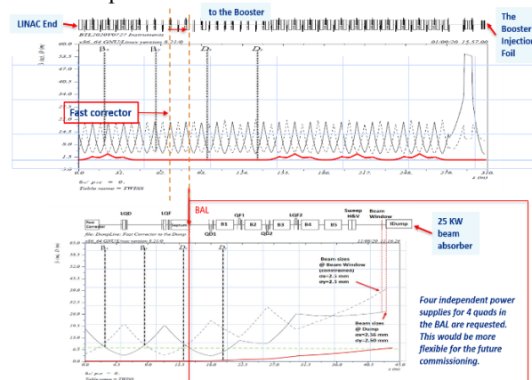
Figure 4: Lattice functions of the BTL and BAL
