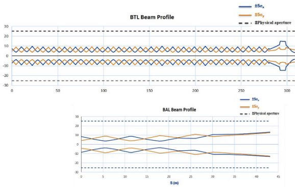
Figure 5: Beam profiles of the BTL and BAL Based on this final lattice design, survey files for CAD 3D model are generated, the layout is shown in Fig.6
