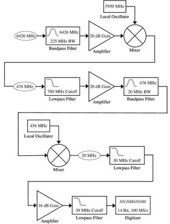
Fig. 10. The electronics used to process the signals from each channel.
