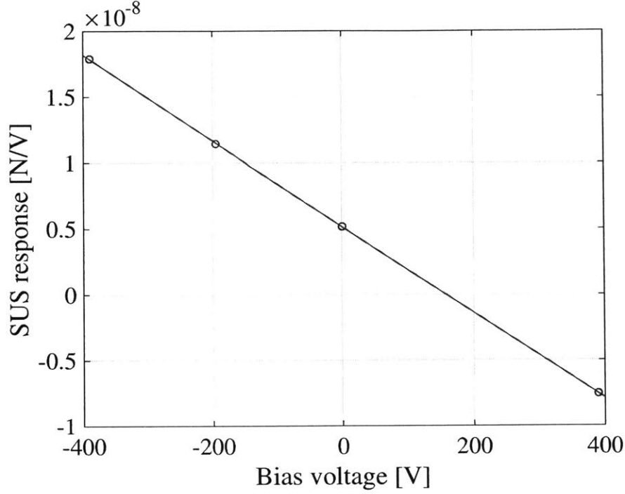
Figure 4-13: Actuation strength of ETMX ring heater with all quadrants driven together vs. bias voltage. Note that the strength of this coupling is about an order of magnitude smaller than from the ESDs, though the voltage noise on the RH drivers is higher than on the ESDs.
