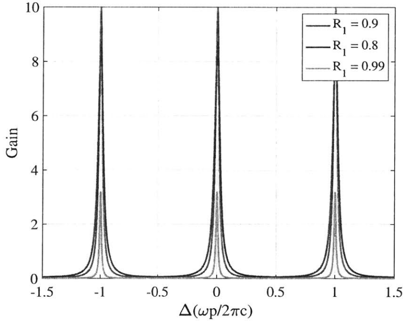
Figure 2-3: Cavity circulating power compared to input power for a number of different FP cavities assuming R_2 = 0.9 .
