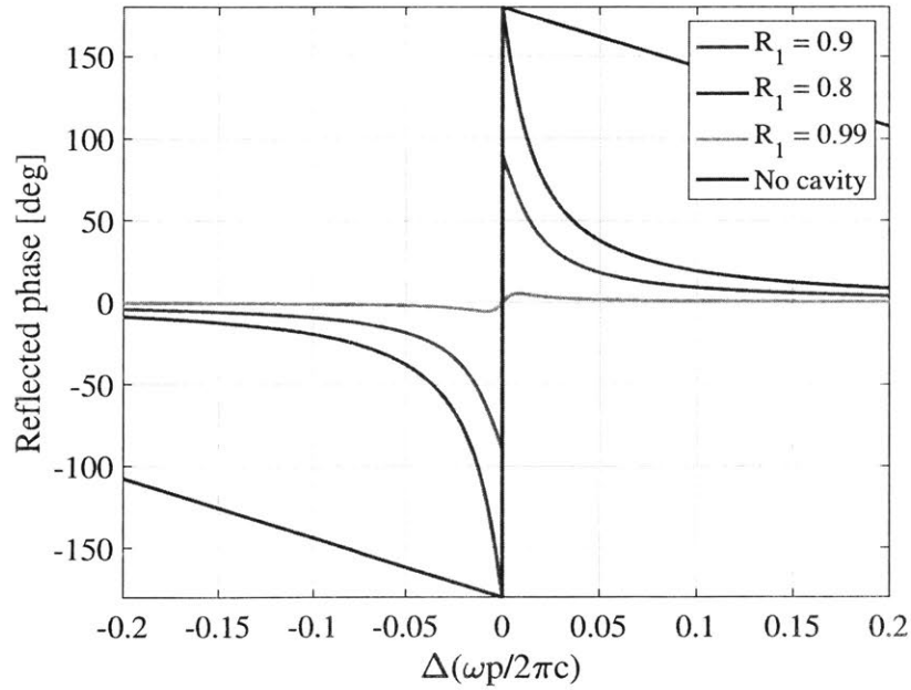
Figure 2-6: Cavity reflected phase for a number of different FP cavities assuming R_2 = 0.9 . Also included is a trace for the phase shift for a single end mirror and no cavity. As expected, the cavity introduces a significantly larger phase shift than with just a single mirror.
