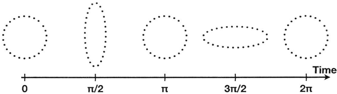
Figure 1-1: The effect of a passing + -polarized gravitational wave traveling into the page on a ring of free masses. This effect has been greatly exaggerated.
