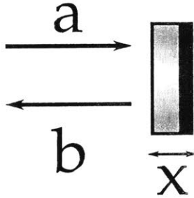
Figure 2-13: Field operators for light incident on and reflected from a perfect reflector free mass. Because we assume a perfectly reflecting mirror, we can ignore the fields on the other side of the mirror.
