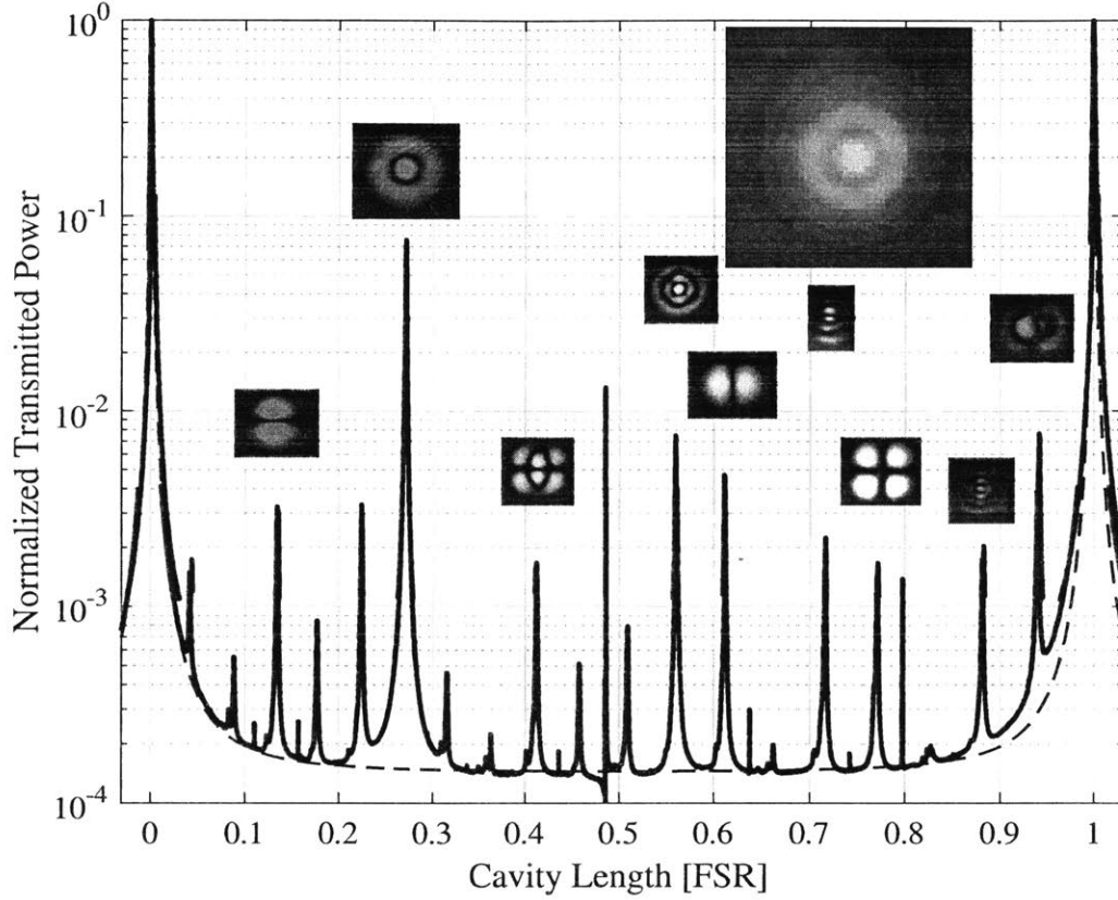
Figure 5-8: Transmission of an optical cavity as the length is swept through a full free spectral range (FSR). Included is the finite width of the \text{TEM}_{00} mode and a DC offset. Narrow peaks are due to leaked s -polarized light, which has a higher finesse and is split due to the intrinsic cavity birefringence. The baseline DC power is suspected to be due to scattered light and not amplified spontaneous emission (ASE), as it scales proportionally to total power. The high content of the Laguerre-Gaussian 10 mode is due to a beam astigmatism that could not be removed with spherical optics. Inset: near-field image of output beam.
