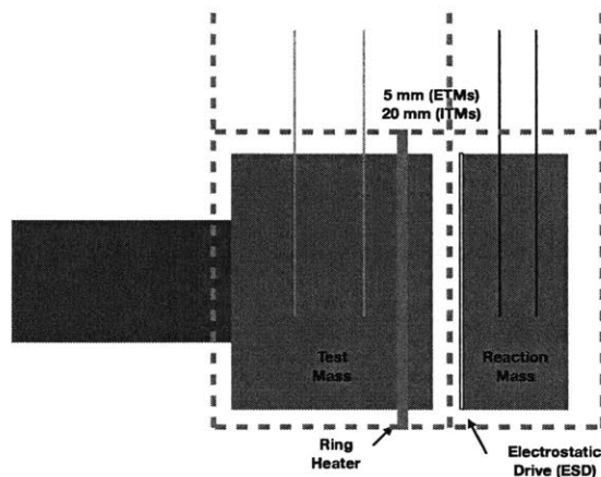
Figure 4-1: Simplified side view of an end test mass/reaction mass and surroundings, including the arm cavity laser beam, the surrounding cage, and ring heater shield. The transmitted laser is omitted. Recall that the test mass is the last stage of the aLIGO quad suspension (figure 1-3).
