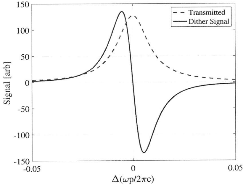
Figure 2-7: Dither locking signal
