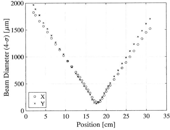
Figure 5-7: M^2 measurement of beam at full power.
