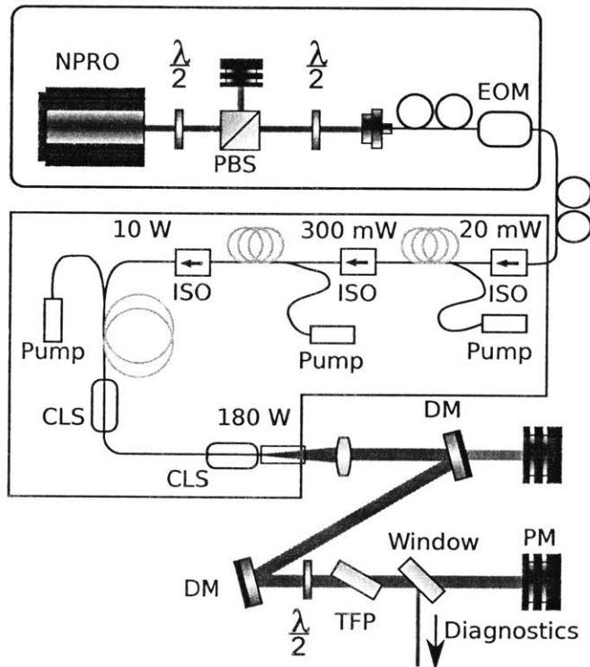
Figure 5-2: Amplifier layout. EOM: in-fiber electro-optic modulator, ISO: fiber isolator, CLS: cladding light stripper, DM: dichroic mirror, TFP: thin-film polarizer, PBS: polarizing beam splitter, PM: power meter.
