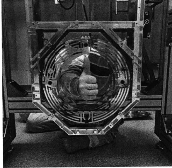
Figure 4-2: The installed end reaction mass (ERM) showing the installed electrostatic drive (ESD) pattern. Prior to O3 the original end reaction masses (ERMs) were replaced with annular ERMs, in which the center section was removed to reduce the effects of squeezed film damping. Photo credit: Gary Traylor and Danny Sellers
