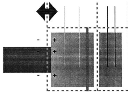
(b) Image charges in the optic cage can couple cage motion to test mass motion.
