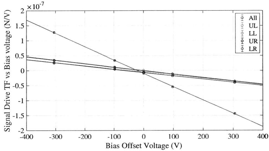
(a) ESD signal trace actuation strength as a function of bias trace voltage. This measurement was also performed with the individual signal trace quadrants (shallow lines) to demonstrate some variation between quadrants.
