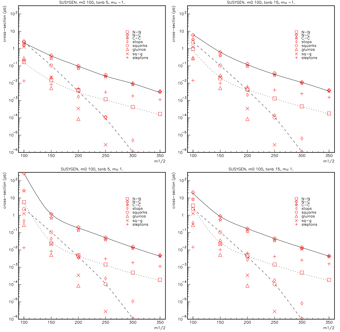
Figure 7.2: Susygen: cross sections (pb) of the supersymmetric particles pairs production as function of m_{1/2} [75]. m_0=100 GeV; \tan\beta=5 (left) and \tan\beta=15 (right); \mu < 0 (up) and \mu > 0 (down); A_0=0 .
