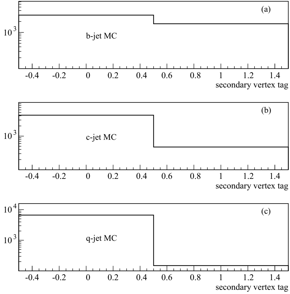
Figure 6.6: Secondary-vertex tag distributions for b , c , and light-quark jets in the Monte Carlo samples.
