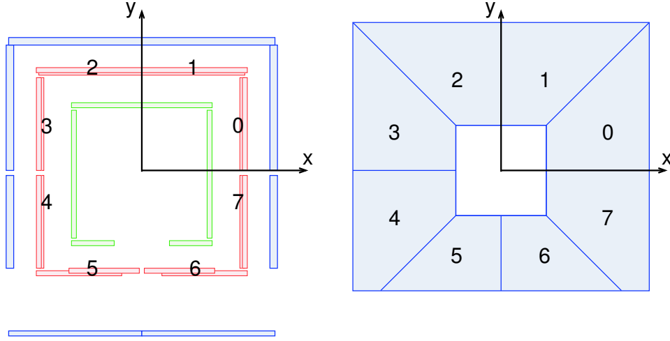
Figure 5.2: View of the chambers of the muon spectrometer in the central (on the left) and in the forward (on the right) region. The digits indicate the octants numbers.
