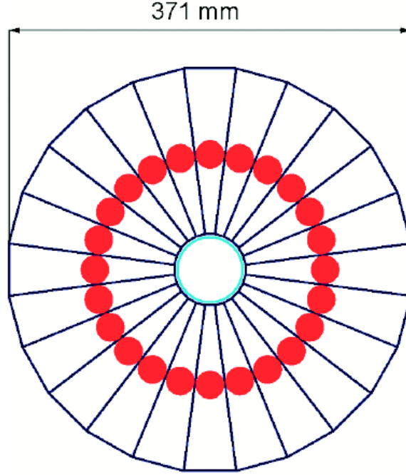
Figure 2.14: Schematic of the Run II Luminosity Monitor (one side). The solid circles represent the locations of the photomultiplier tubes.
