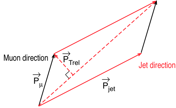
Figure 6.7: P_{Trel} definition.
