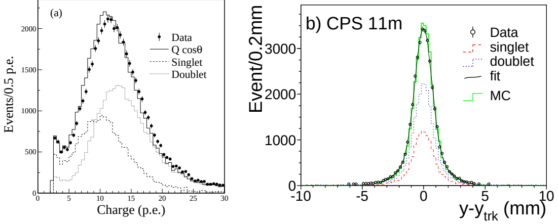
Figure 2.5: Preshower detector cosmic ray muon tests: (a) light yield (p.e. = photoelectrons); (b) fitted track residuals.
