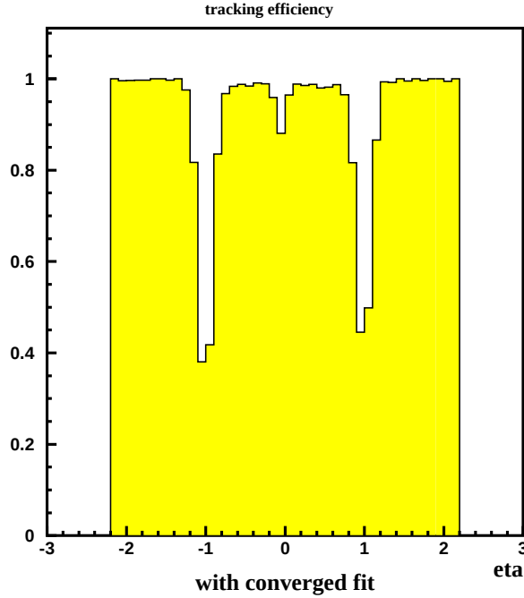
Figure 5.4: Local track reconstruction efficiency as a function of \eta [143].
