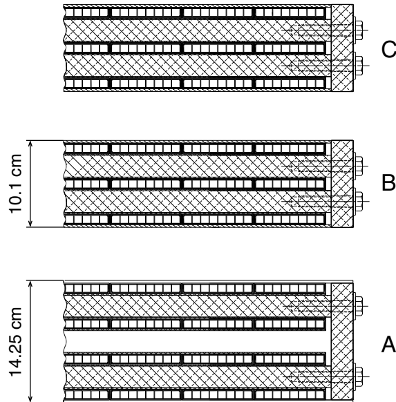
Figure 2.13: Layout of the three MDT planes.
