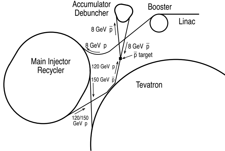
Figure 2.1: The Fermilab accelerator chain.
