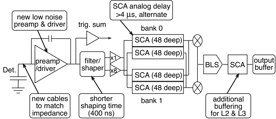
Figure 2.9: Schematic view of the electronics system for the DØ calorimeter at Run II. The added text corresponds to the modification performed after Run I.
