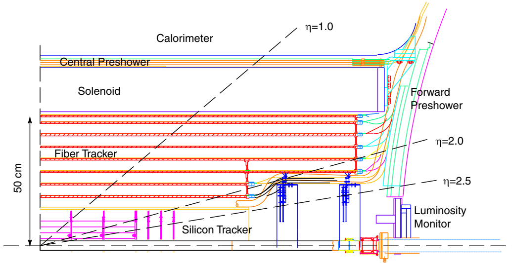
Figure 2.2: r - z view of the DØ tracking system.
