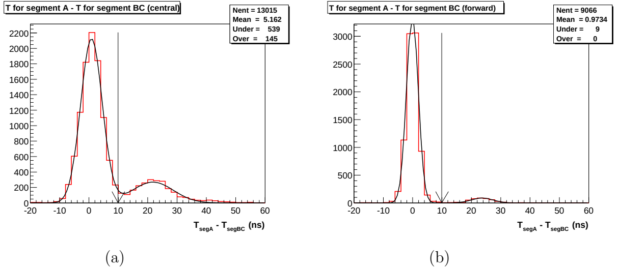
Figure 5.9: Difference between the muon arrival time in the A and in the BC layers for central (a) and forward (b) region.
