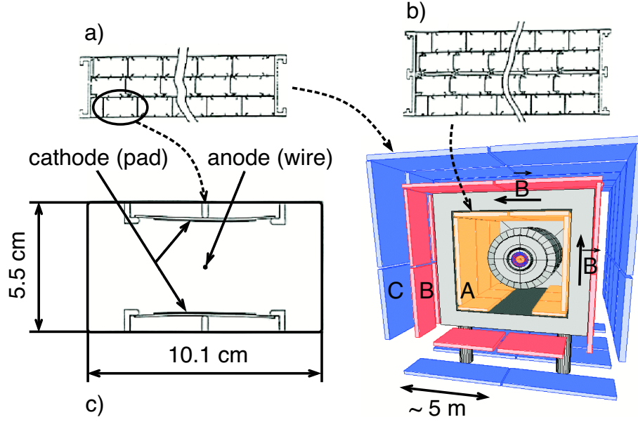
Figure 2.12: WAMUS. (a) is the end view of the 3-deck extrusion. (b) is the end view of the 4-deck extrusion. (c) is the end view of a single cell, including the cathode pad.
