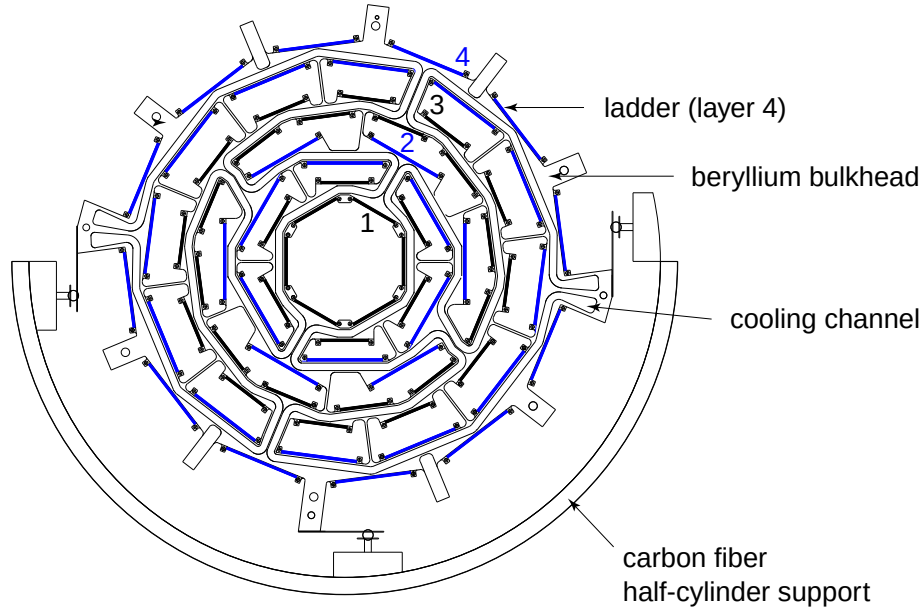
Figure 2.3: Cross sectional r\varphi view of an SMT barrel.
