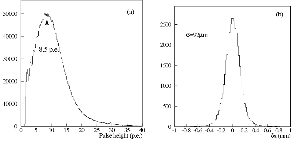
Figure 2.4: CFT cosmic ray test stand results: (a) photoelectron yield per fiber; (b) distribution of doublet residuals from fitted tracks.
