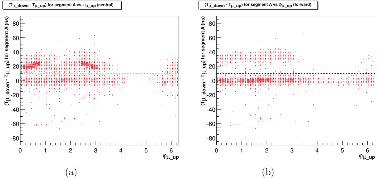
Figure 5.8: Difference between the arrival time of upward muon and downward muon for central (a) and forward (b) region.
