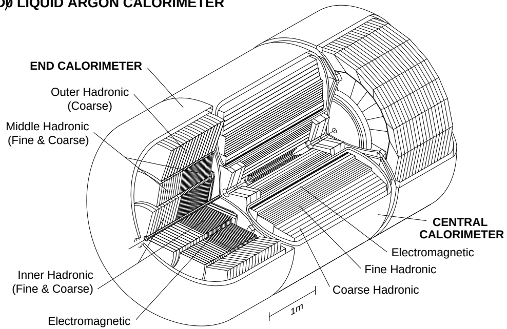
Figure 2.7: Cutaway view of the DØ calorimeter.
