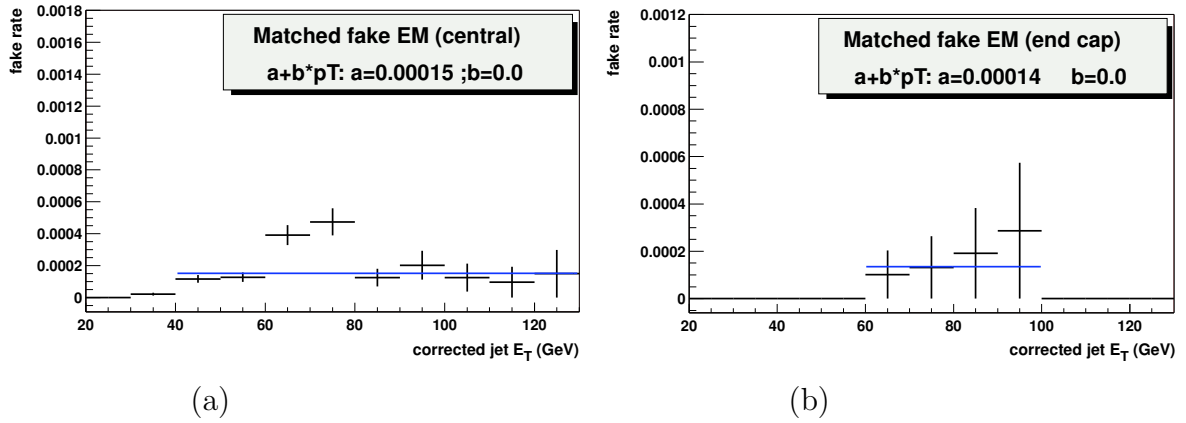
Figure 4.12: Electron fake rate with central track matching condition for central (a) and forward (b) region.
