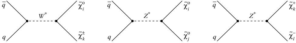
Figure 7.1: Gaugino pair production diagrams ( i, j = 1 \dots 4 ; k, l = 1, 2 ) at the Tevatron.
