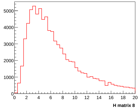
Figure 4.3: Distribution of H-matrix \chi^2 for the EM clusters in a MC \gamma^*/Z \rightarrow ee sample.
