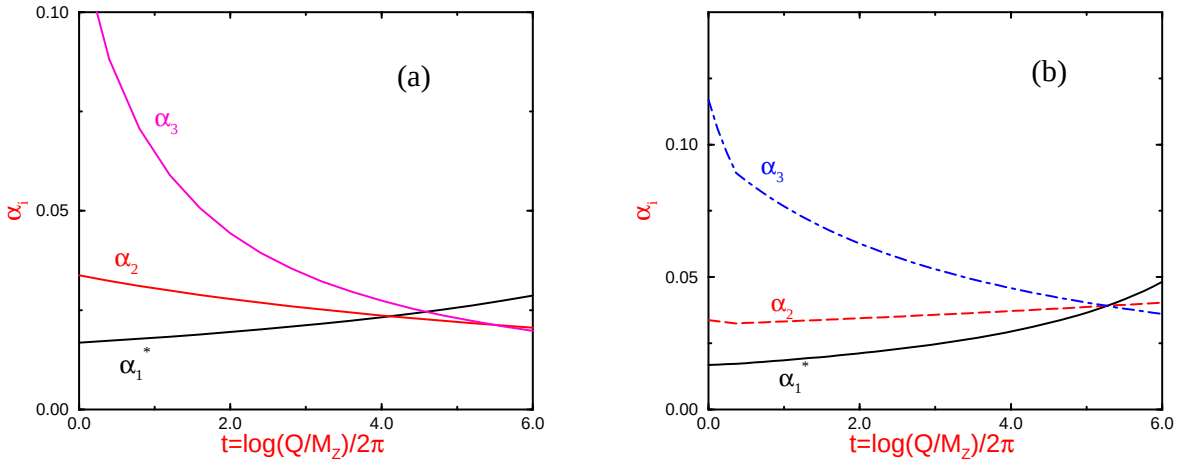
Figure 1.6: Evolutions of the coupling constants. Shown are the evolutions of the U(1) ( \alpha_1 ), SU(2) ( \alpha_2 ), and SU(3) ( \alpha_3 ) coupling constants with the energy scale. Plot (a) shows the evolution in the Standard Model. Plot (b) is the evolution within the MSSM. The addition of the sparticles changes the running of the coupling strengths so that they all converge at the same point, suggesting that the interactions arise from a single grand unified force.
