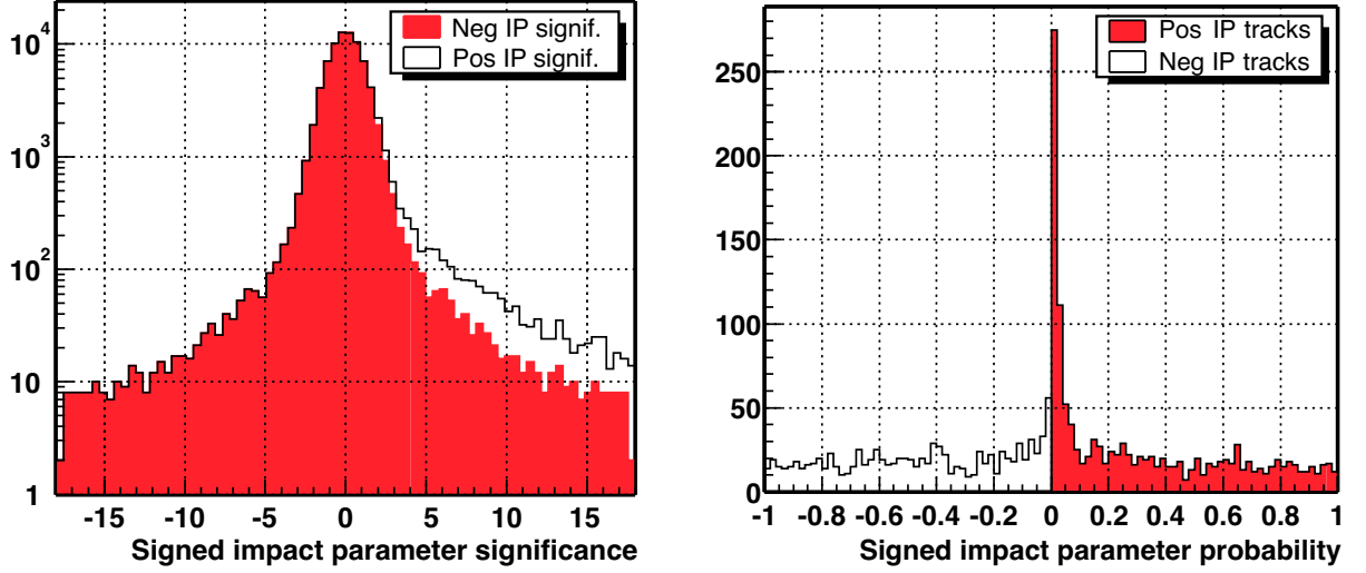
Figure 6.3: Signed track impact parameter significance (left) and track impact parameter probabilities (right) [147].
