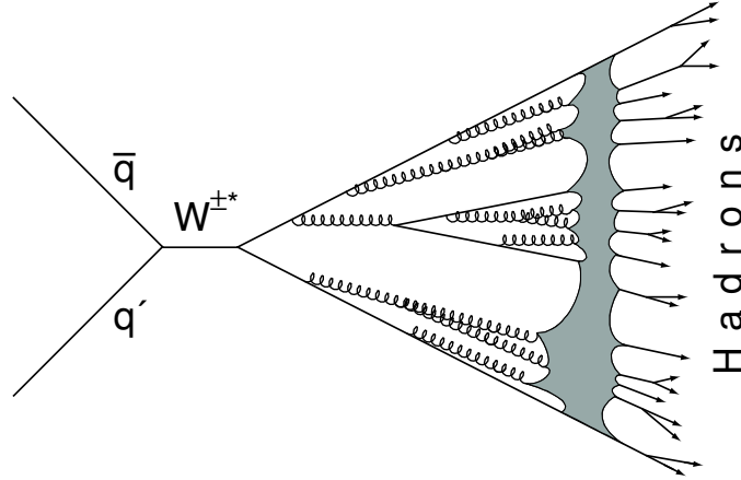
Figure 1.1: An example of Hadronization. Two high energy quarks on the left are shown annihilating into a W boson. The W then decays into two high energy quarks which hadronize by emitting many gluons (curly lines) that emit q\bar{q} pairs. The grey region is where the quarks form hadrons, the particles that are observed in a detector. The direction of the cartoon lines do not represent real particle directions. The final hadrons will be collimated along the direction of their parent quarks or gluons forming jets. There will be at least two jets from the two quarks that decayed from the W . Hard gluons decaying from those quarks may also produce jets (final state radiation). The jets will be balanced in the event if the incident quarks have the same energy (if not, the jets will balance only in azimuthal angle). For example, if two jets are produced and the W is not boosted, the jets will have the same energy and will appear back to back.
