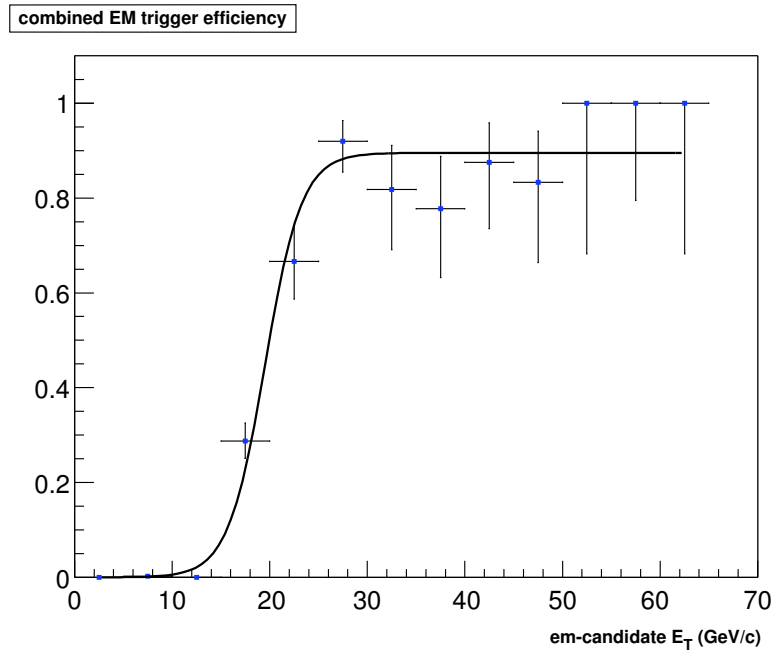
Figure 8.1: Trigger efficiency as a function of the EM-candidate energy.
