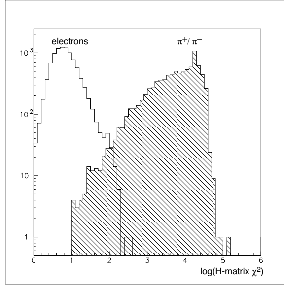
Figure 4.2: Distribution of H-matrix \chi^2 for the EM clusters in a MC electron and pion samples [131].
