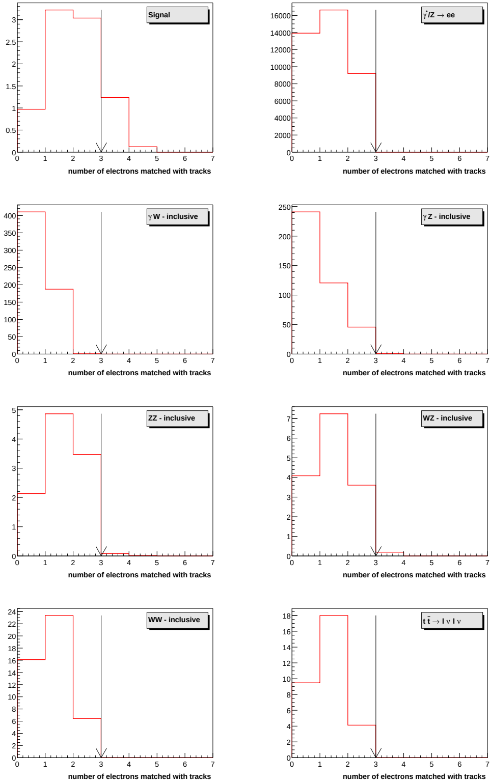
Figure 8.7: Distributions of the number of electrons ( p_T > 15 GeV) matched with a central track and the chosen cut (shown as vertical arrow). For the signal, a typical point in the mSUGRA parameter space, m_0 = 200 GeV/ c^2 and m_{1/2} = 260 GeV/ c^2 has been chosen.
