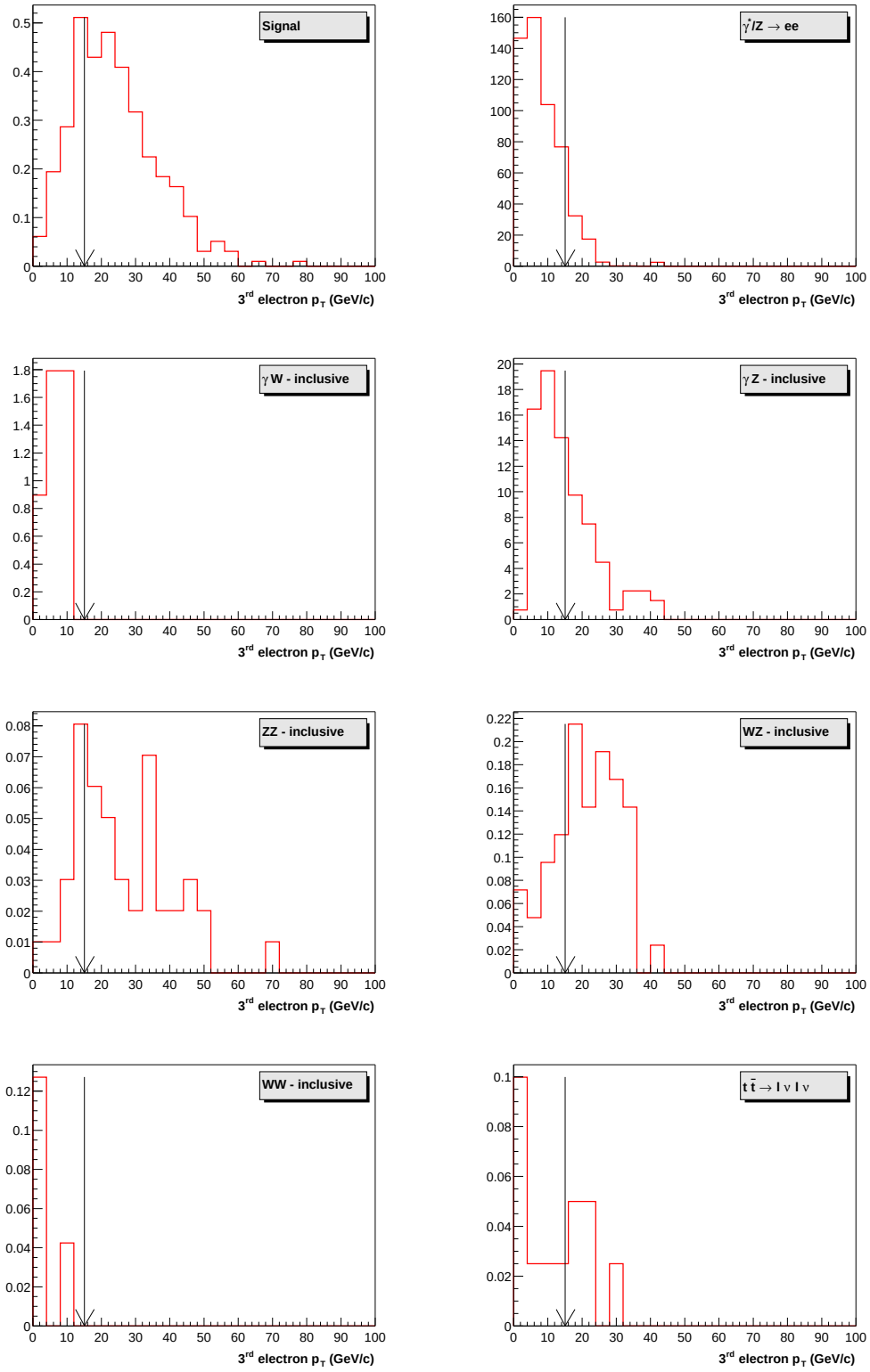
Figure 8.5: p_T distributions of the third highest p_T electron and the chosen cut (shown as vertical arrow). For the signal, a typical point in the mSUGRA parameter space, m_0 = 200 \text{ GeV}/c^2 and m_{1/2} = 260 \text{ GeV}/c^2 has been chosen.
