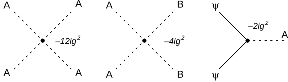
Figure 1.3: Interactions involving the A scalar particle. The vertex factors are shown with each interaction.
