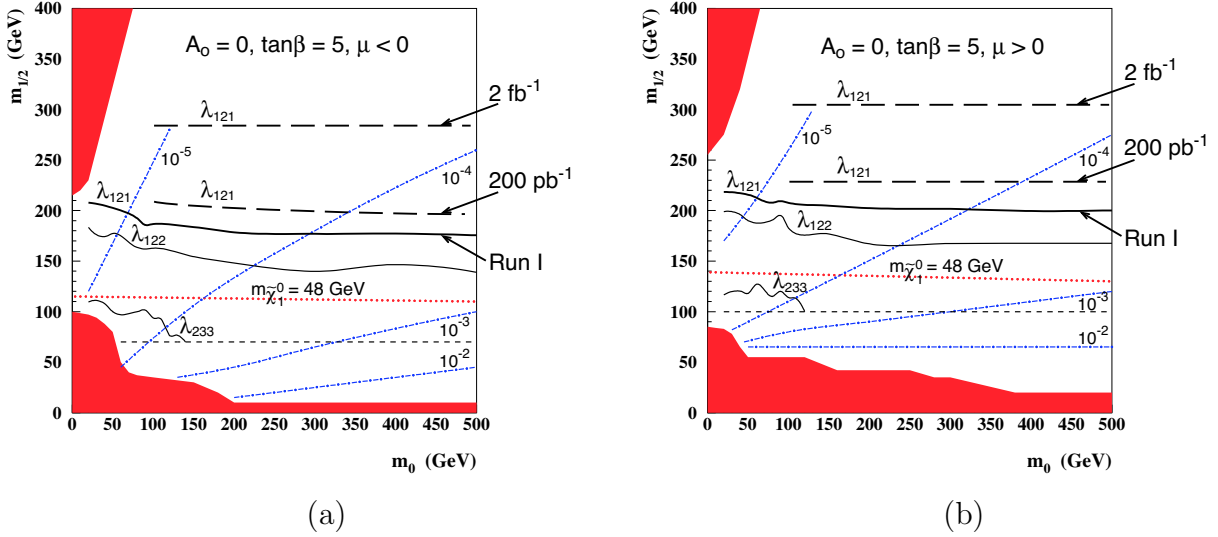
Figure 7.5: Exclusion contour in the m_0 - m_{1/2} plane for A_0 = 0 , \tan \beta = 5 , \mu < 0 (a) and \mu > 0 (b) and for the case of finite \lambda_{121} , \lambda_{122} and \lambda_{233} couplings. The Run I limits [76] are shown as solid lines. For the case of \lambda_{121} coupling expected limits for different integrated luminosity ( 200 \text{ pb}^{-1} and 2 \text{ fb}^{-1} ) are shown as bold dashed lines. The exclusion regions at 95% C.L. correspond to the spaces below the lines labelled with the coupling types, and above the dash-dotted curves specifying the numerical values of \lambda .
