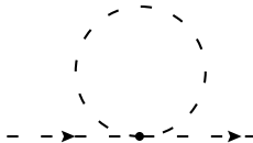
Figure 1.2: Self interaction diagram of fundamental scalars. This diagram is quadratically divergent.
