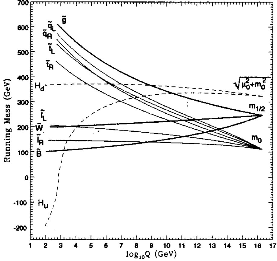
Figure 1.7: Evolution of sparticle mass parameters in Minimal Supergravity. This plot shows the mass parameters of various sparticles vs. energy scale ( Q ). Note that the gauginos are in states before electroweak symmetry breaking ( \tilde{W} and \tilde{B} ). The Higgs mass parameter running negative is at the origin of EWSB. These evolutions are for a particular choice of the model parameters. A different choice of m_0 , m_{1/2} , and the other parameters will lead to different evolutions. For some values of the parameters, the Higgs mass stays positive which means that EWSB is not predicted by those models.
