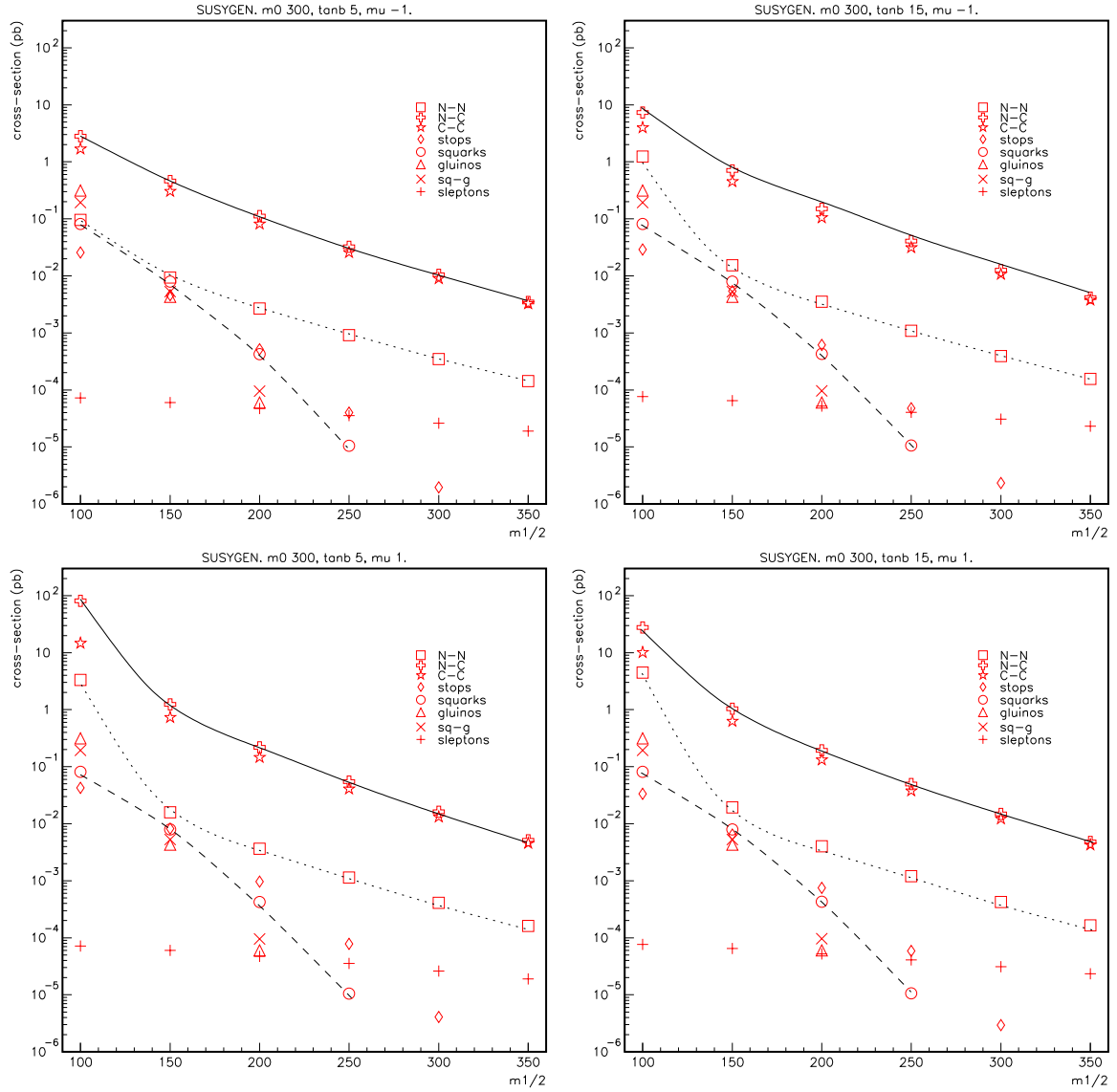
Figure 7.3: Susygen: cross sections (pb) of the supersymmetric particles pairs production as function of m_{1/2} [75]. m_0 = 300 GeV; \tan\beta=5 (left) and \tan\beta = 15 (right); \mu < 0 (up) and \mu > 0 (down); A_0 = 0 .
