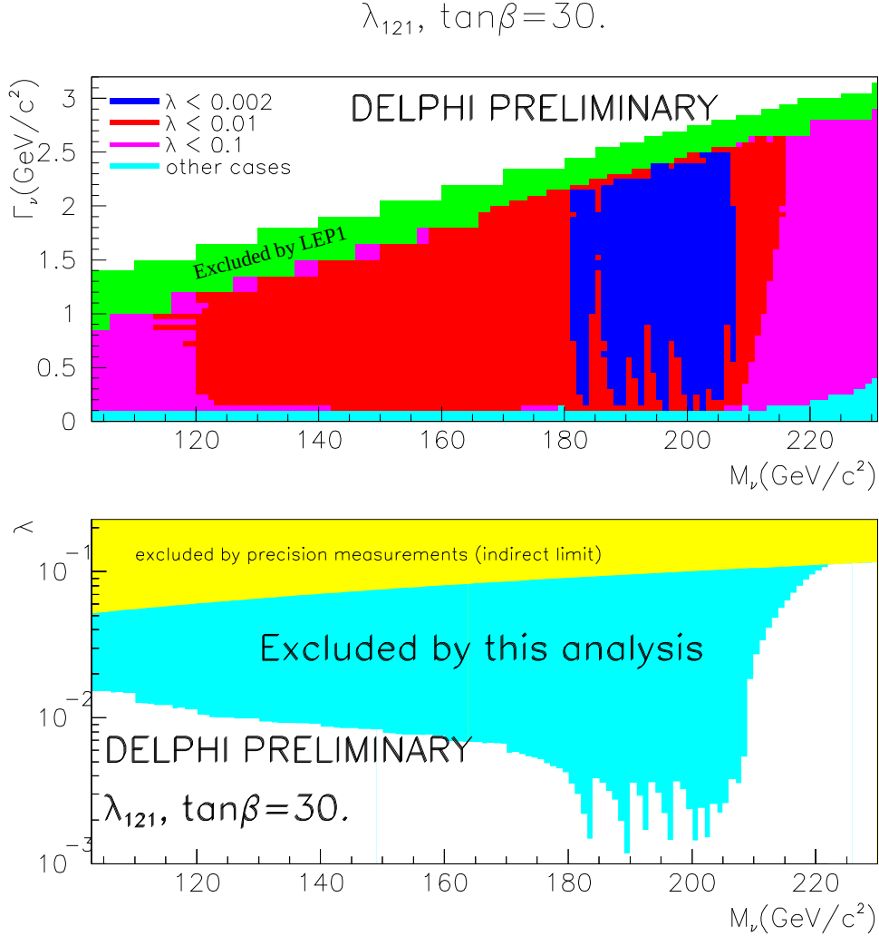
Figure 1.10: For \tan\beta = 30 , upper limit on \lambda_{121} as a function of M_{\tilde{\nu}} and \Gamma_{\tilde{\nu}} (top) and as a function of M_{\tilde{\nu}} and assuming \Gamma_{\tilde{\nu}} > 150 \text{ MeV}/c^2 (bottom). The indirect limit coming from precision measurements is given assuming M_{\tilde{e}_R} = M_{\tilde{\nu}} [28].
