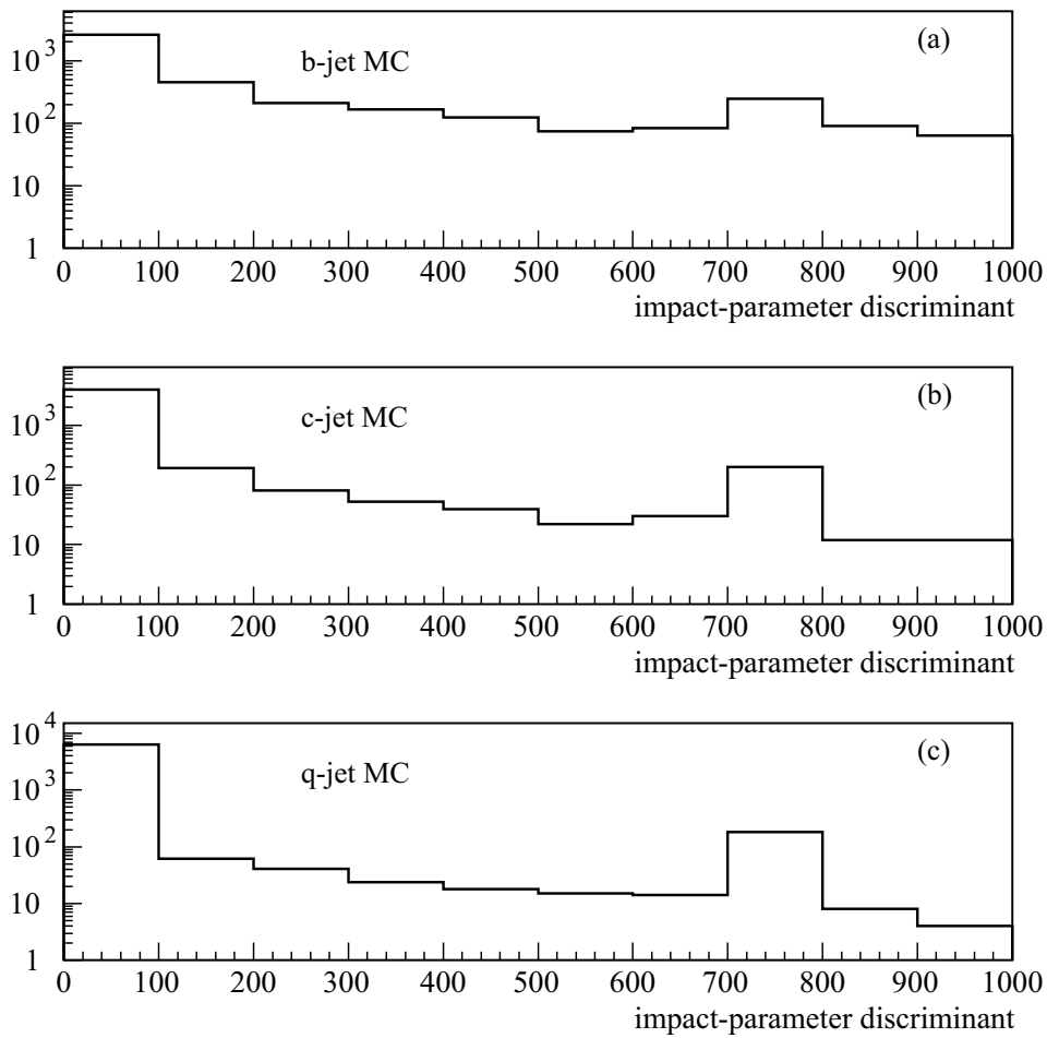
Figure 6.4: Impact-parameter discriminant ( -\ln(P_N) ) distributions for b , c , and light-quark jets in the Monte Carlo samples ("non-taggable" jets due to a dearth of reconstructed tracks have a discriminant of zero, and are included in the plot) [149].
