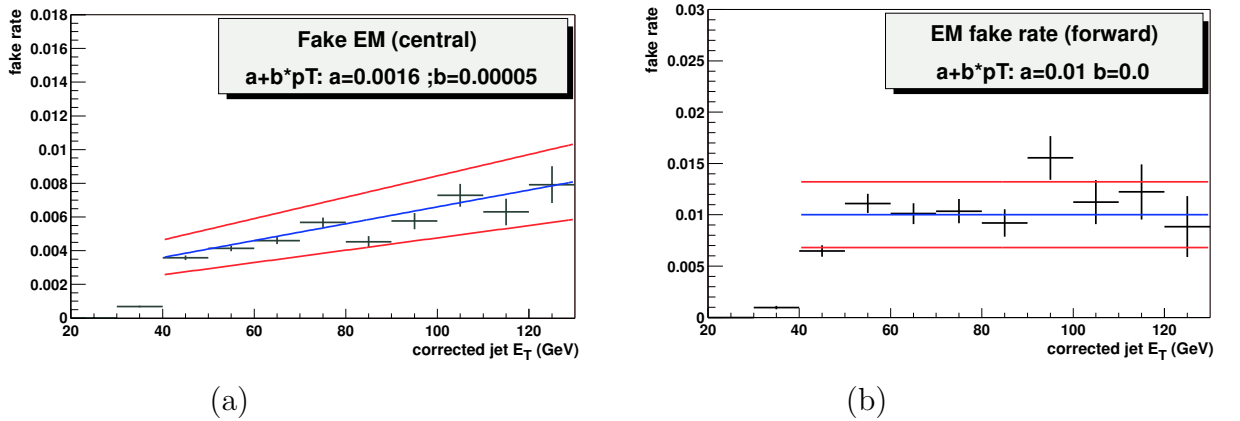
Figure 4.9: Nominal fake electron rate obtained from the jet triggers for central (a) and forward (b) region. Low-energy "turn-off" is the artifact of the various thresholds, amplified by jet energy corrections.
