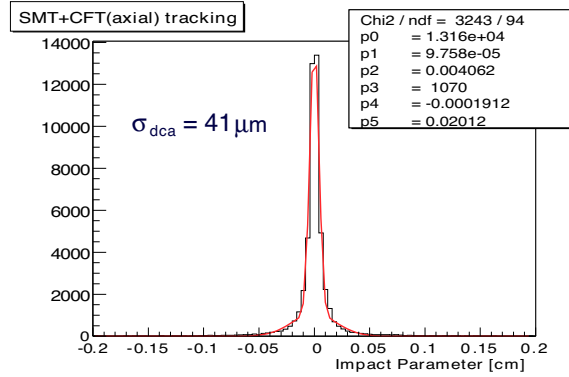
Figure 6.2: Resolution of the impact parameter in the transverse plane [146]
