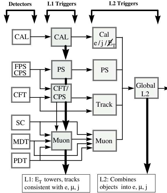
Figure 3.1: Structure of the levels 1 and 2 of the DØ triggering system.
