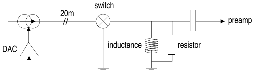
Figure 2.10: Schematic diagram of the measuring chain.
