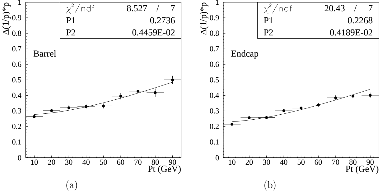
Figure 5.5: Transverse momentum resolution of the reconstructed local track for central (a) and forward (b) region [143].
