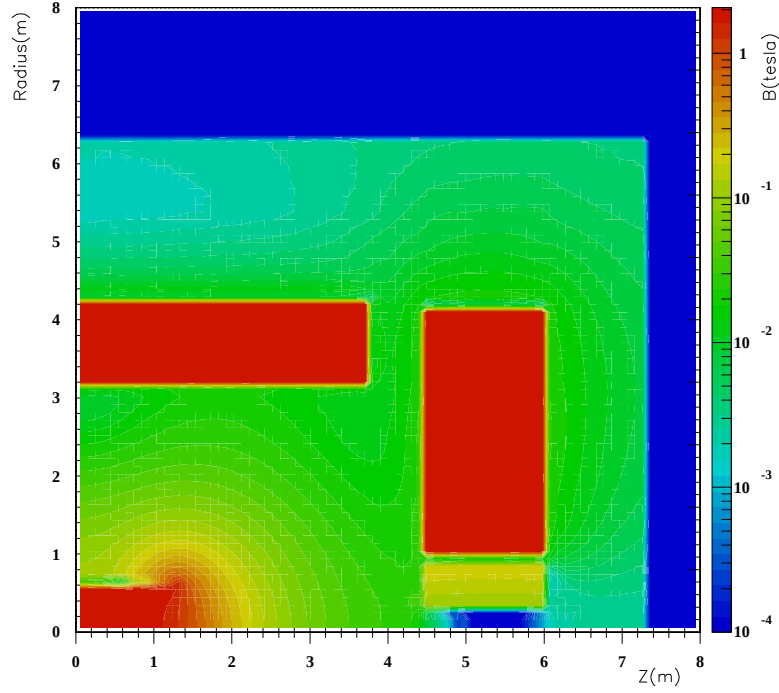
Figure 5.1: Magnetic field map in the DØ detector calculated by the TOSCA program [144].
