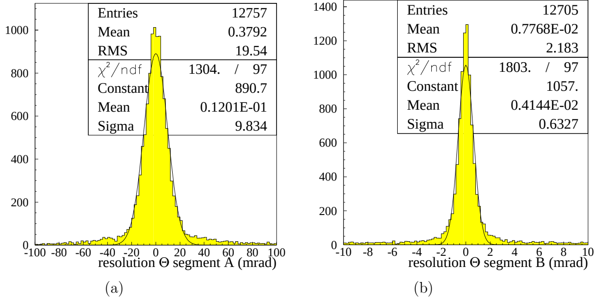
Figure 5.3: Angular resolution (in mrad) of the segments deviation for the layer A (a) and layers BC (b) [143].
