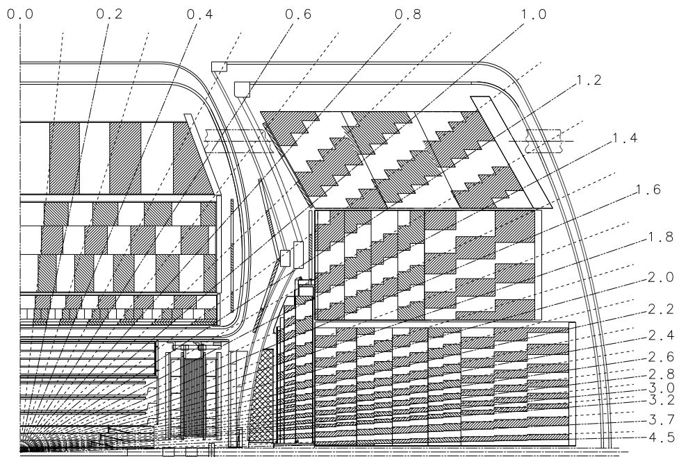
Figure 2.8: One quarter view of the calorimeter.
