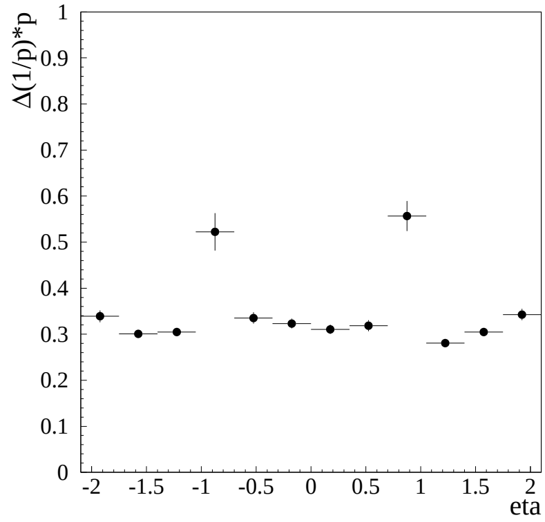
Figure 5.6: Track transverse momentum resolution as a function of \eta for reconstructed local muon tracks [143].
