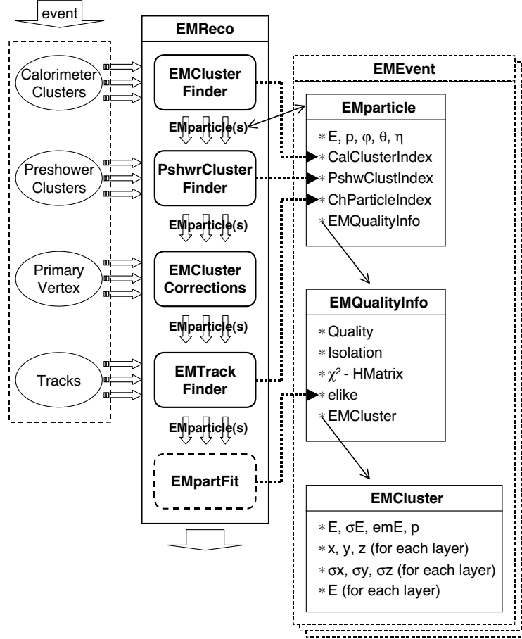
Figure 4.7: General structure of the DØ electron reconstruction program EMReco.
