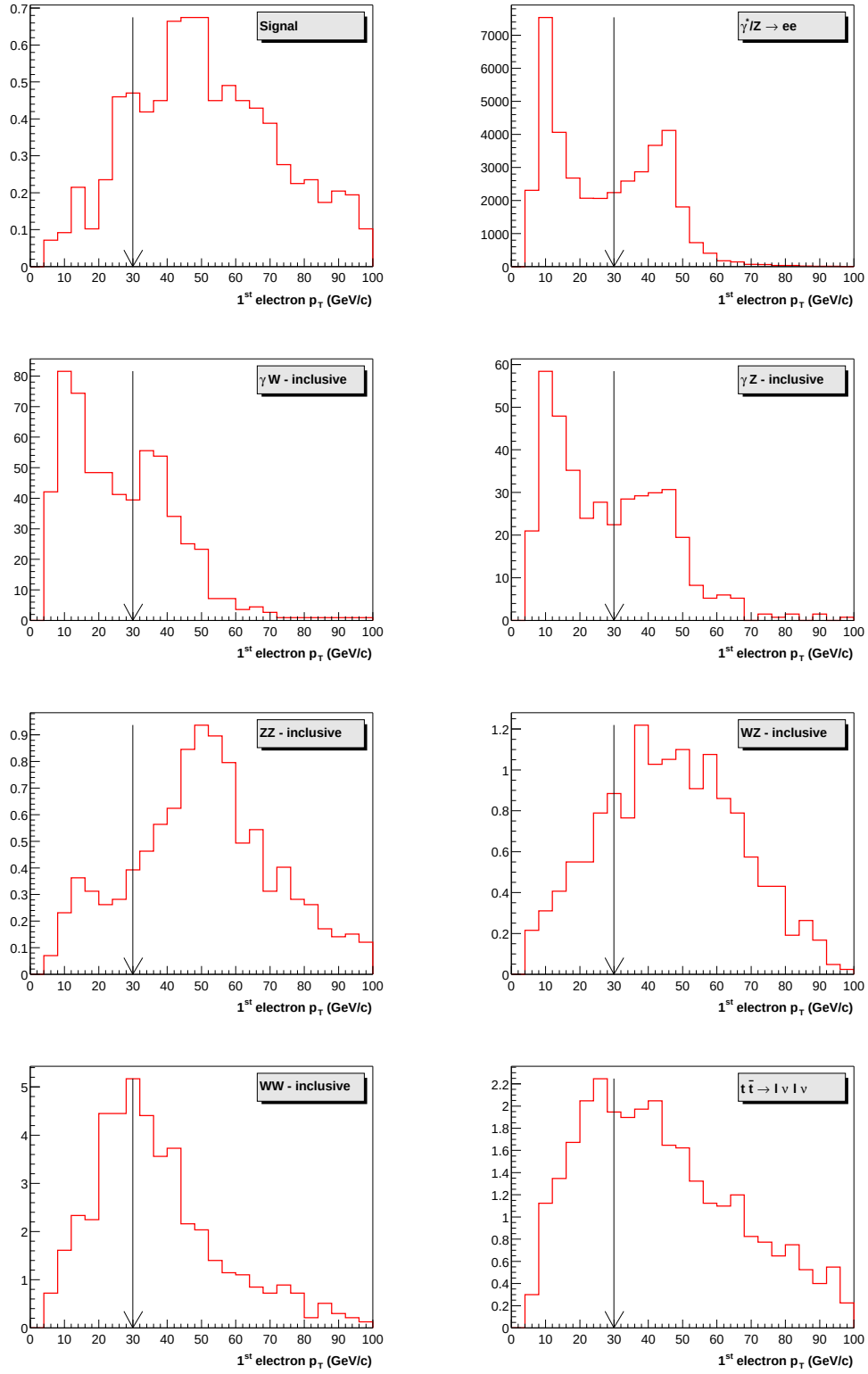
Figure 8.3: p_T distributions of the first highest p_T electron and the chosen cut (shown as vertical arrow). For the signal, a typical point in the mSUGRA parameter space, m_0 = 200 \text{ GeV}/c^2 and m_{1/2} = 260 \text{ GeV}/c^2 has been chosen.
