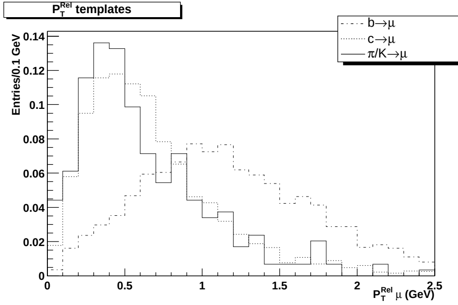
Figure 6.8: Muon P_{Trel} distribution of three MC samples. Solid is QCD, dotted c\bar{c} , dashed b\bar{b} [153].
