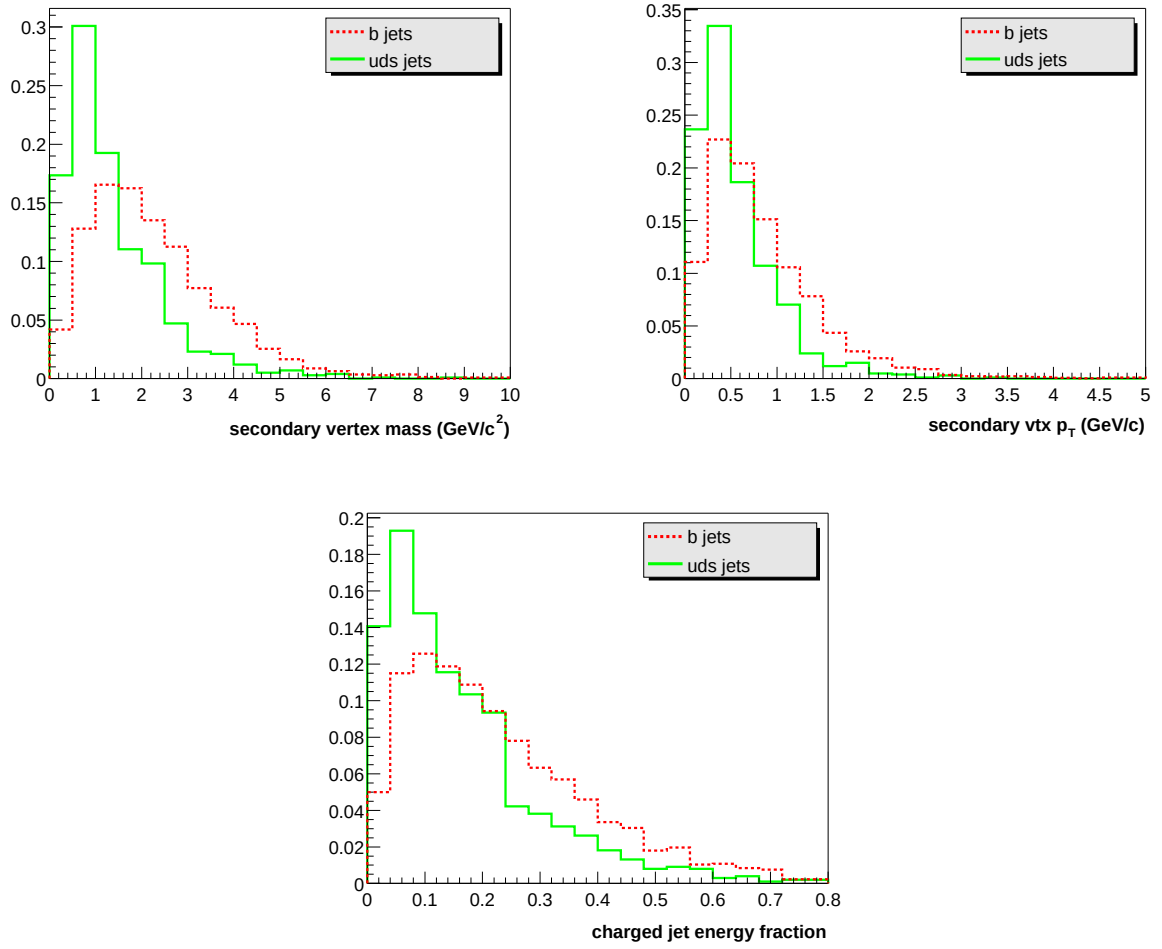
Figure 6.10: Distribution of discriminating variables for uds and b -quark jets.
