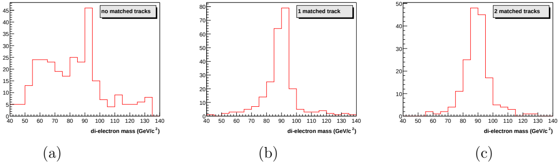
Figure 4.6: Invariant mass distributions for di-electron pairs in Run II data if a) no cluster is matched to a track, b) one and only one cluster is matched to a track and c) when both clusters are matched to a track.
