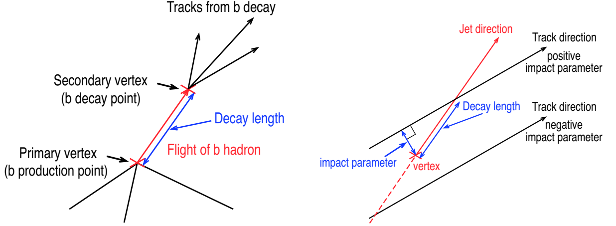
Figure 6.1: Schematic decay pattern of a b -hadron (left) and representation of the signed impact parameter with respect to primary vertex (right).
