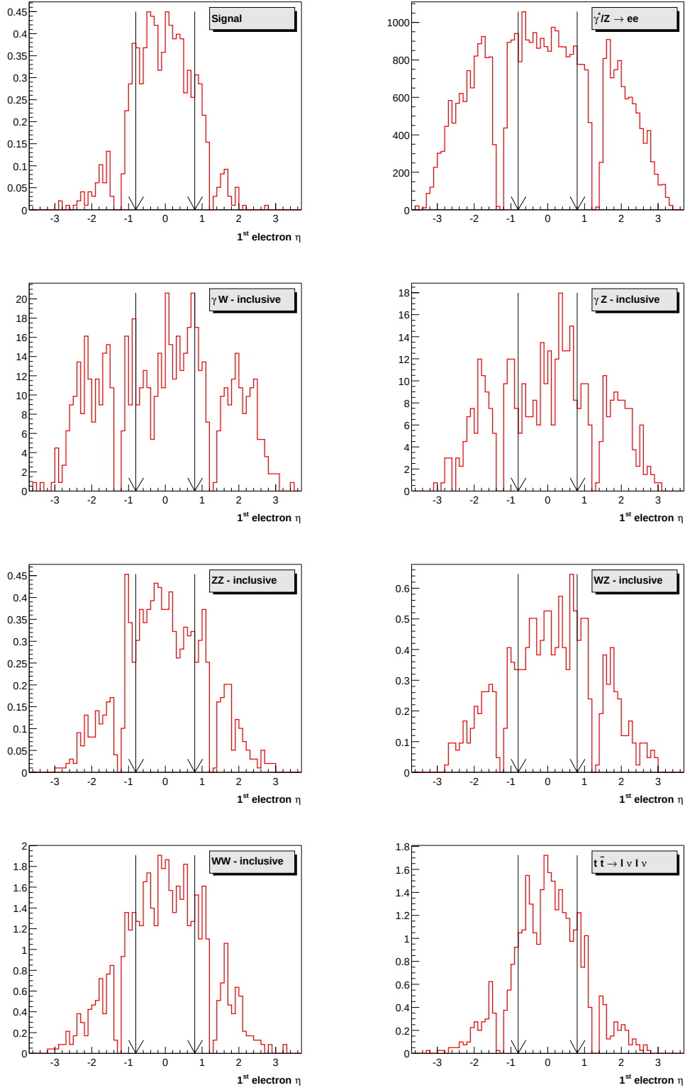
Figure 8.4: \eta distributions of the first highest p_T electron and the chosen cut (shown as vertical arrow). For the signal, a typical point in the mSUGRA parameter space, m_0 = 200 \text{ GeV}/c^2 and m_{1/2} = 260 \text{ GeV}/c^2 has been chosen.
