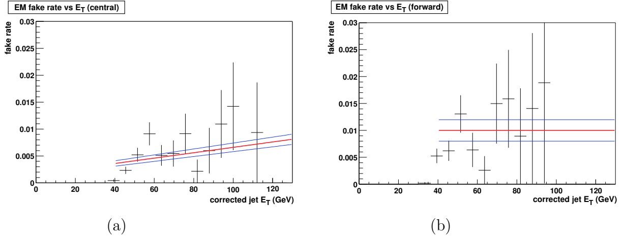
Figure 4.11: Comparison of the nominal fake electron rates with the ones obtained from the muon triggers for central (a) and forward (b) region. Low-energy "turn-off" is the artifact of the various thresholds, amplified by jet energy corrections.
