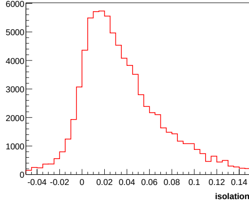
Figure 4.4: Distribution of isolation for the EM clusters in a MC \gamma^*/Z \rightarrow ee sample.
