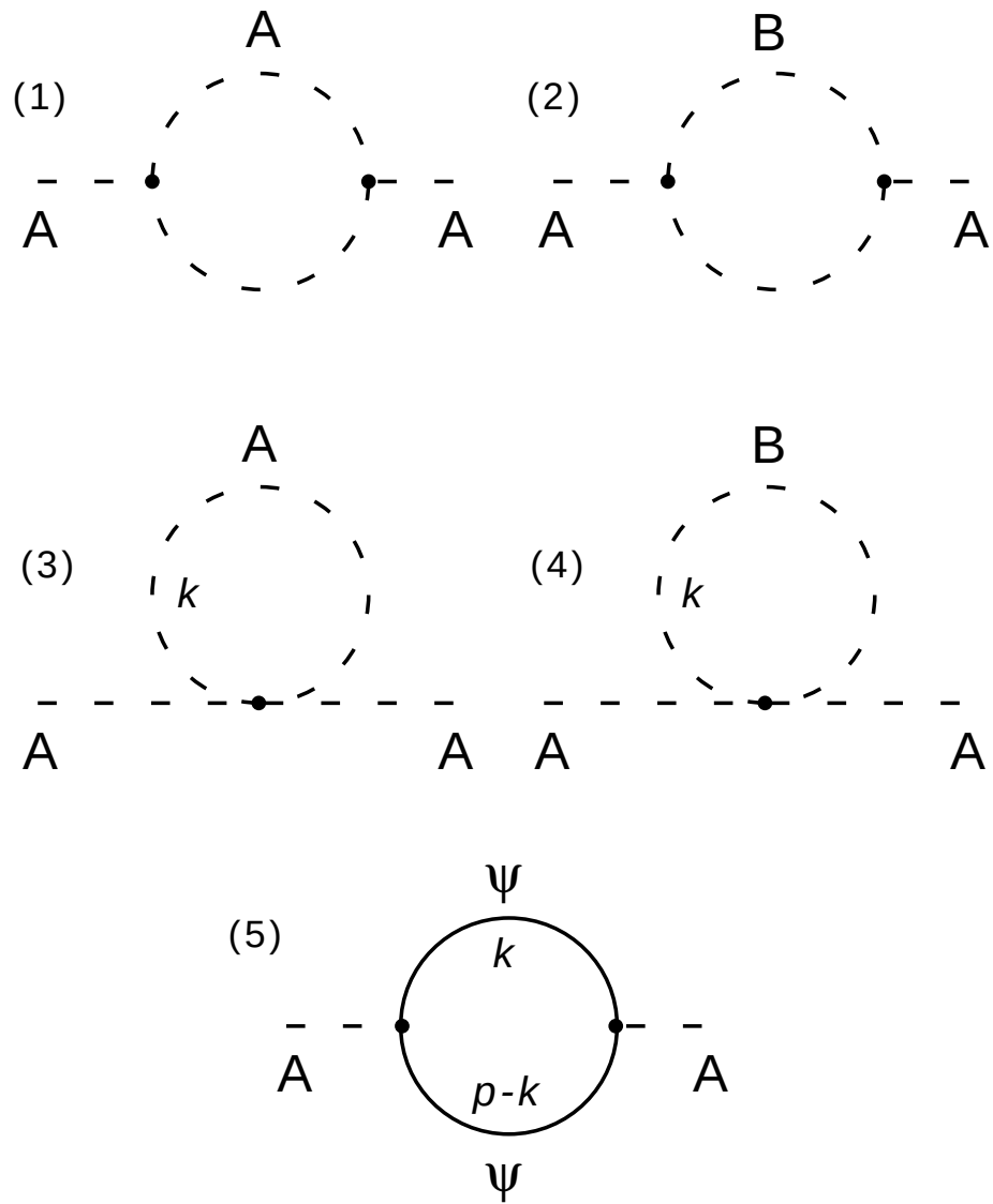
Figure 1.4: Self interaction loop corrections for the A scalar particle.
