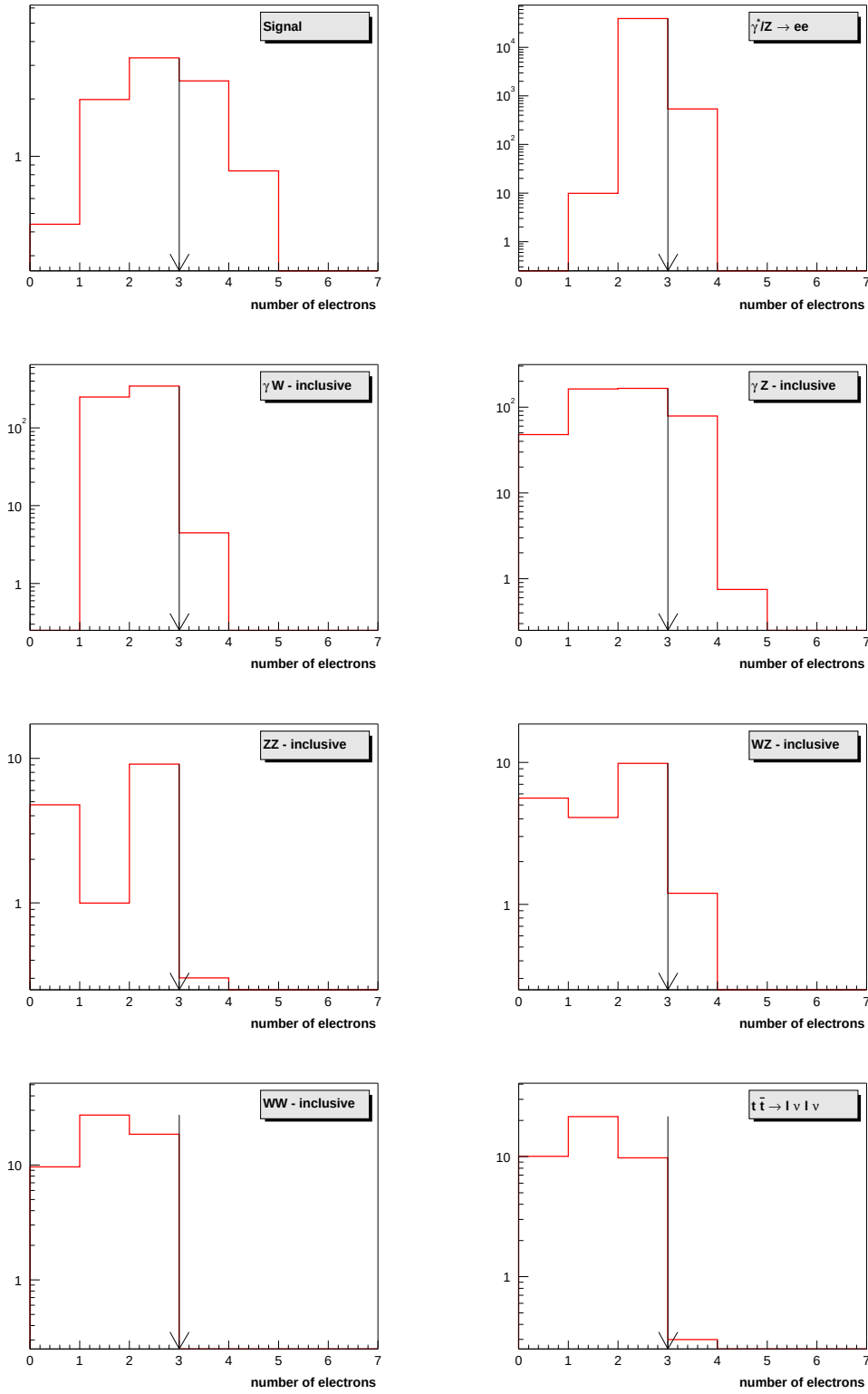
Figure 8.6: Distributions of the number of electrons ( p_T > 15 GeV) and the chosen cut (shown as vertical arrow). For the signal, a typical point in the mSUGRA parameter space, m_0 = 200 GeV/ c^2 and m_{1/2} = 260 GeV/ c^2 has been chosen.
