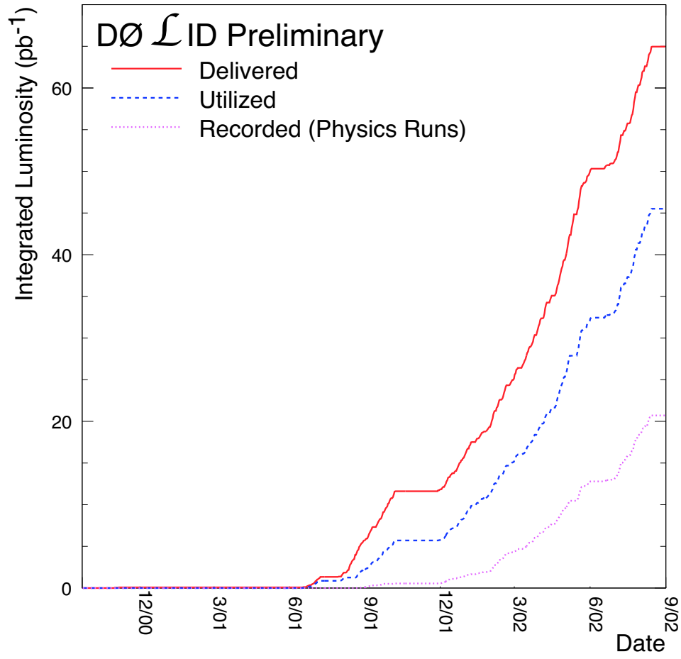
Figure 3.2: Accumulated luminosity as a function of time.
