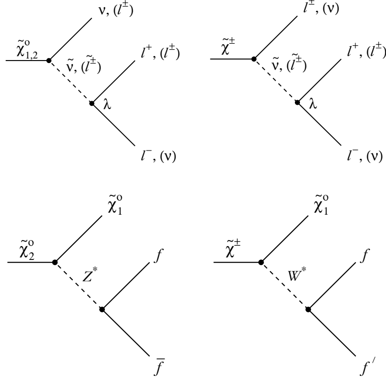
Figure 7.4: Gaugino direct (upper part) and indirect (lower part) decay diagrams for a \lambda_{ijk} coupling.
