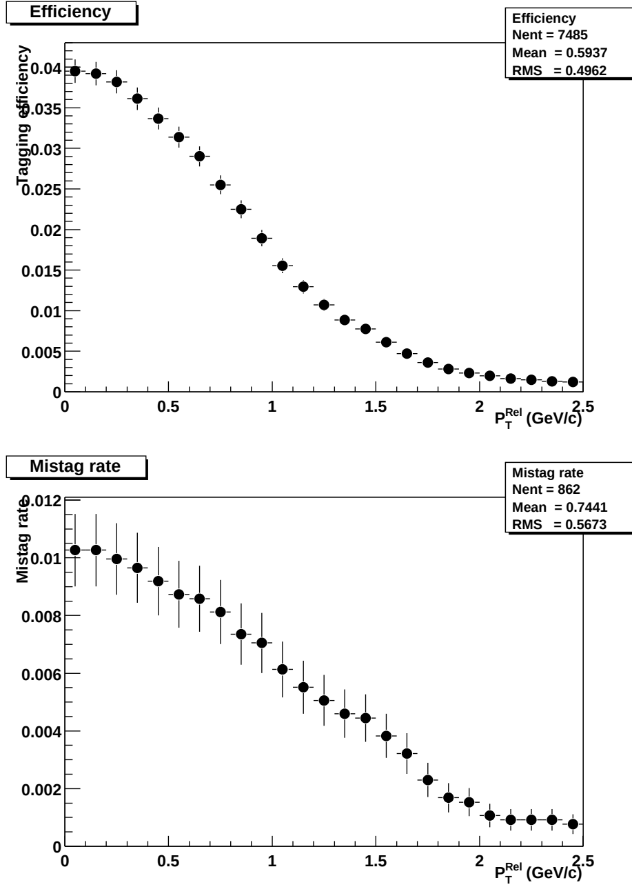
Figure 6.9: The top plot shows the efficiency to tag a b -jet in the b\bar{b} sample as function of the P_{Trel} cut applied. The bottom plot shows the efficiency to tag a light jet in the sample. There is no requirement on an associated muon present with the jet.
