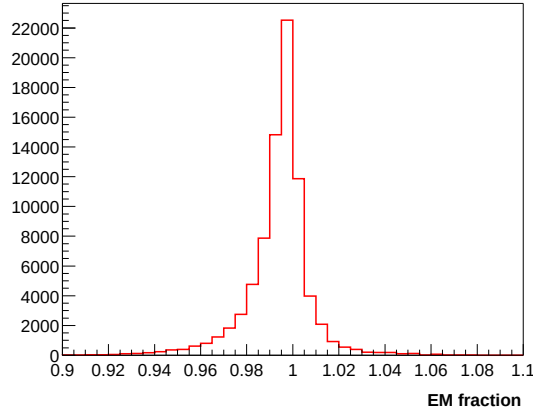
Figure 4.1: Distribution of EM energy fraction for the EM clusters in a MC \gamma^*/Z \rightarrow ee sample.
