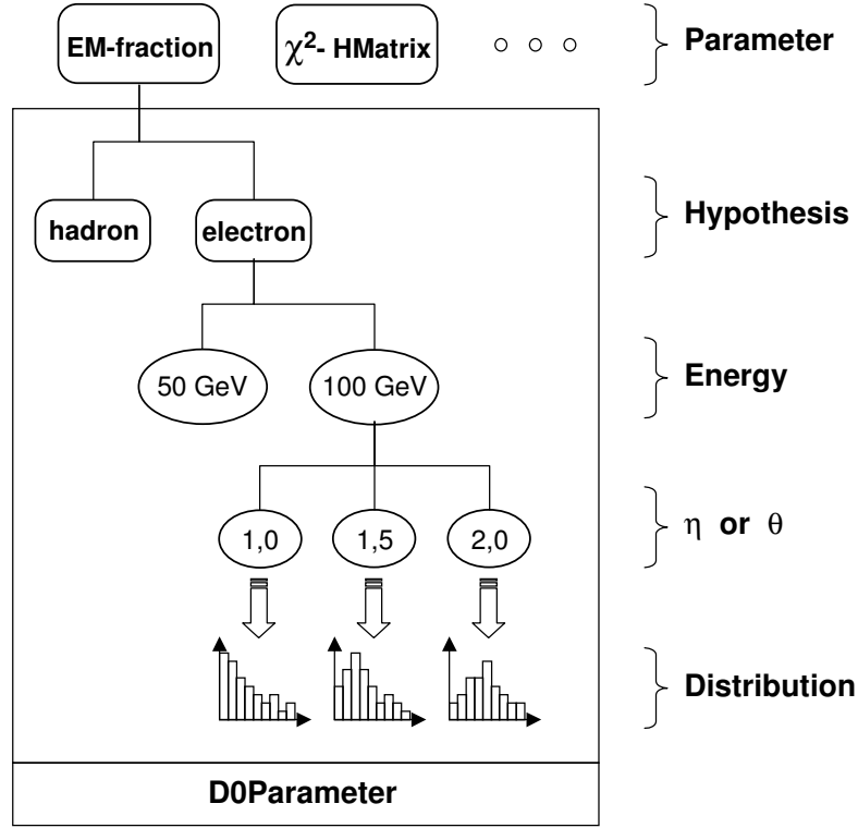
Figure 4.8: Database structure for storing probability distributions for the EM likelihood.
