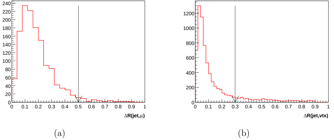
Figure 6.5: \Delta R(jet, \mu) = \sqrt{\Delta\varphi^2 + \Delta\eta^2} between jet and muon (a), and jet and secondary vertex (b) for a b\bar{b} MC sample. Chosen cuts are shown as vertical arrows.
