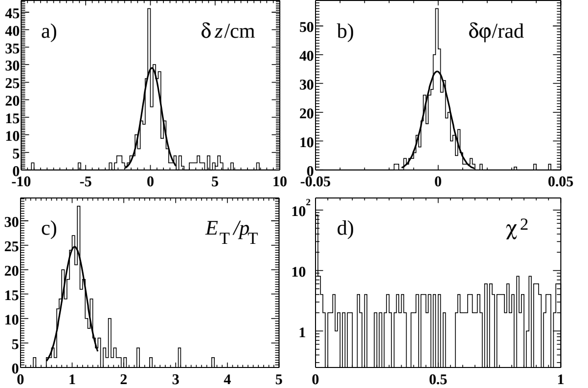
Figure 4.5: Electromagnetic cluster-track matching distributions in the Z Run II data sample. a) \delta z , b) \delta \varphi , c) E_T/p_T and d) \chi^2 probability [132].
