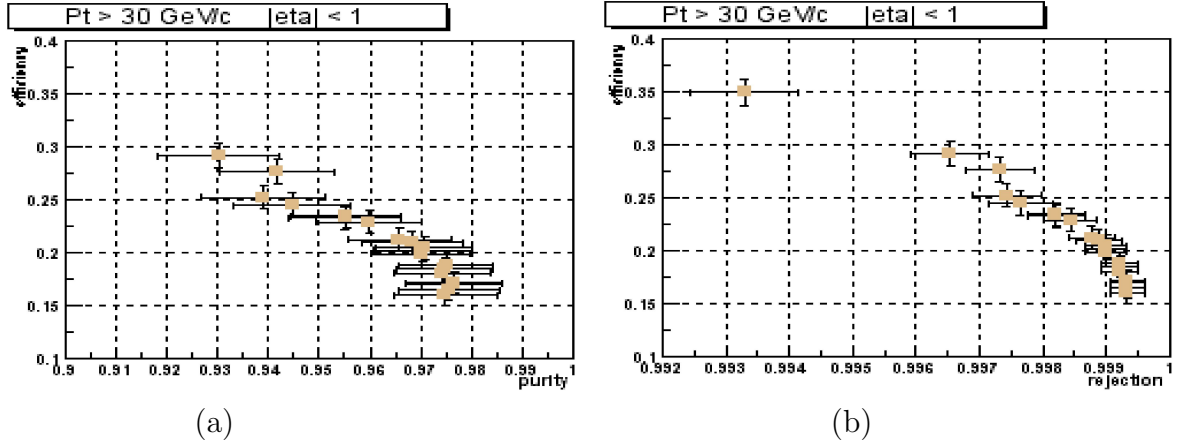
Figure 6.12: Tagging efficiency as a function of the purity of the tagged sample (a) and as a function of the background rejection ratio (b).
