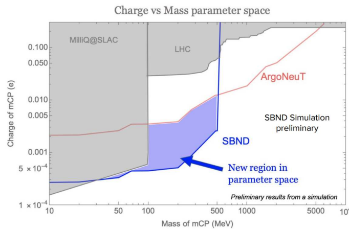
Figure 4. SBND’s preliminary projected sensitivity in millicharged particle phase space.
