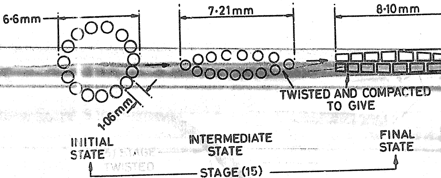
FIG. 4a. AC V 15 STRAND - LOZENGE SECTION CABLE
