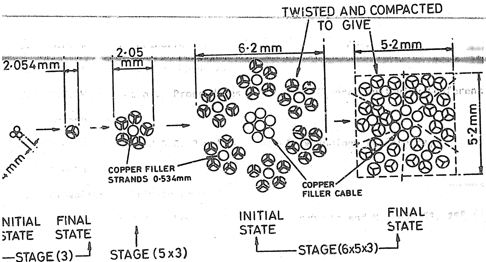
FIG. 1a. AC III, 90 STRAND - SQUARE SECTION CABLE
