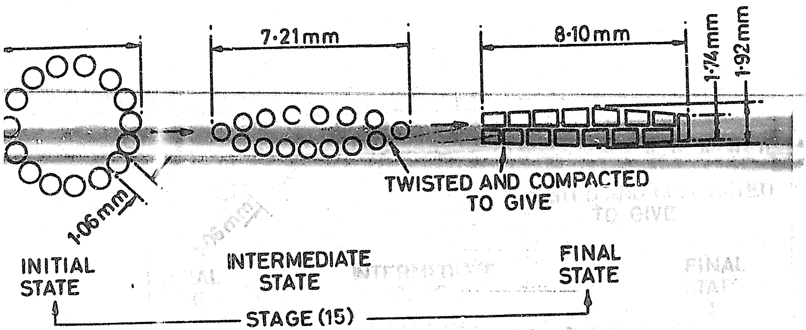
FIG.4a. AC V 15 STRAND - LOZENGE SECTION CABLE
