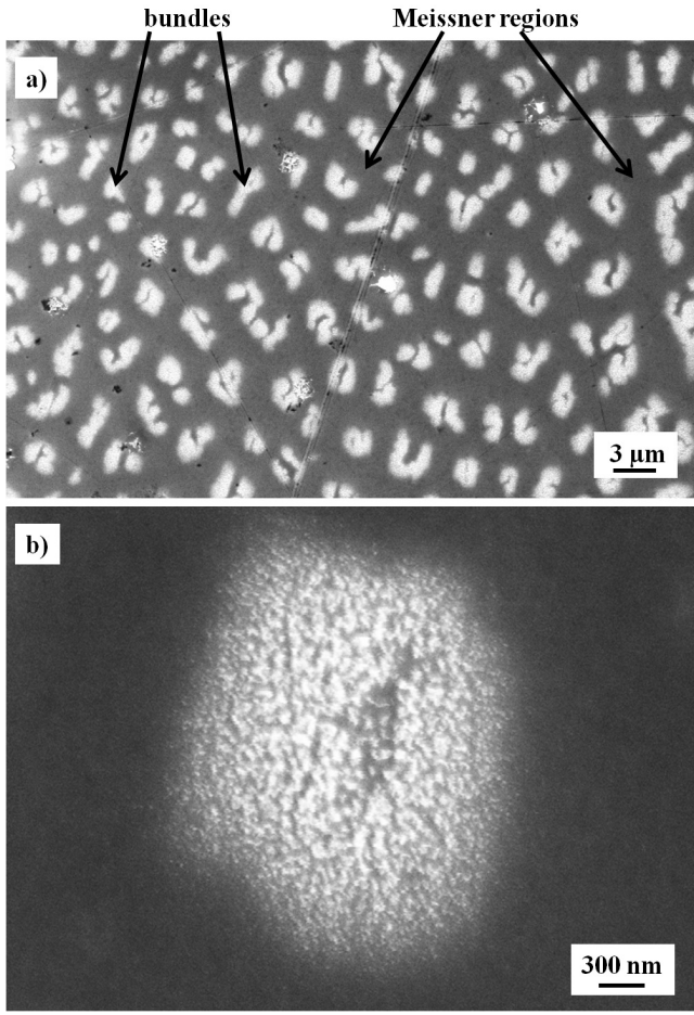
Figure 1: a) Decoration pattern at the magnetic field 10 mT reveals coexistence of “bundles” and Meissner regions. Each bundle carries 80 magnetic flux quanta in average; b) zoom-in of a single bundle.
