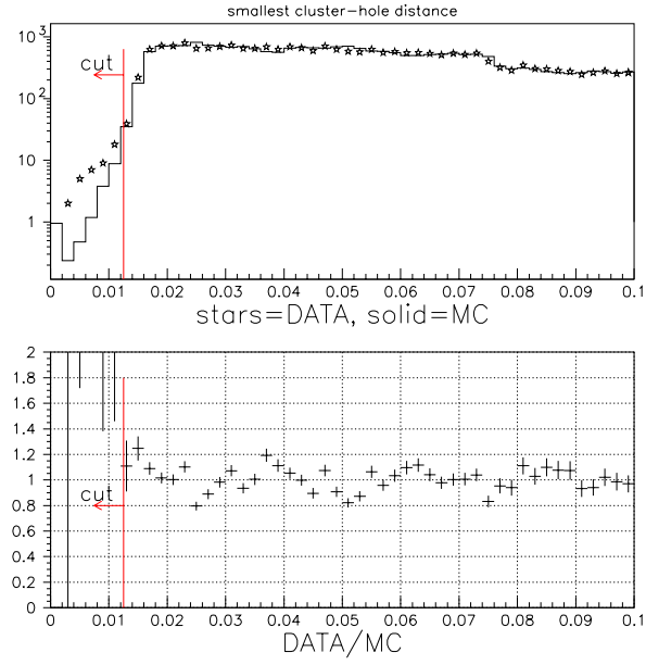
Figure 8.8: Smallest cluster-hole distance (meters). All other cuts are made.
