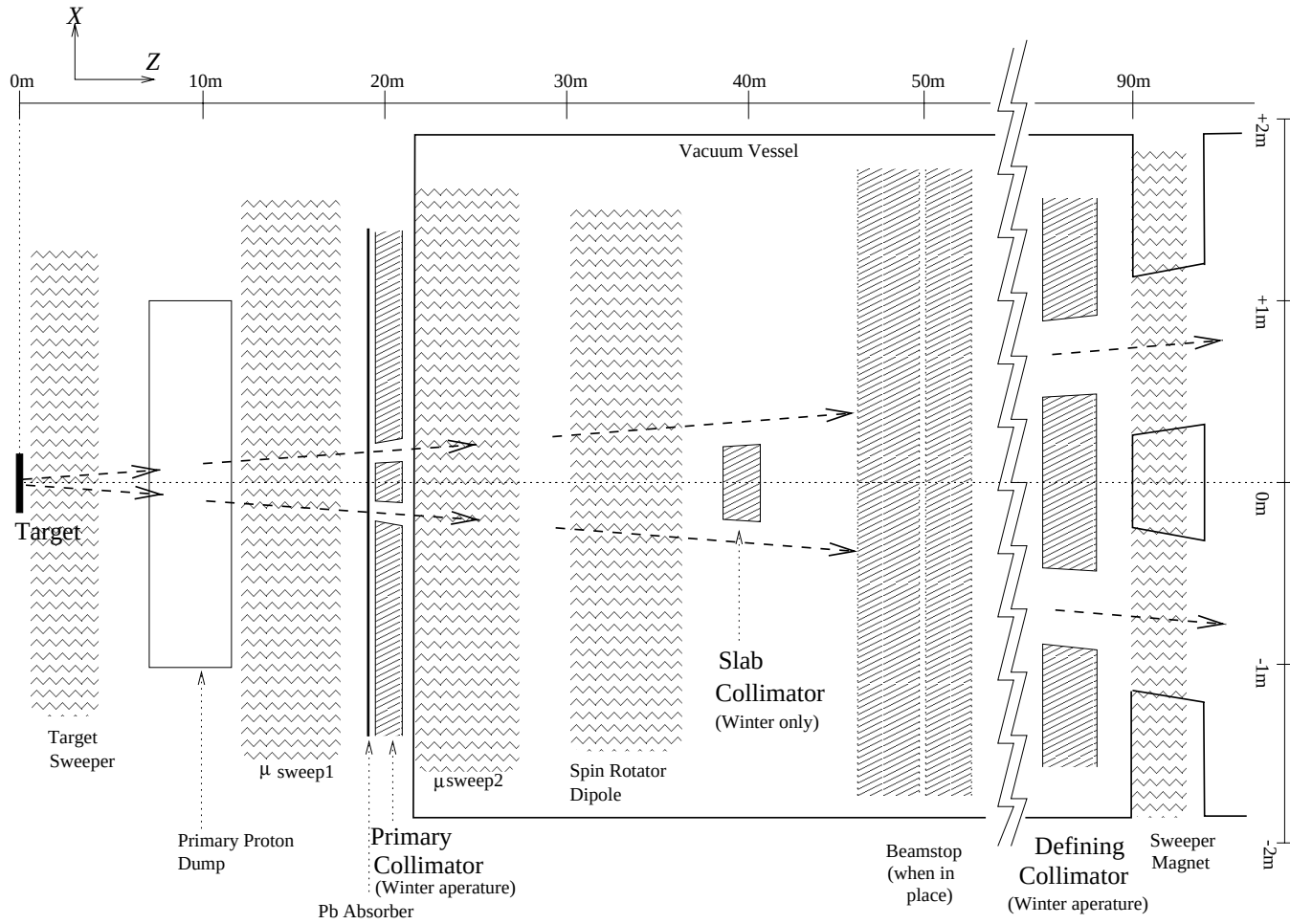
Figure 2.1: Secondary beam, plan view. X and Z scales are different. Dashed lines indicate nominal beam position. X positions of edges that do not impinge on the beams are represented arbitrarily. Elements which do not affect the beams in E799 are not included.
