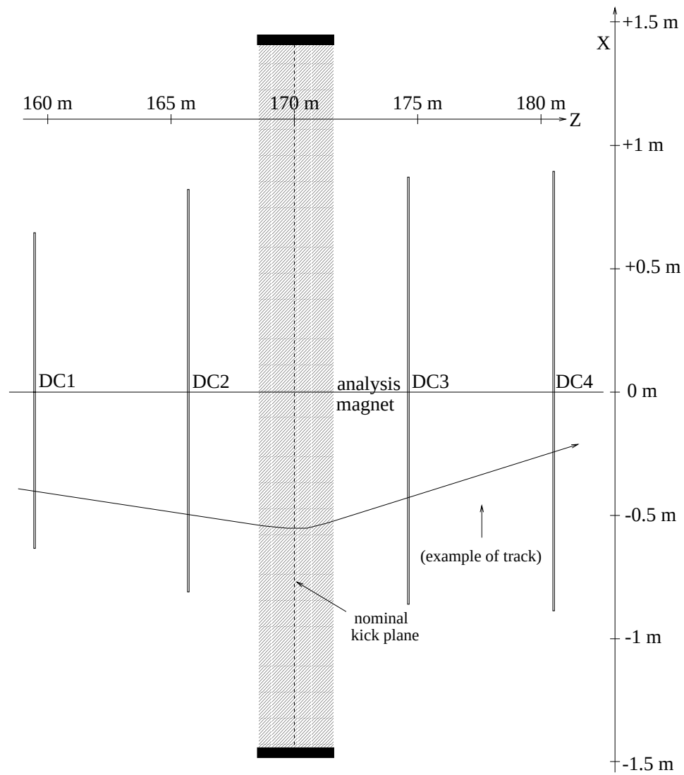
Figure 2.4: Spectrometer elements. X and Z scales differ. The plan view is shown, but the elevation view differs mainly in that no deflection occurs in Y in the magnet.
