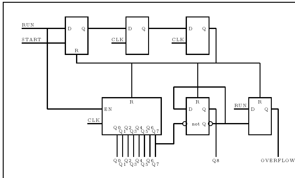
Figure 3.9: Block diagram of TDC circuit. Only one polarity is shown for differential ECL signals for simplicity.
