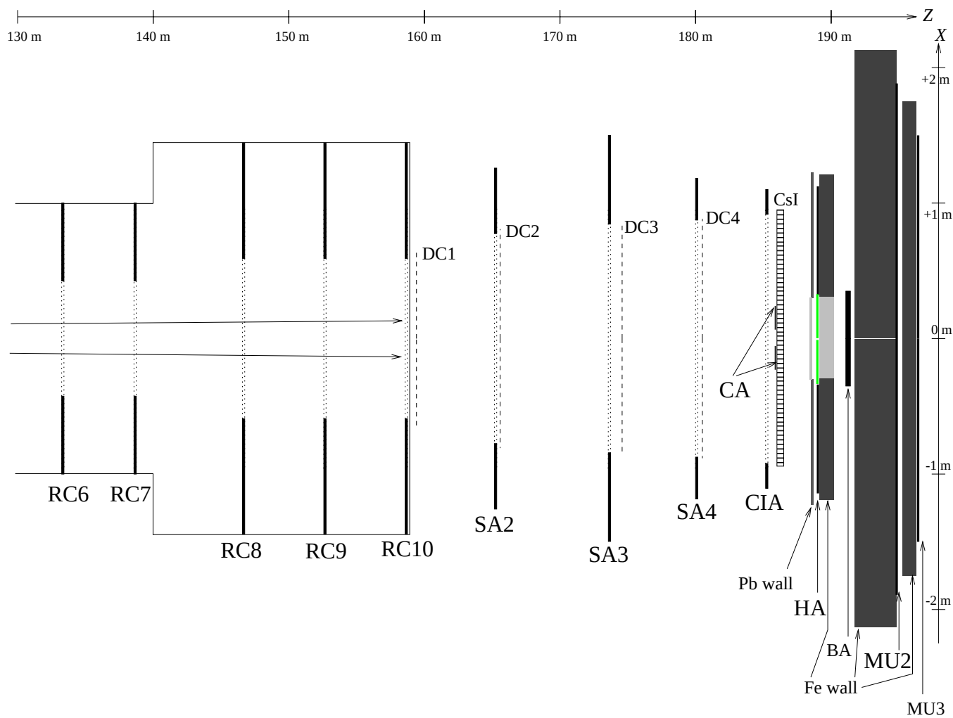
Figure 2.9: Veto detectors, plan view. X and Z scales differ.
