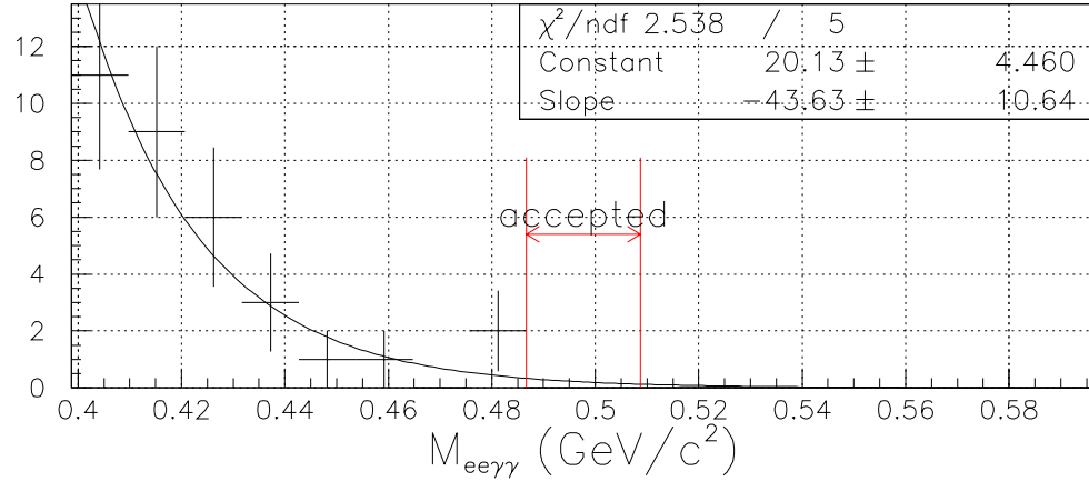
Figure 9.12: M_{ee\gamma\gamma} for simulated K \rightarrow \pi^0 \pi^0 \pi_{Dalitz}^0 , in \text{GeV}/c^2 . The MC sample size corresponds to \sim 31.6\% of the flux. All other cuts are applied.
