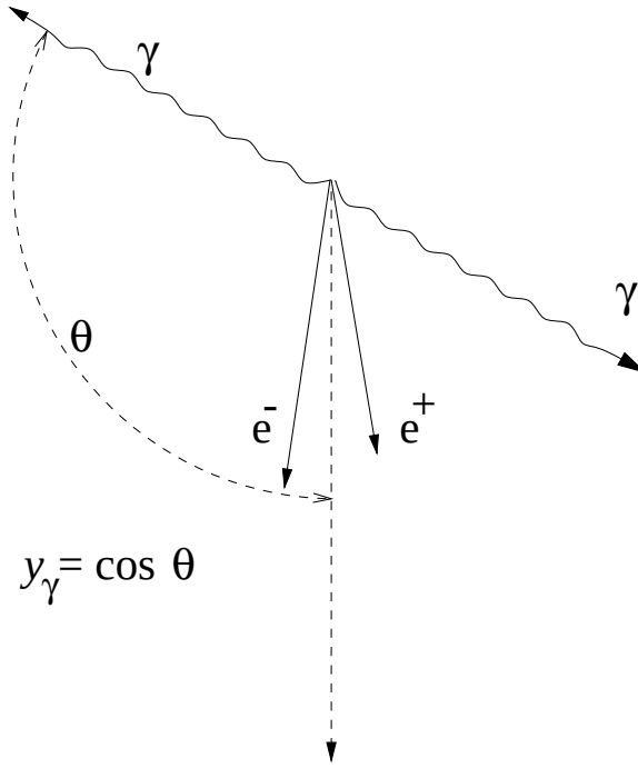
Figure 9.19: Phase-space variable y_\gamma .
