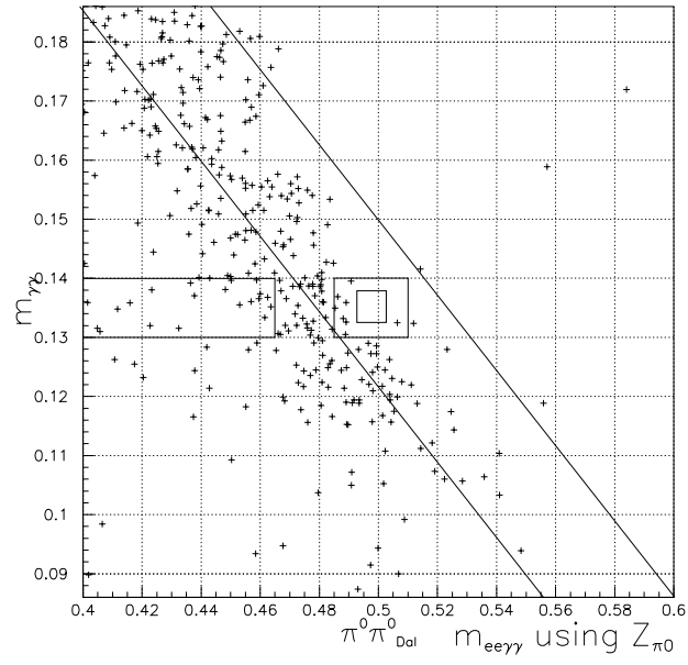
Figure 10.18: M_{\gamma\gamma} vs M_{ee\gamma\gamma} in GeV/c 2 , after all other cuts, for simulated K \rightarrow \pi^0 \pi^0_{Dalitz} .
