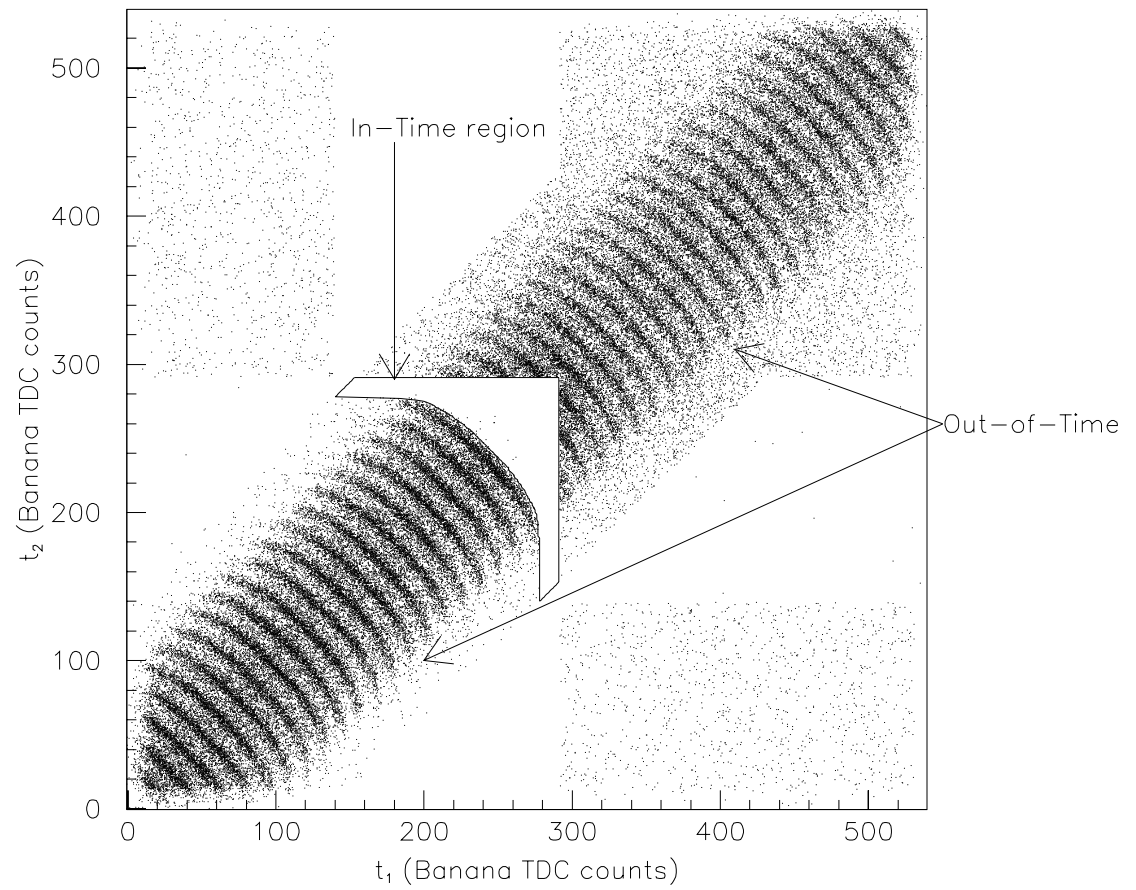
Figure 3.12: Banana t_1 vs. t_2 and in-time pair region boundary for isolated pairs rejected by Banana.
