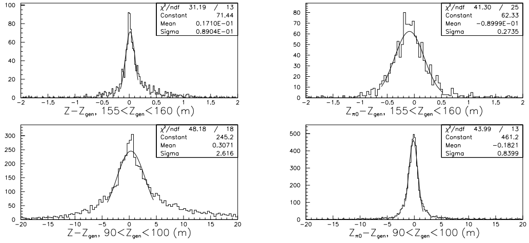
Figure 8.3: Decay-vertex-Z resolution in simulated K \rightarrow \pi^0 \pi^0_{Dalitz} . Reconstructed Z minus generated Z in a sample of MC events, near fiducial limits. (Left) Reconstructed vertex uses DC tracks, (Right) reconstructed vertex uses Z_{\pi^0} .
