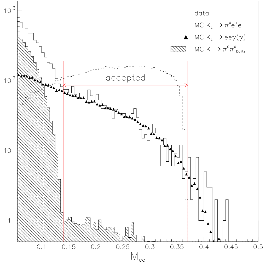
Figure 10.3: e^+e^- invariant mass, in \text{GeV}/c^2 , after general, M_{\pi+\pi-\gamma\gamma} , and TRD cuts. The K_L \rightarrow \pi^0 e^+ e^- distribution has arbitrary normalization.
