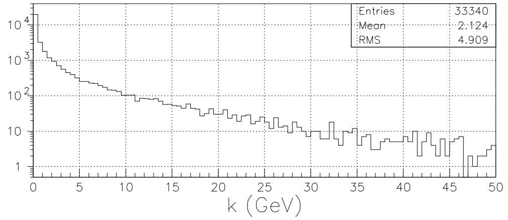
Figure 6.7: Energy of the bremsstrahlung photon.
