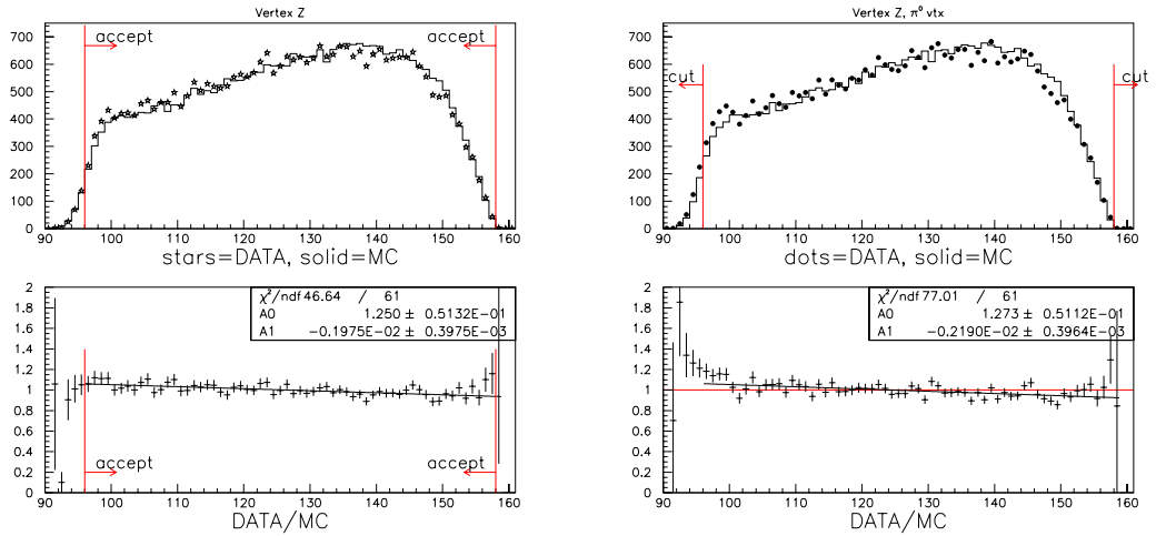
Figure 8.4: Vertex Z for all data and MC, after all other cuts. (Left) DC track vertex, (Right) Z_{\pi^0} .
