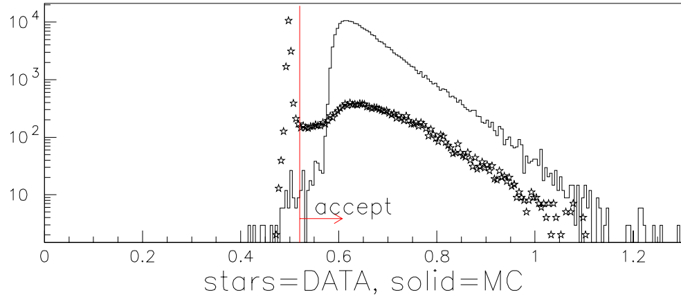
Figure 10.1: \pi^+ \pi^- \gamma \gamma invariant mass, in \text{GeV}/c^2 . Only general, non-TRD cuts are made. The solid line is simulated K_L \rightarrow \pi^0 e^+ e^- with arbitrary normalization.
