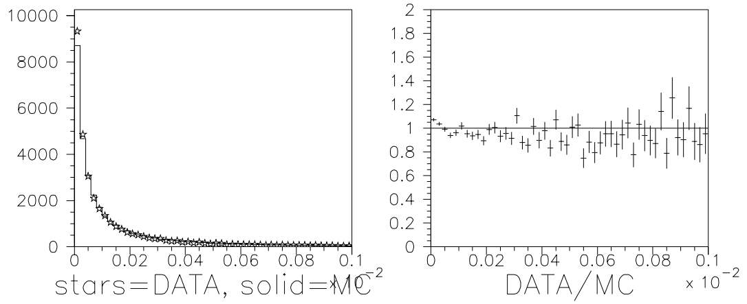
Figure 8.23: \vec{P}_T^2 (using Z_{\pi^0} ), in \text{GeV}^2/c^2 . All non- \vec{P}_T^2 cuts are made.
