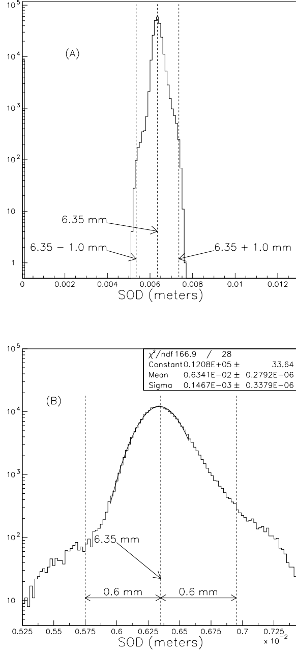
Figure 5.4: “Corrected” SOD. Y-view hits on tracks in K \rightarrow \pi^0 \pi^0_{Dalitz} decays. (B) is the peak in (A), with a gaussian fit.
