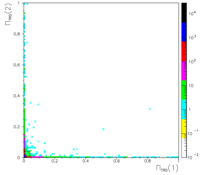
Figure 8.12: \Pi_{\text{TRD}} for each track in all data events, after all other cuts. The box indicates the cut.
