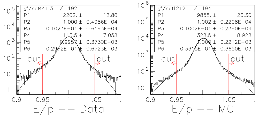
Figure 8.15: E/p for each track in Data and MC events, after all other cuts. The parameters are results of fitting to sum of two Gaussians.
