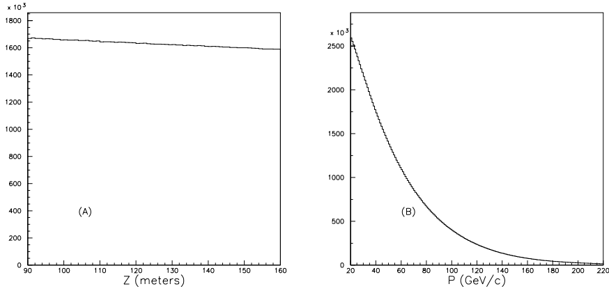
Figure 6.2: (A) Vertex Z and (B) momentum for a sample of generated K_L \rightarrow e^+e^-\gamma MC.
