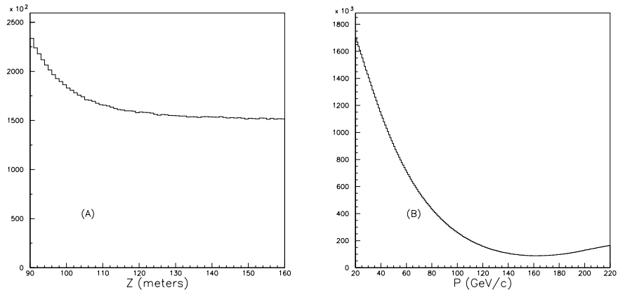
Figure 6.4: (A) Vertex Z and (B) momentum for a sample of generated K \rightarrow \pi^0 \pi^0_{Dalitz} MC.
