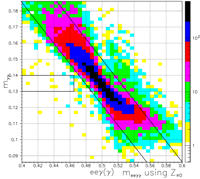
Figure 10.7: M_{\gamma\gamma} vs M_{ee\gamma\gamma} in \text{GeV}/c^2 , for simulated K_L \rightarrow e^+e^-\gamma(\gamma) , before kinematic cuts.
