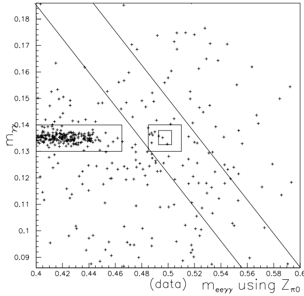
Figure 10.22: M_{\gamma\gamma} vs M_{ee\gamma\gamma} in \text{GeV}/c^2 , after all other cuts, for data failing \Pi_{\text{TRD}} cut. Thus all events shown here, including those in the box, are rejected.
