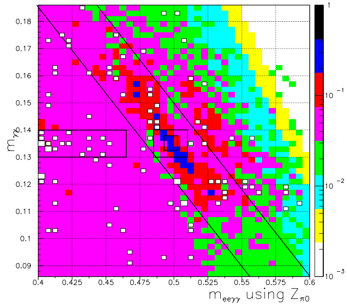
Figure 10.15: M_{\gamma\gamma} vs M_{ee\gamma\gamma} in \text{GeV}/c^2 , after all other cuts. The shaded boxes are the results of the background fit. The empty boxes are data, plotted on a linear Z scale. Data events inside the “box” are not shown.
