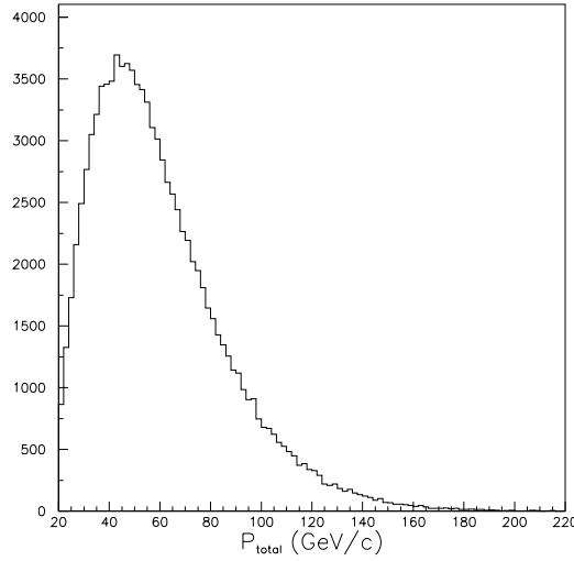
Figure 2.2: Kaon momenta, as reconstructed in K_L \rightarrow \pi^+\pi^-\pi^0 decays.
