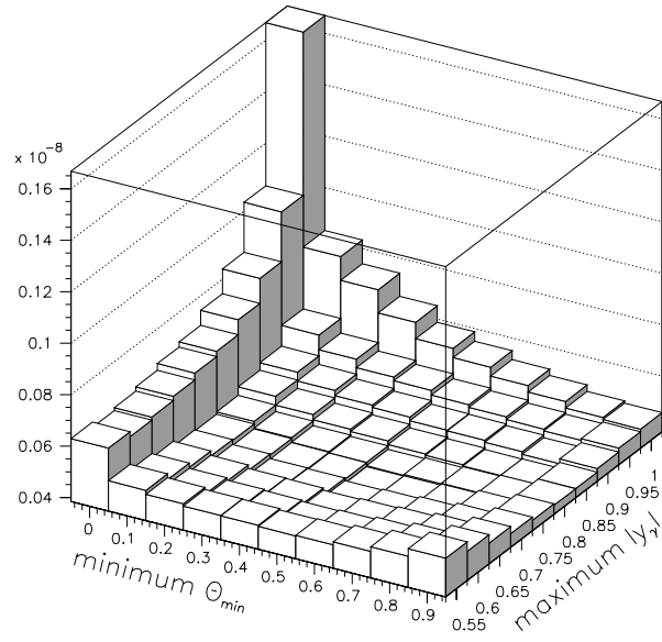
Figure 10.24: Estimated branching ratio limit, as function of cuts on \theta_{min} and |y_\gamma| , assuming vector model for K_L \rightarrow \pi^0 e^+ e^- .
