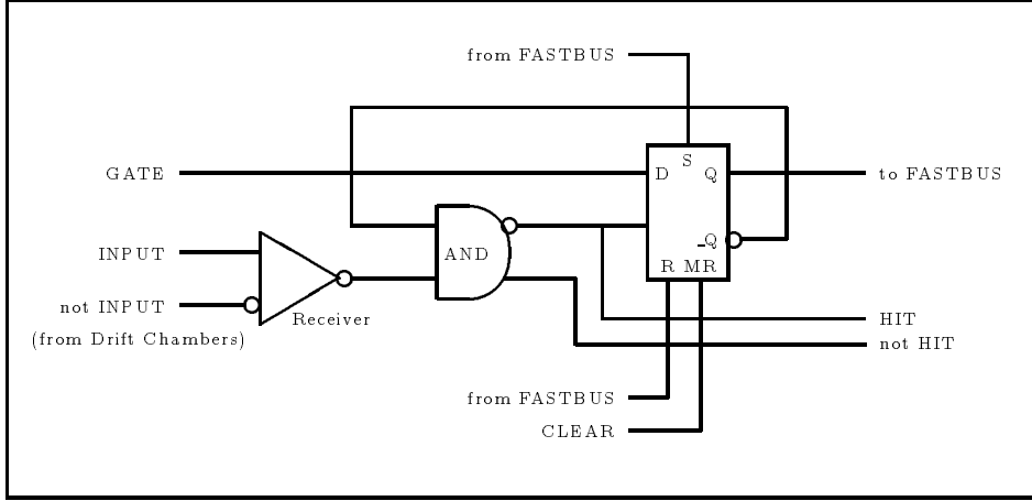
Figure 3.5: Block diagram of receiving/latching circuit
