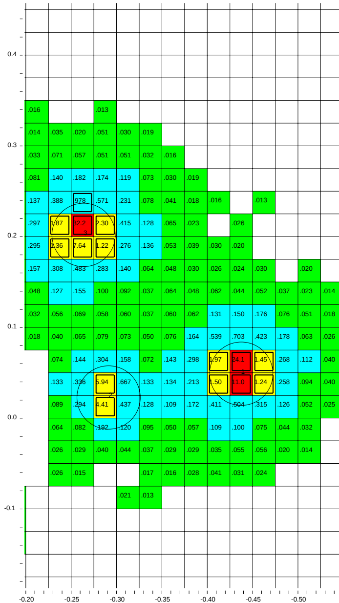
Figure 5.1: Event display of calorimeter. The circles are centered on found clusters. The dark squares are on channels with HCC bits set.
