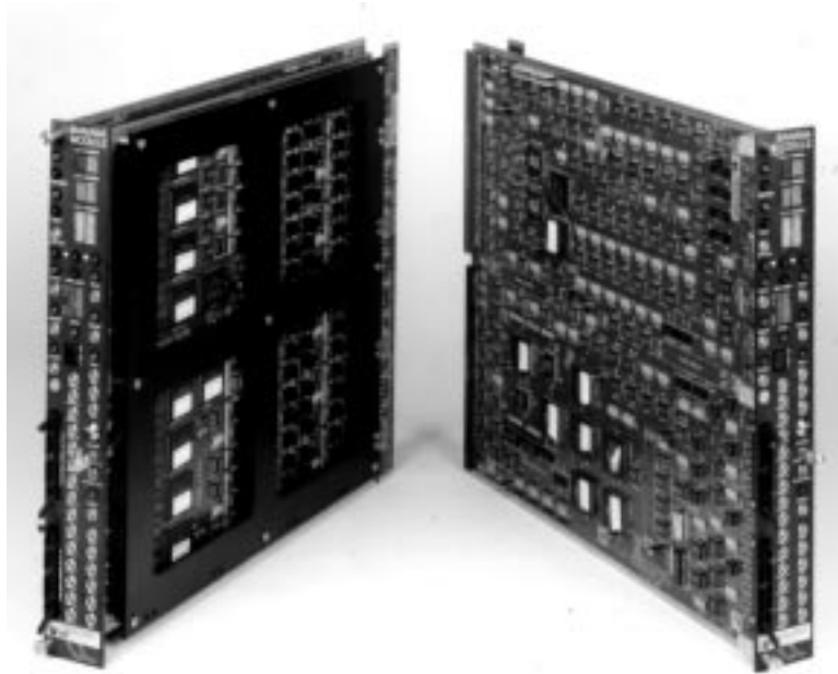
Figure 3.7: Photograph of Banana modules. In the left module, the hit logic and flash TDC chips are visible behind the stiffener plate. The right module shows chips for all other circuits.
