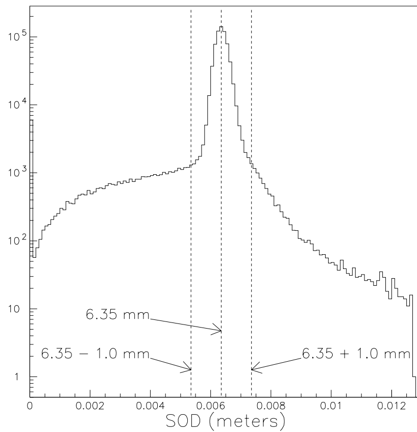
Figure 5.3: “Raw” SOD. Y-view hits on tracks in K \rightarrow \pi^0 \pi_{Dalitz}^0 decays. The entries at SOD=0 are isolated hits.
