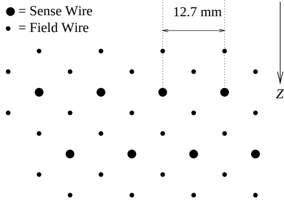
Figure 2.5: DC plane pair schematic. Short segment of plane pair, showing upstream and downstream planes, and hexagonal geometry of wire cells.
