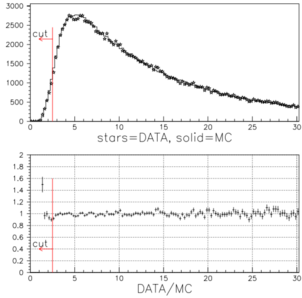
Figure 8.9: All calorimeter cluster energies (GeV). All other cuts are made, except for ETOT verification.
