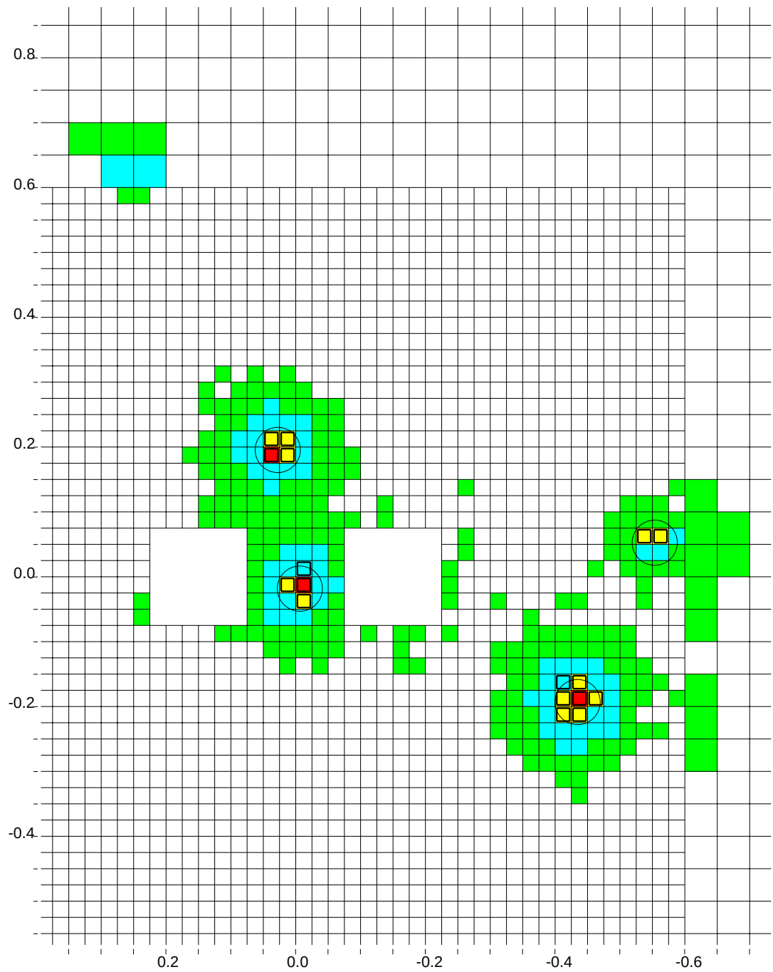
Figure 3.1: Example of energy in calorimeter. The shading indicates energy deposited in that crystal, in steps of 0.01–0.1 GeV, 0.1–1.0 GeV, 1.0–10.0 GeV, and more than 10.0 GeV. The circles indicate where the HCC algorithm found clusters.
