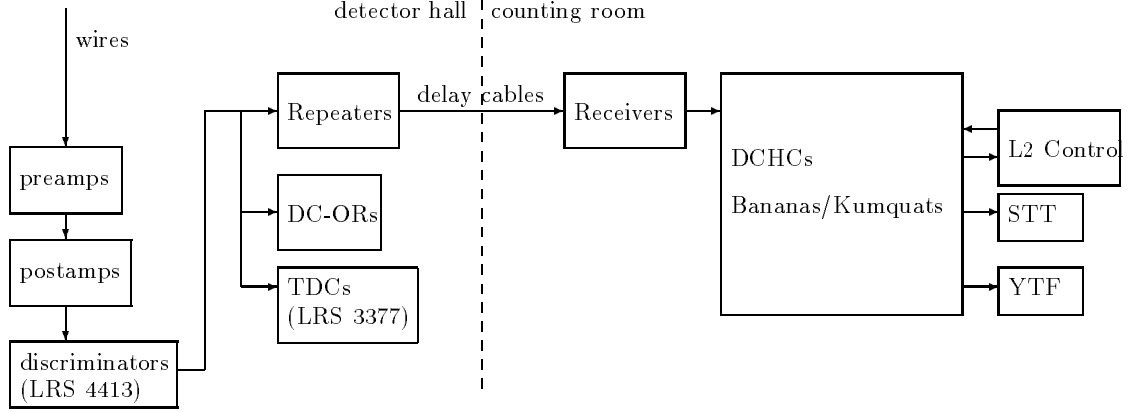
Figure 3.2: DCHC overview.
