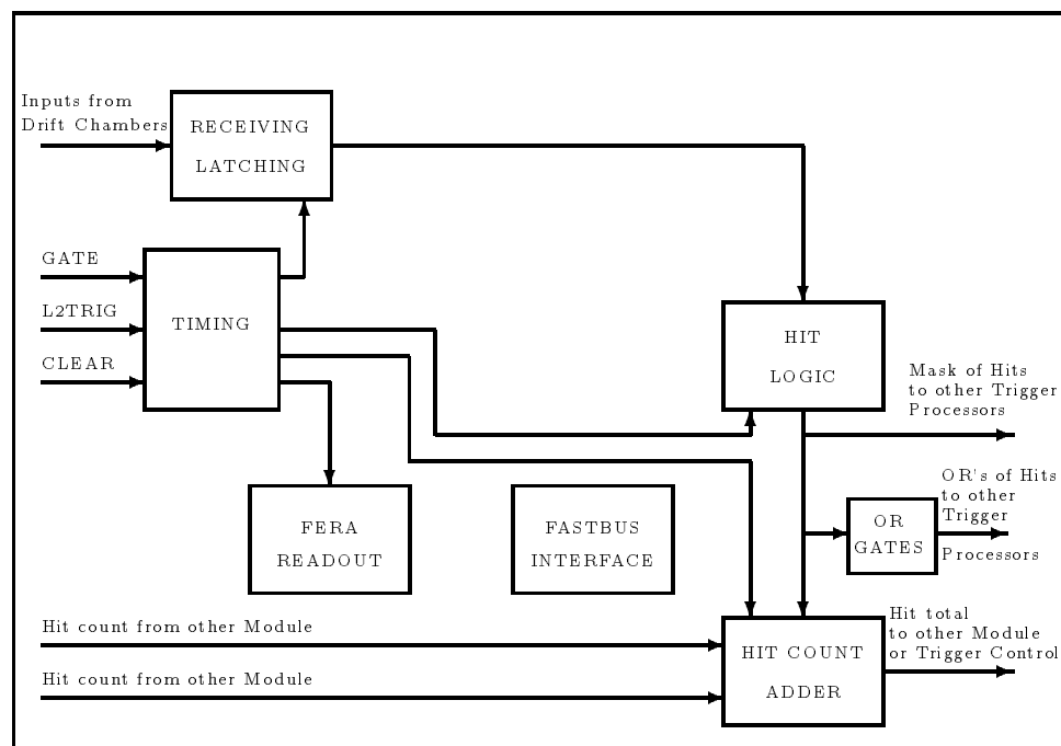
Figure 3.4: Block diagram of Kumquat module.
