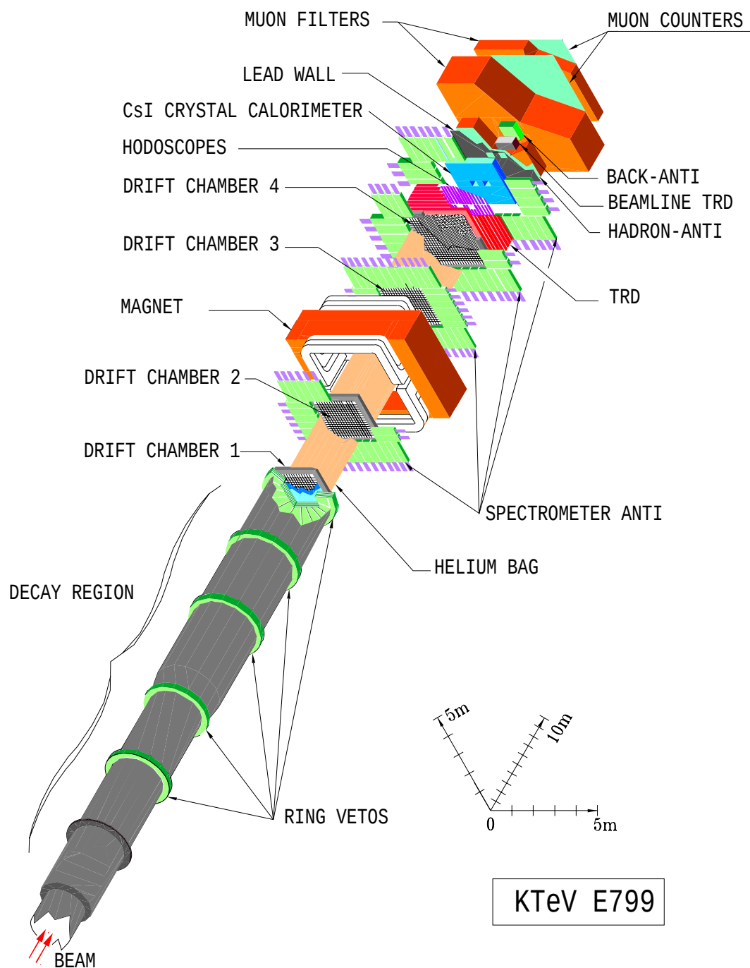
Figure 2.3: KTeV detector. X and Y scales are blown up, relative to Z scale.
