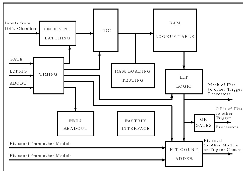
Figure 3.8: Block diagram of Banana module.
