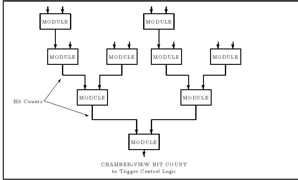
Figure 3.13: Structure of DCHC adder tree.
