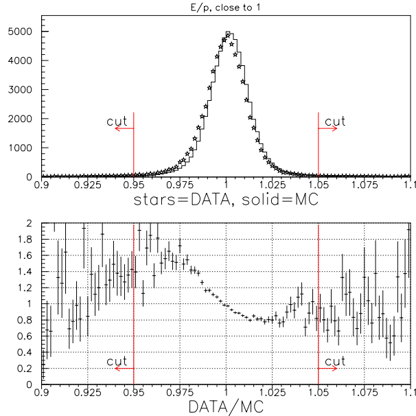
Figure 8.13: E/p for each track in Data and MC events, after all other cuts.
