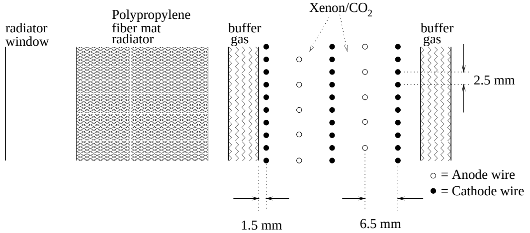
Figure 2.7: TRD cross section, plan view. Scale is approximate, except for wire spacing and as noted.
