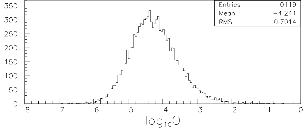
Figure 6.6: Log of the bremsstrahlung opening angle \theta .
