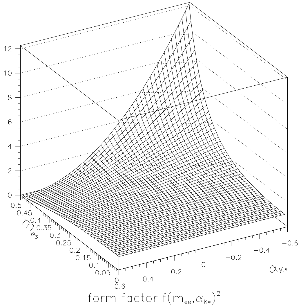
Figure 9.13: Square of BMS form factor, vs \alpha_{K^*} and M_{ee} in \text{GeV}/c^2 . Note that equation 1.3 gives f(x) , while f(M_{ee}, \alpha_{K^*})^2 is plotted here.
