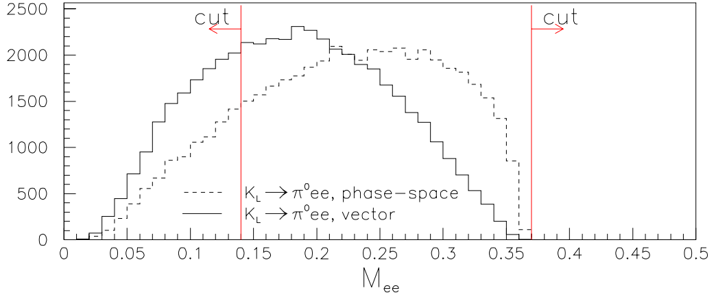
Figure 10.25: e^+e^- mass, in \text{GeV}/c^2 , for K_L \rightarrow \pi^0 e^+ e^- MC samples after all other cuts.
