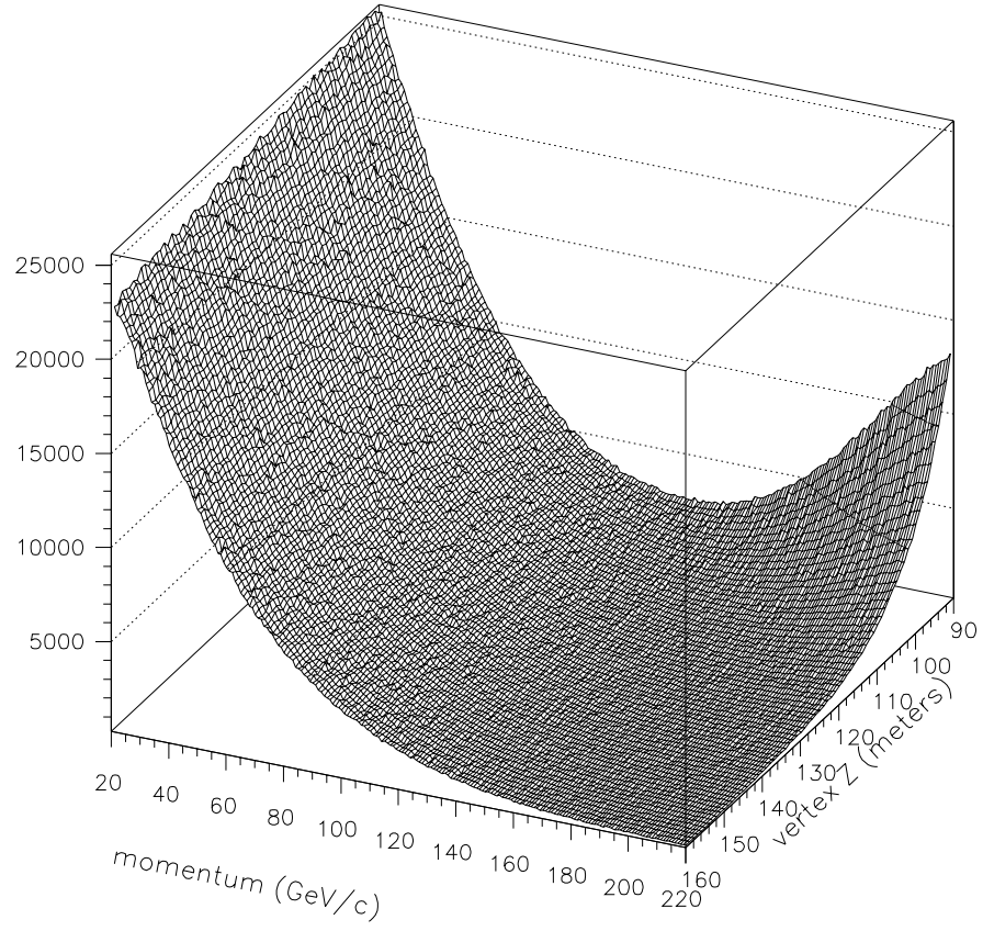
Figure 6.3: P vs. Z for a sample of generated K \rightarrow \pi^0 \pi^0_{Dalitz} MC.
