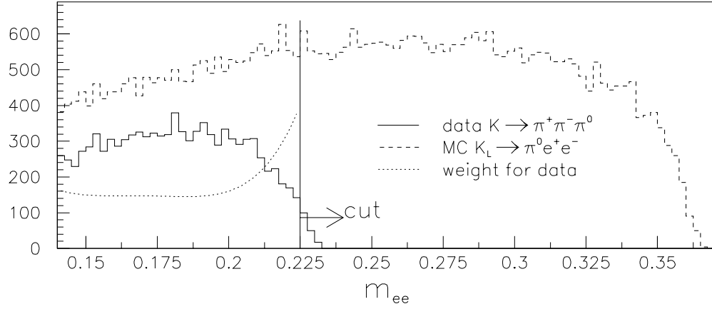
Figure 10.16: e^+e^- invariant mass, in (\text{GeV}/c^2)^2 . All non- M_{\gamma\gamma} cuts have been applied to MC. The M_{ee} cut shown is only used for the M_{\gamma\gamma} resolution study.
