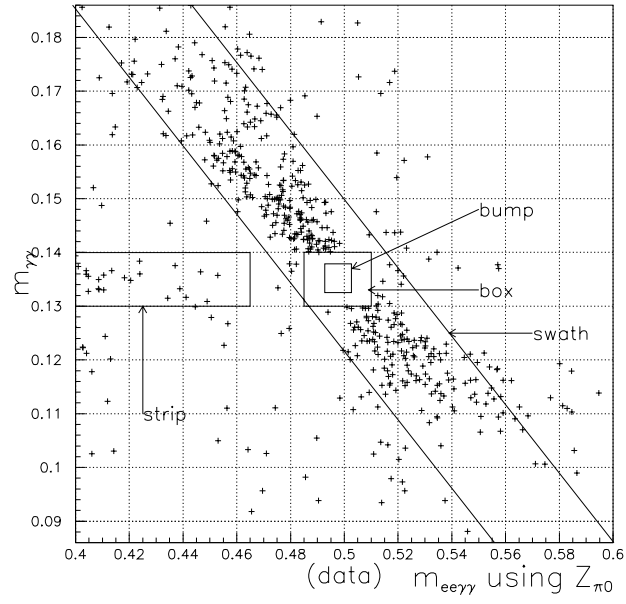
Figure 10.6: M_{\gamma\gamma} vs M_{e\bar{e}\gamma\gamma} in \text{GeV}/c^2 , for data, before kinematic cuts.
