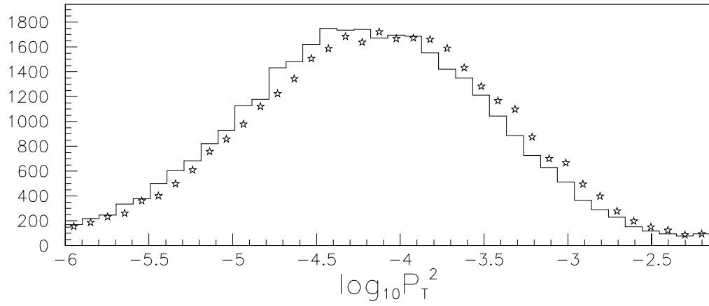
Figure 8.22: \log_{10} \vec{P}_T^2 using track-vertex Z (Dots) and Z_{\pi^0} (Line), measuring \vec{P}_T^2 in (\text{GeV}/c)^2 . All other cuts are made.
