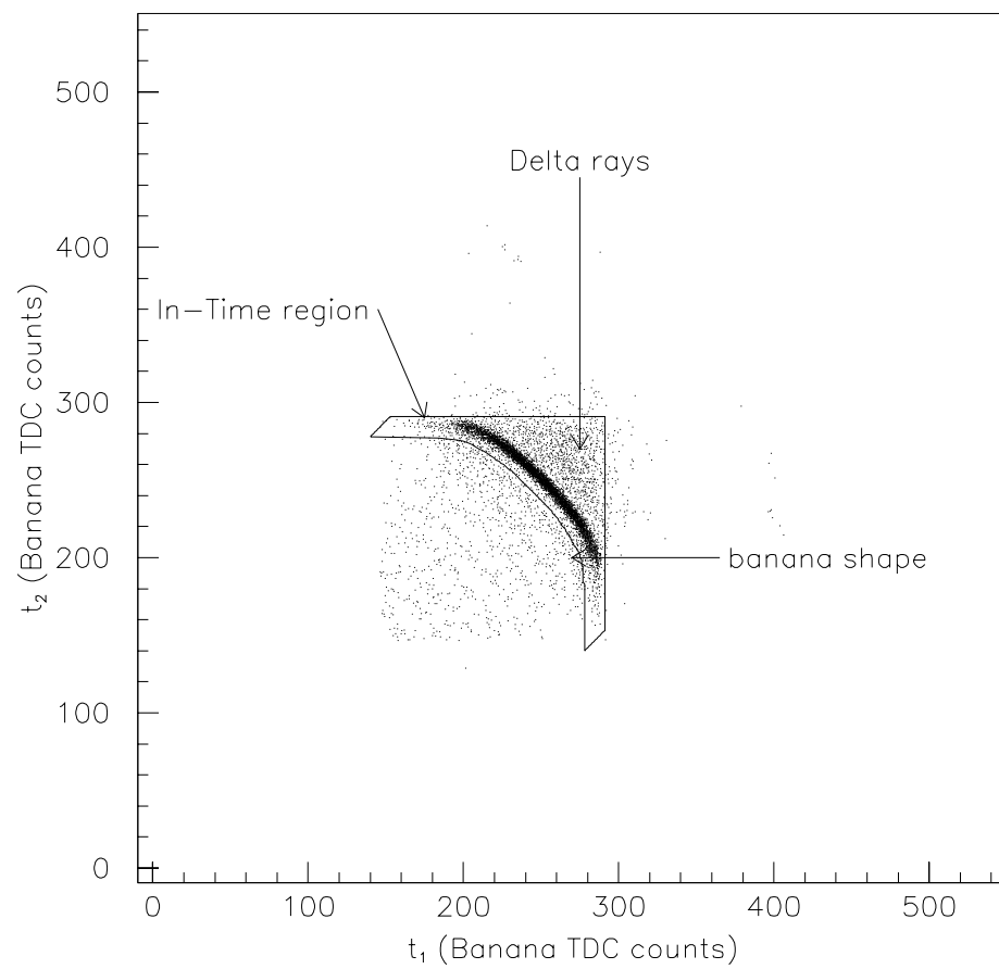
Figure 3.11: Banana t_1 vs. t_2 and in-time pair region boundary for hits on tracks.
