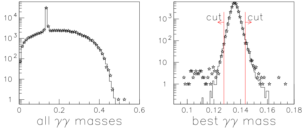
Figure 8.18: Two-photon invariant mass, in \text{GeV}/c^2 , for all pairings (Left) and for best pairing (Right). Dots are data and solid line is MC. All other cuts are made.
