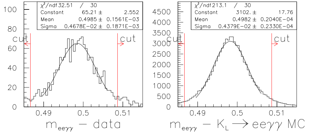
Figure 9.9: e^+e^-\gamma\gamma invariant mass in \text{GeV}/c^2 after all other cuts, for data (Left) and simulated K_L \rightarrow e^+e^-\gamma\gamma (Right).
