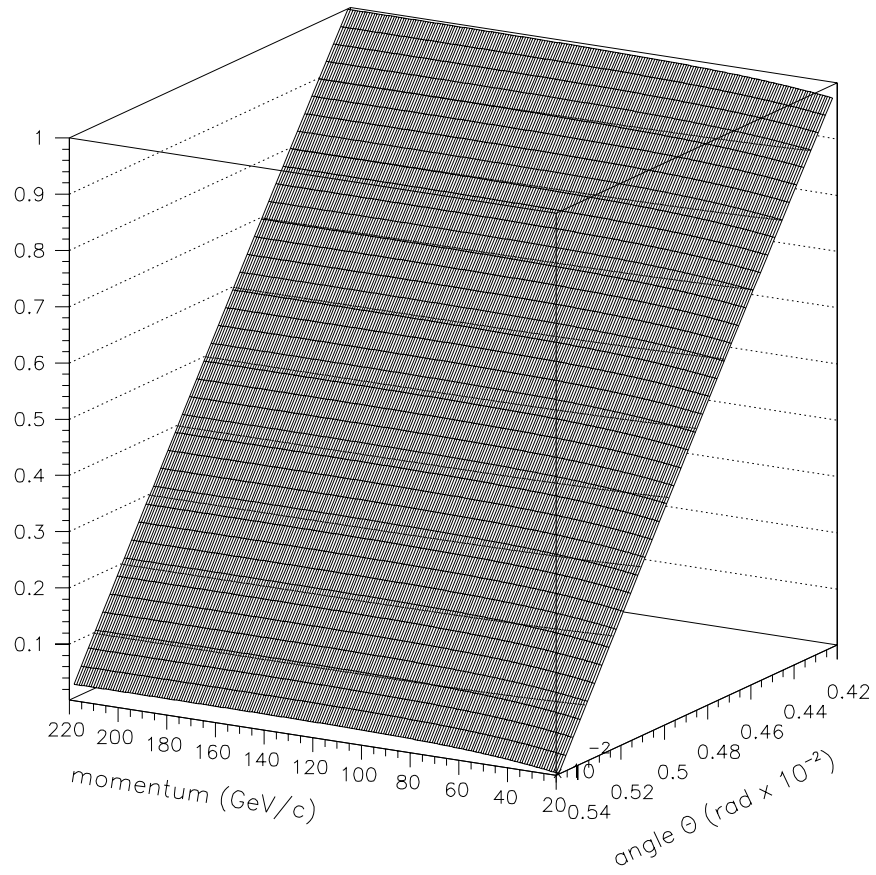
Figure 6.1: Momentum vs. vertical angle at target. As mentioned in chapter 2, the proton beam angle is -0.48 \times 10^{-2} rad. K^0 and \bar{K}^0 distributions are similar and are averaged here.
