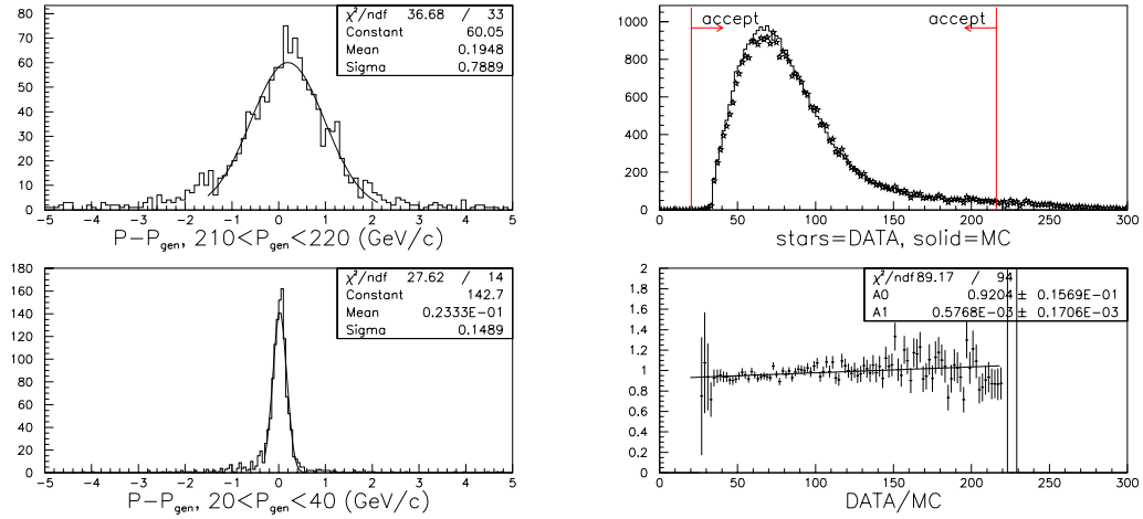
Figure 8.2: (Left) Momentum resolution in simulated K \rightarrow \pi^0 \pi^0_{Dalitz} . Reconstructed total momentum minus generated total momentum in a sample of MC events, near fiducial limits. (Right) Reconstructed momentum for all data and MC, after all other cuts.
