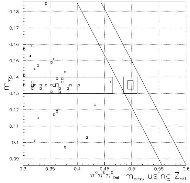
Figure 10.19: M_{\gamma\gamma} vs M_{ee\gamma\gamma} in GeV/c 2 , after all other cuts, for simulated K \rightarrow \pi^0 \pi^0 \pi^0_{Dalitz} . Note that the M_{ee\gamma\gamma} scale is expanded in this plot.
