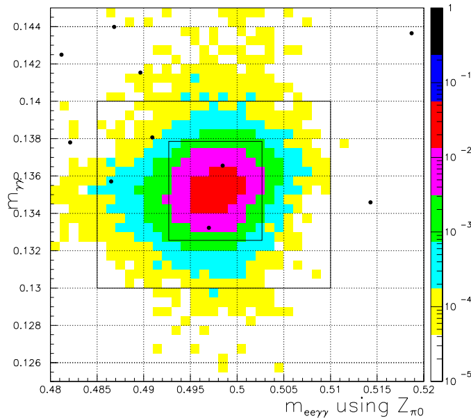
Figure 10.23: M_{\gamma\gamma} vs M_{ee\gamma\gamma} in \text{GeV}/c^2 , after all other cuts. The box is open. The shaded bins are K_L \rightarrow \pi^0 e^+ e^- MC, normalized to 1.
