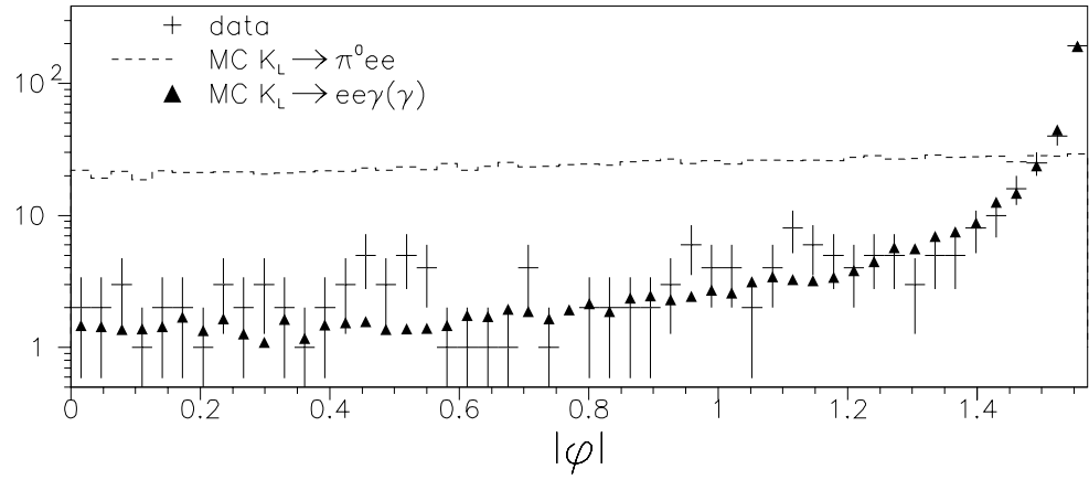
Figure 10.13: Absolute value of |\phi| for events in swath but outside box. Simulated K_L \rightarrow \pi^0 e^+ e^- events are from inside box, and have arbitrary normalization.
