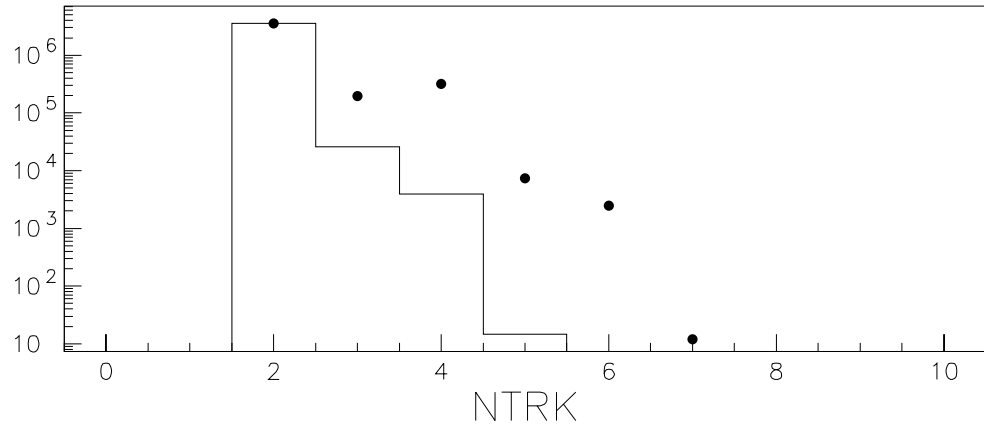
Figure 8.1: Number of tracks in K \rightarrow \pi^0 \pi^0_{Dalitz} reconstruction. Dots are data and line is MC, normalized to data. No cut has limited the number of clusters yet.
