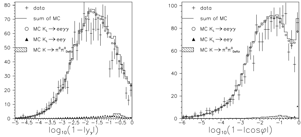
Figure 9.20: Phase-space angles y_\gamma and \phi . All cuts are made.
