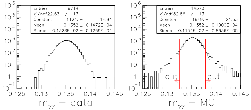
Figure 10.17: \gamma\gamma invariant mass, in (\text{GeV}/c^2)^2 , for K_L \rightarrow \pi^+\pi^-\pi^0 data (Left) and simulated K_L \rightarrow \pi^0 e^+ e^- (Right).
