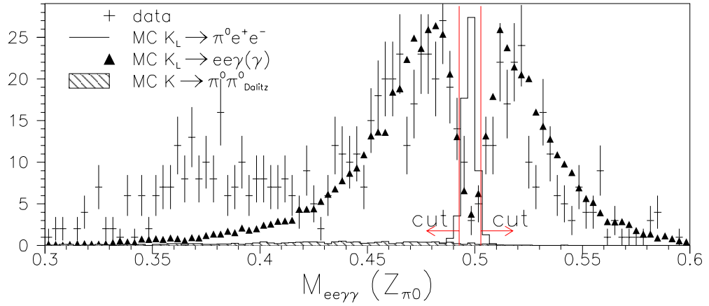
Figure 10.5: e^+ e^- \gamma \gamma invariant mass, using Z_{\pi^0} , in (\text{GeV}/c^2)^2 , after general, M_{\pi^+ \pi^- \gamma \gamma} , TRD, M_{ee} , and \vec{P}_T^2 cuts. The K_L \rightarrow \pi^0 e^+ e^- distribution has arbitrary normalization. The fit “box” has been excluded in the data and K_L \rightarrow e^+ e^- \gamma(\gamma) samples. The excess data below 420 \text{ MeV}/c^2 are mostly from K_{e4} decays.
