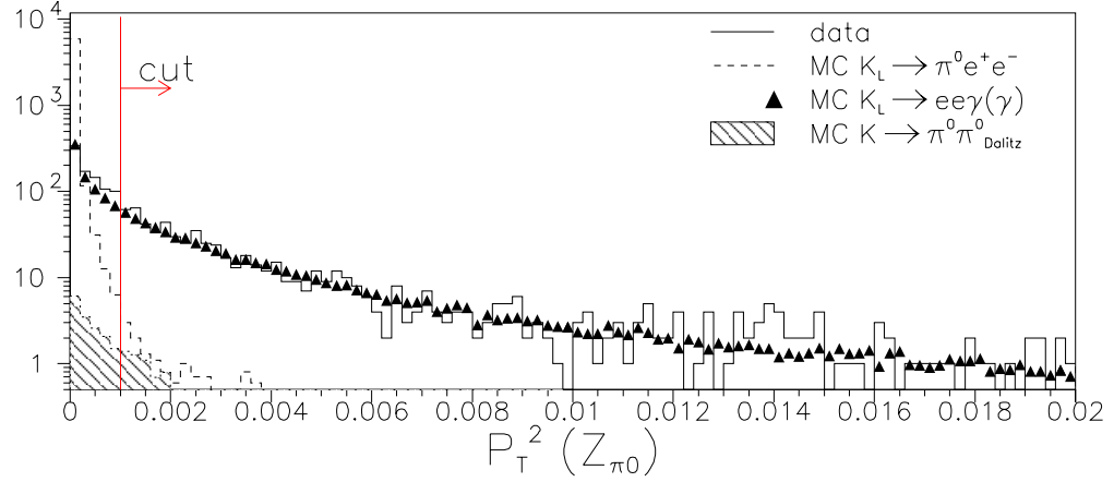
Figure 10.4: Transverse momentum, \vec{P}_T^2 , using Z_{\pi^0} , in (\text{GeV}/c^2)^2 , after general, M_{\pi^+ \pi^- \gamma \gamma} , TRD, and M_{ee} cuts. The K_L \rightarrow \pi^0 e^+ e^- distribution has arbitrary normalization.
