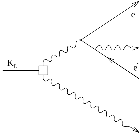
Figure 1.3: K_L \rightarrow e^+e^-\gamma\gamma . The other tree-level Feynmann diagrams have the radiated photon coming from the positron and exchange the radiated and direct photons.
