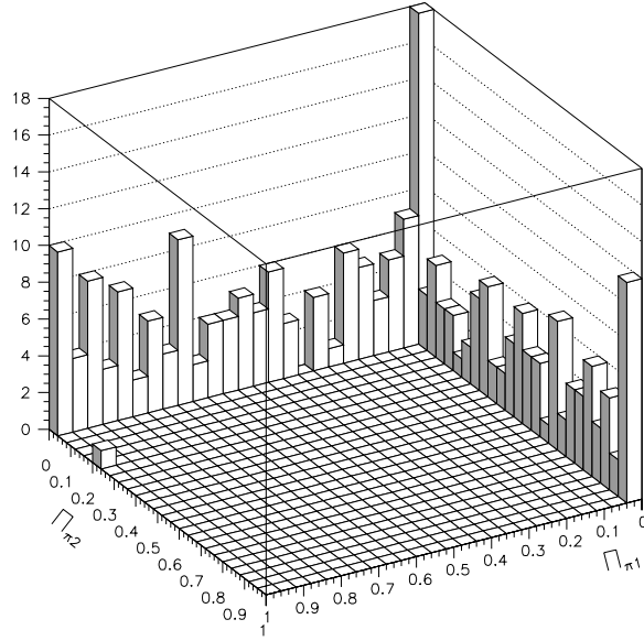
Figure 10.20: TRD \Pi_{\text{TRD}} for data events with 130 < M_{\gamma\gamma} < 140 \text{ MeV}/c^2 and 400 < M_{e\gamma\gamma} < 465 \text{ MeV}/c^2 , after all other cuts. The only region accepted by the TRD cuts is the bin that has 18 events.
