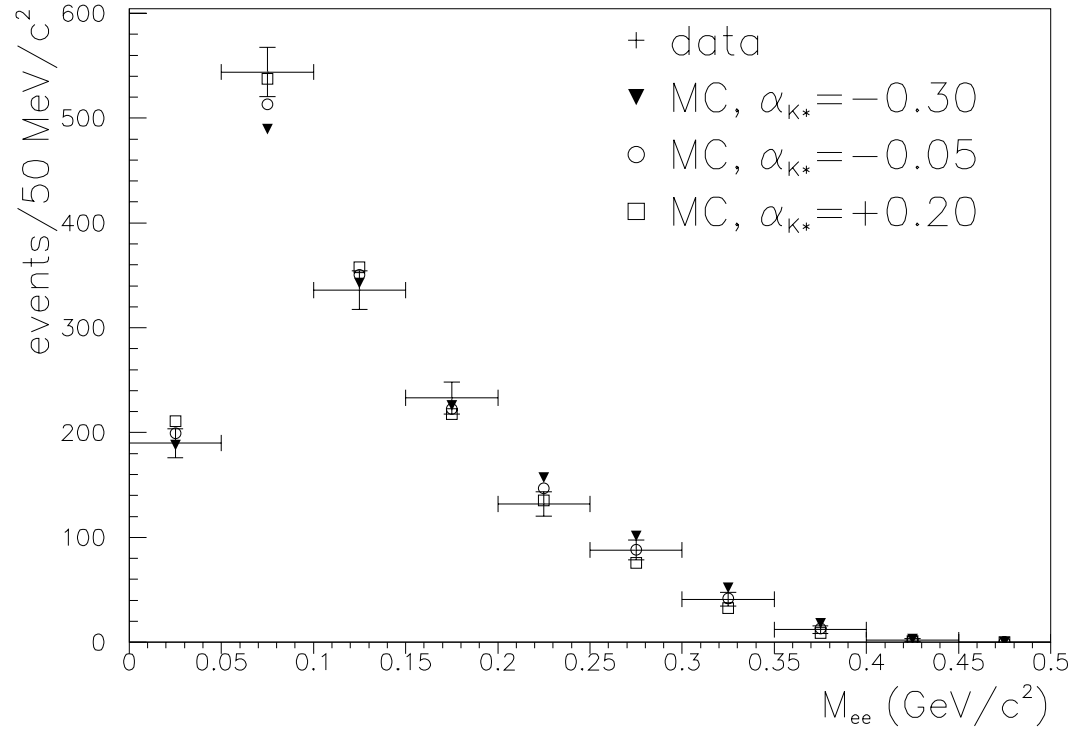
Figure 9.15: e^+e^- invariant mass for data and MC with several \alpha_{K^*} , in \text{GeV}/c^2 . The error bars on the MC levels are smaller than the symbols at the levels.
