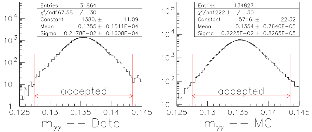
Figure 8.19: Two-photon invariant mass, in \text{GeV}/c^2 , data (Left) and simulated K \rightarrow \pi^0 \pi^0_{\text{Dalitz}} (Right). All other cuts are made.
