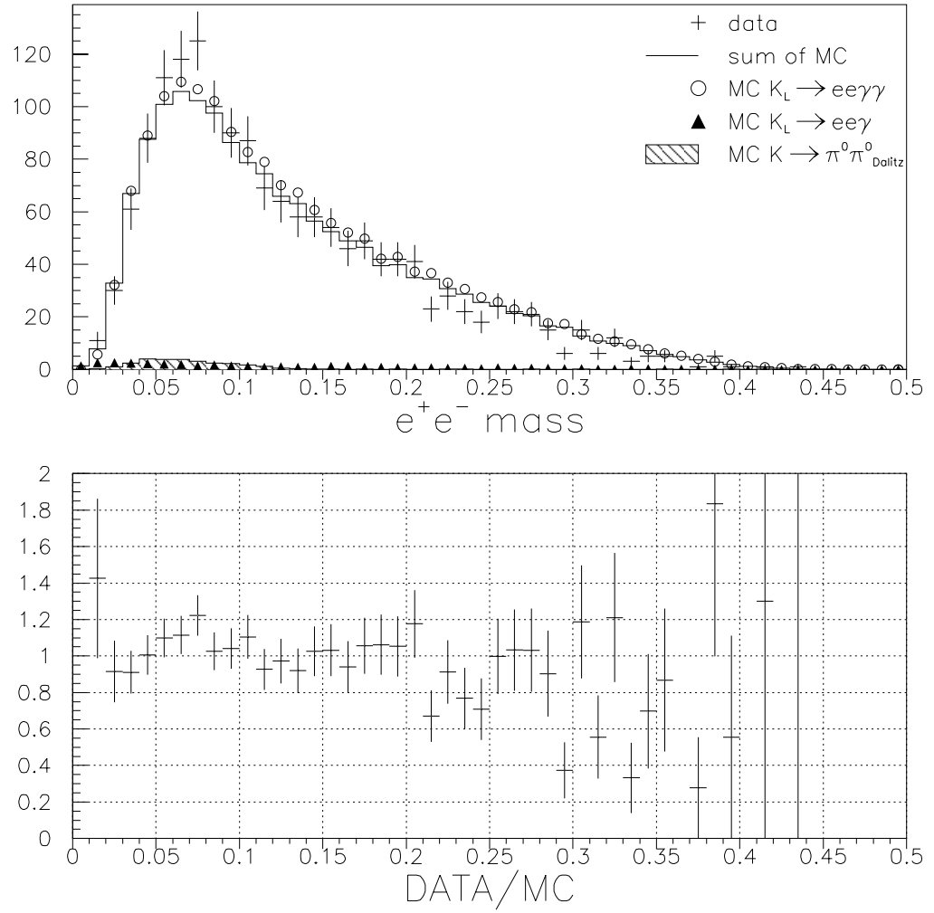
Figure 9.14: e^+e^- invariant mass, in \text{GeV}/c^2 . Note that the summed MC is normalized to have the same area as the data, while the other MC distributions are normalized by flux and BR. The data/MC ratio plot uses summed MC. All cuts are applied.
