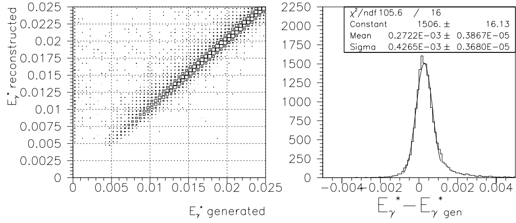
Figure 9.2: E_{\gamma}^* as generated in simulation and as reconstructed, for K_L \rightarrow e^+e^-\gamma(\gamma) MC, in GeV. (Right) Difference between E_{\gamma}^* s when both are less than 25 MeV. All other cuts are made.
