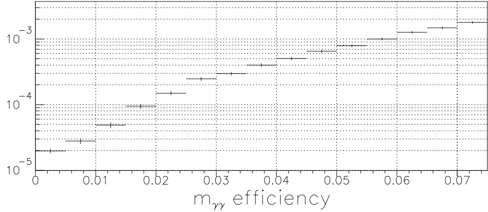
Figure 9.6: Efficiency vs. M_{\gamma\gamma} , in \text{GeV}/c^2 . All other cuts are made.
