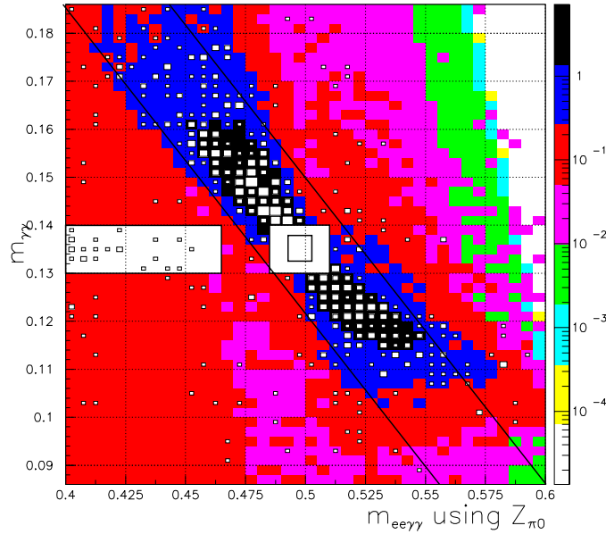
Figure 10.8: M_{\gamma\gamma} vs M_{ee\gamma\gamma} in \text{GeV}/c^2 , before kinematic cuts. The shaded boxes are the results of the background fit. The empty boxes are data, plotted on a linear Z scale. Data events inside the “box” are not shown.
