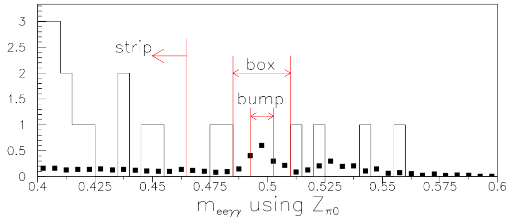
Figure 10.21: e^+e^-\gamma\gamma invariant mass after all other cuts, in \text{GeV}/c^2 . The squares are the background fit, which excludes the strip, and the fit error bars are not shown. The fit and the data use the same 5 \text{ MeV}/c^2 bins. No data from inside the box are shown. The M_{\gamma\gamma} cut is applied.
