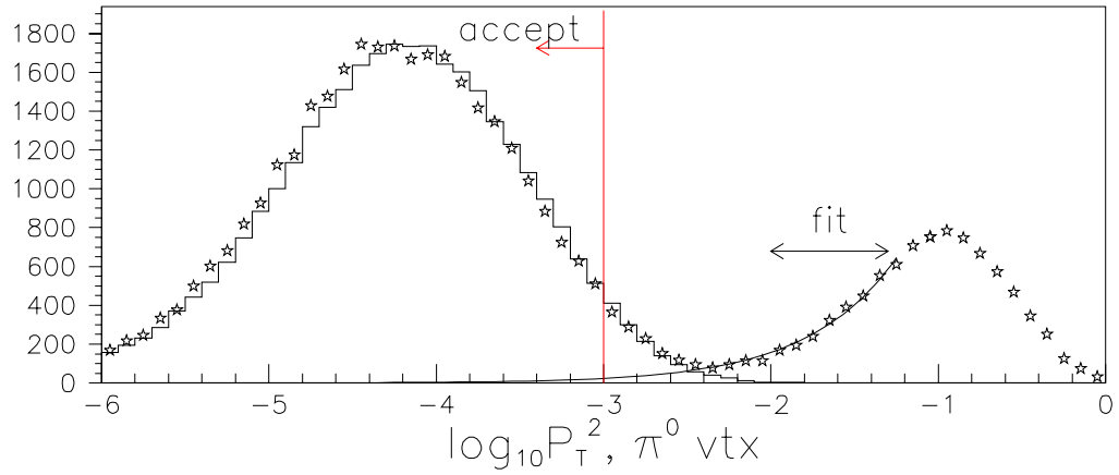
Figure 8.24: \log_{10} \vec{P}_T^2 (using Z_{\pi^0} ), where the dots are data. The smooth line is a fit to the data. The MC is shown as a histogram, normalized to make the peak heights match below the cut. \vec{P}_T^2 is measured in (\text{GeV}/c)^2 . All non- \vec{P}_T^2 cuts are made.
