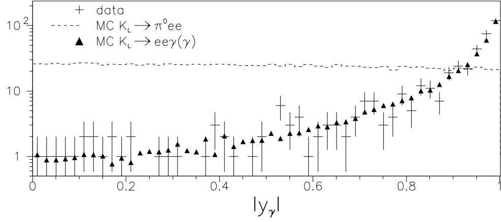
Figure 10.12: Absolute value of y_\gamma for events in swath but outside box. Simulated K_L \rightarrow \pi^0 e^+ e^- events are from inside box, and have arbitrary normalization.
