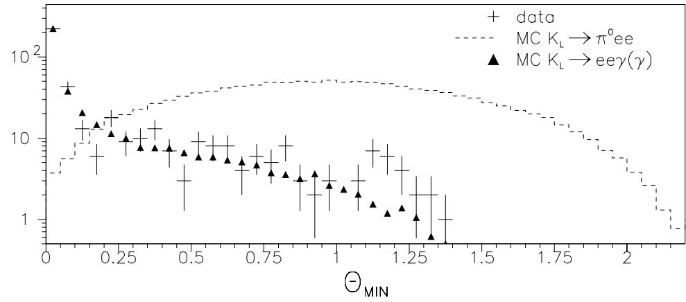
Figure 10.11: \theta_{min} for events in swath but outside box. Simulated K_L \rightarrow \pi^0 e^+ e^- events are from inside box, and have arbitrary normalization.
