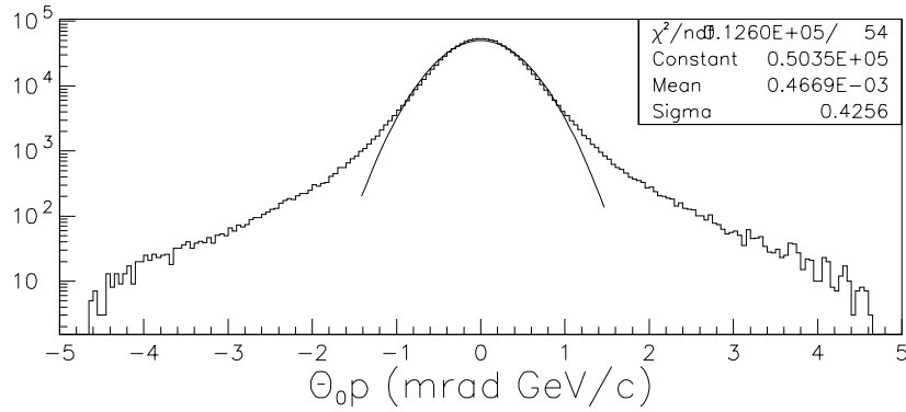
Figure 6.5: Momentum times multiple-scattering angle projected onto plane, for e^+ and e^- at vacuum window. The fit to a gaussian goes from -1.4 mrad GeV/c to +1.4 mrad GeV/c, a region which includes 98% of the distribution.
