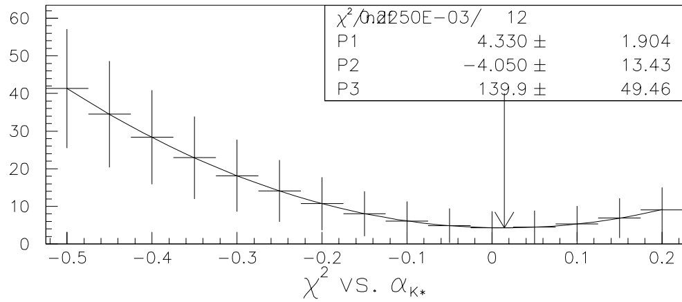
Figure 9.16: \chi^2 for data fit to summed MC with varied \alpha_{K^*} . The arrow indicates the minimum of the fit at \alpha_{K^*} = +0.0145 and \chi^2 = 4.30 .
