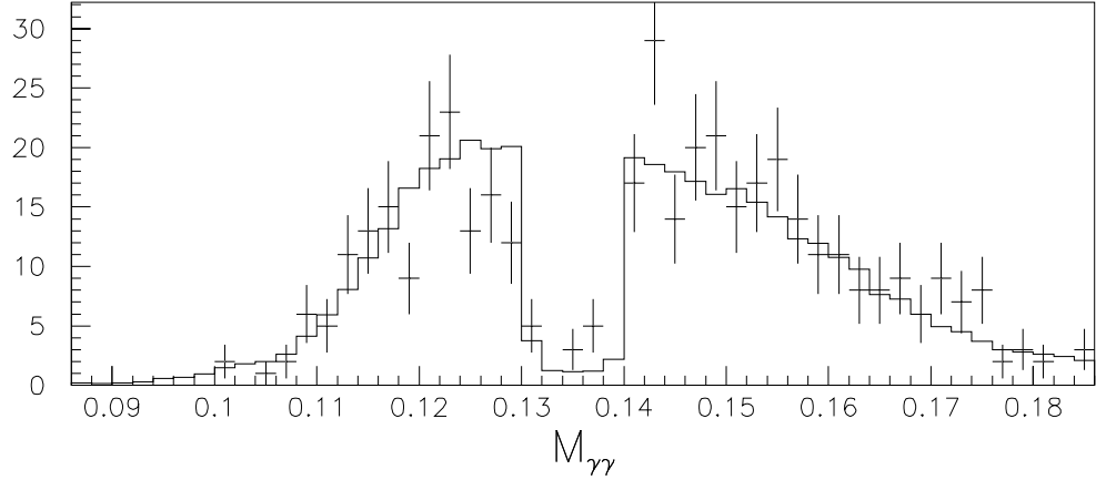
Figure 10.9: M_{\gamma\gamma} in \text{GeV}/c^2 , before kinematic cuts, in M_{\gamma\gamma} , M_{ee\gamma\gamma} “swath.” Crosses are data and solid line is fit.
