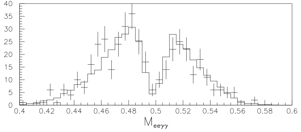
Figure 10.10: M_{ee\gamma\gamma} in \text{GeV}/c^2 , before kinematic cuts, in M_{\gamma\gamma} , M_{ee\gamma\gamma} “swath.” Crosses are data and solid line is fit.
