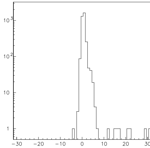
Figure 3.10: Banana TDC accuracy. Measured Banana TDC time minus LeCroy 3377 TDC time, in units of Banana TDC counts (1.6 ns), for a single channel.
