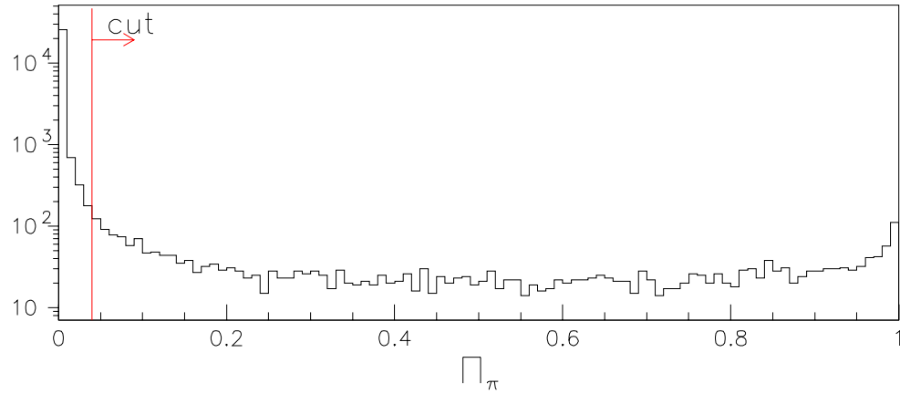
Figure 10.2: TRD \Pi_{\text{TRD}} for both tracks in data events.
