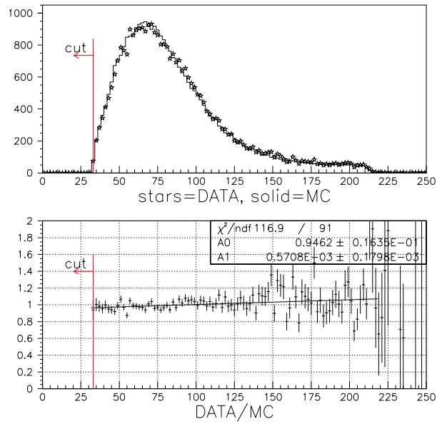
Figure 8.7: Total calorimeter energy (GeV), for ETOT verification. All other cuts are made, except for total momentum cut.
