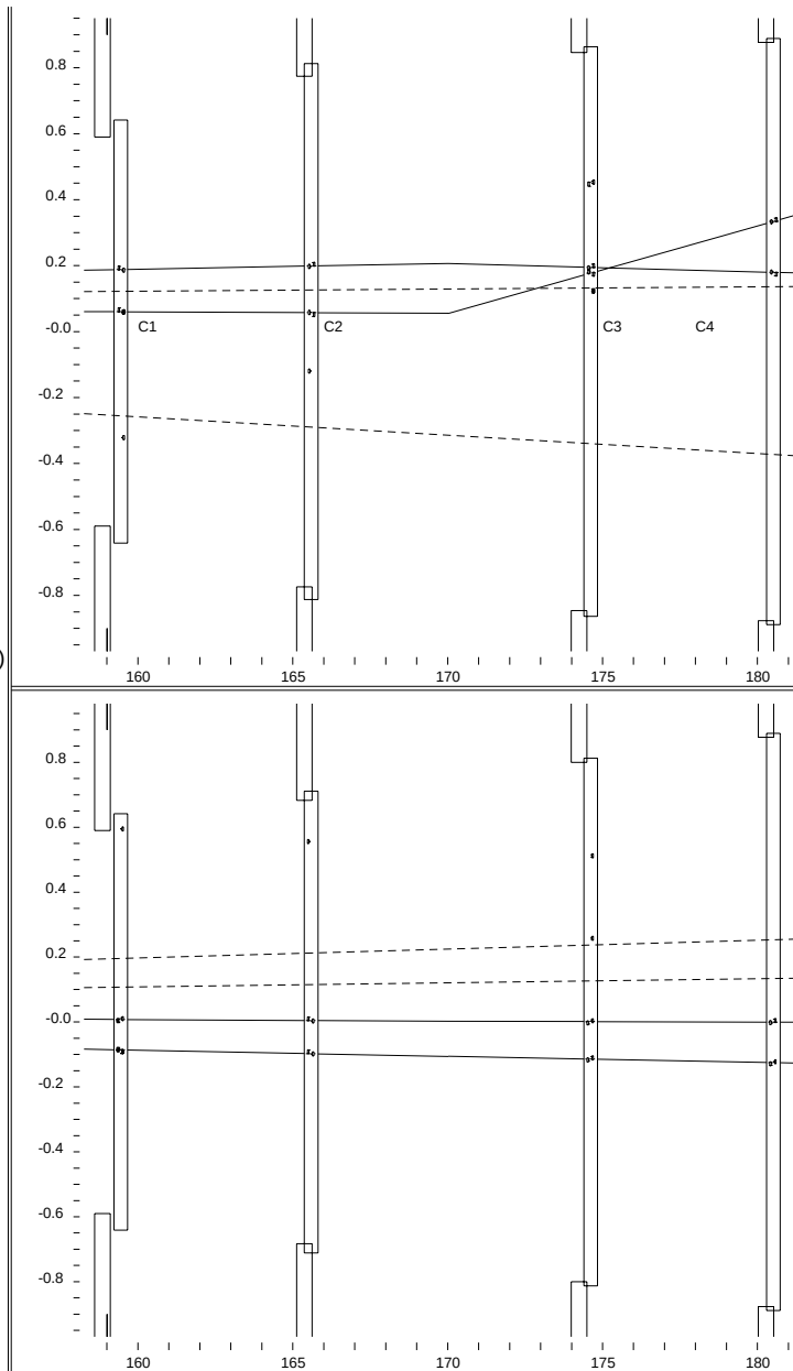
Figure 5.2: Event display of drift chambers. Upper plot is X-view, lower plot is Y-view. Solid lines are reconstructed tracks. Dashed lines are reconstructed photon trajectories.
