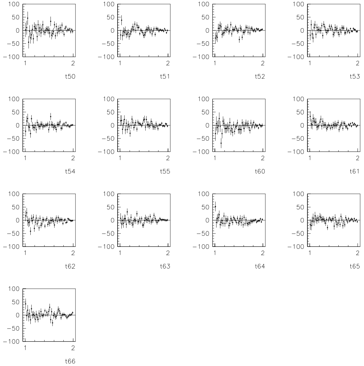
Figure 44: Uncorrected moments t'_{\ell m} for \ell = 5, 6 , m = 0, \dots, \ell , as a function of the K_s^0 K_s^0 invariant mass ( x -axis).
