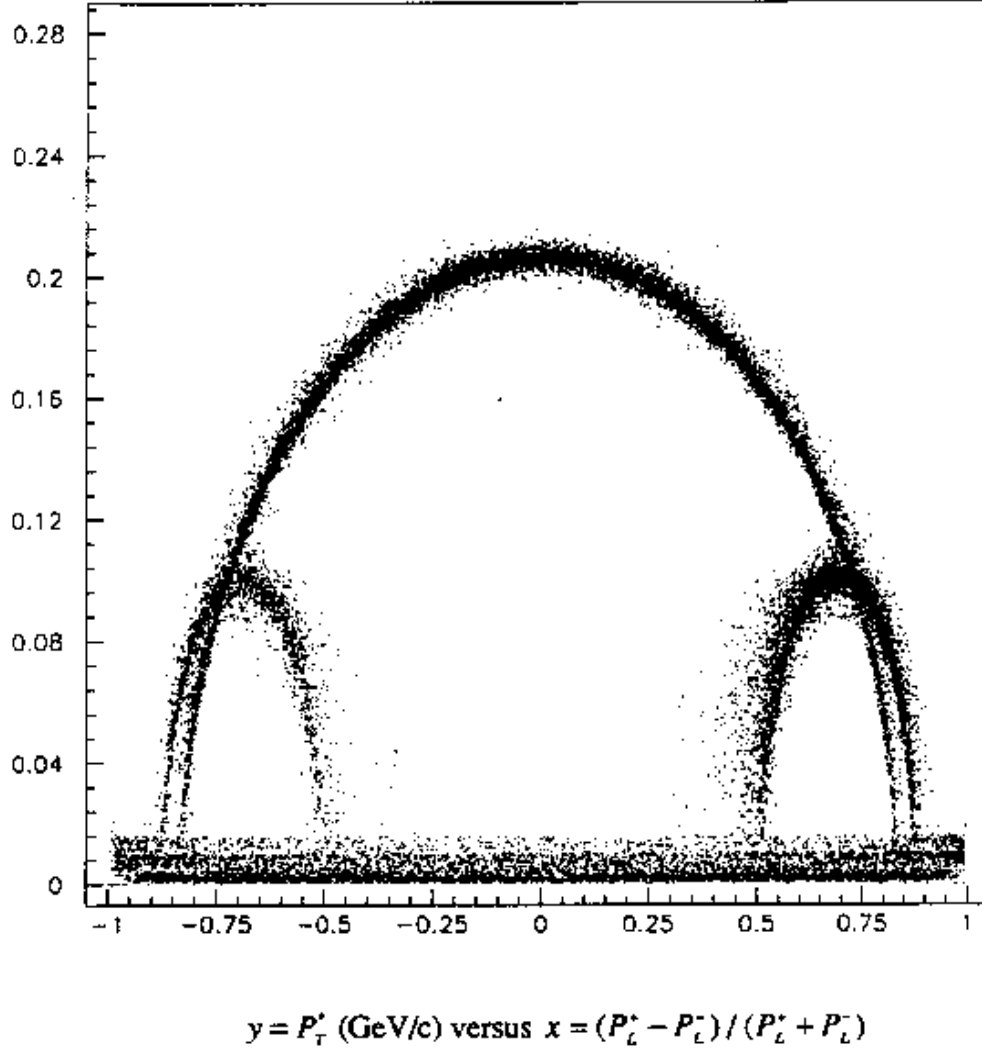
Figure 16: P_T^* versus (P_L^+ - P_L^-)/(P_L^+ + P_L^-) for vertices formed by a pair of oppositely charged particles reconstructed in the JGGS. P_T^* is the transverse momentum, and P_L^+ , P_L^- are the longitudinal momenta of the positive and negative particles, respectively, defined with respect to the momentum sum of the pair. The large ellipse corresponds to K_s^0 \rightarrow \pi^+ + \pi^- decays. The smaller ellipses on the right and left correspond to \Lambda^0 \rightarrow p + \pi^- and \bar{\Lambda}^0 \rightarrow \bar{p} + \pi^+ decays, respectively. Photon conversions to e^+e^- pairs in material contribute the band at small P_T^* .
