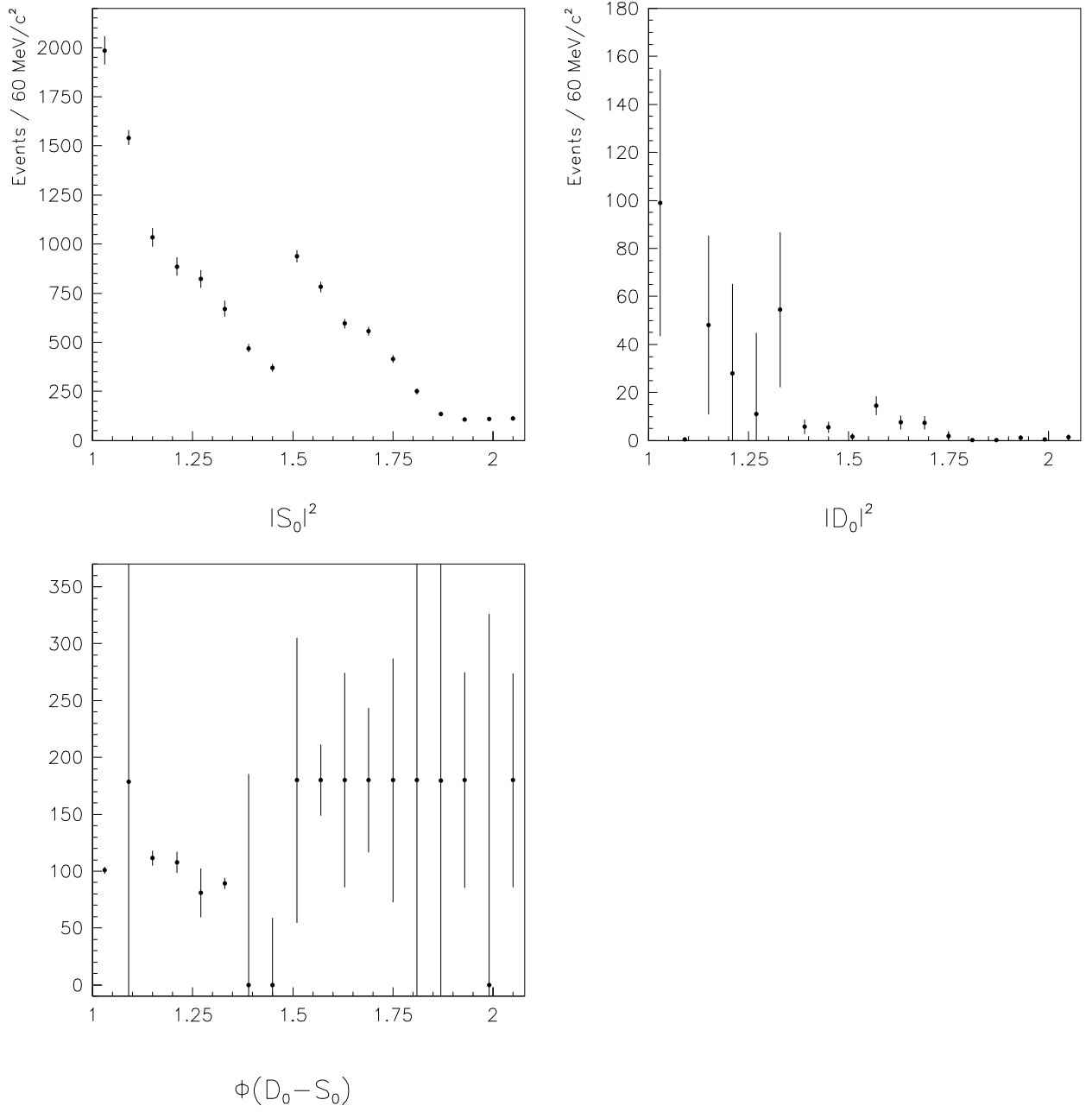
Figure 41: Number of events in the \mathcal{S}_0^- and \mathcal{D}_0^- waves, from maximum likelihood, as a function of the K_s^0 K_s^0 invariant mass ( x -axis). Comparing to fig.38, we see that within error bars both methods give the same amounts for each wave, although maximum likelihood is a better estimation of the parameters used to describe the intensity distribution.
