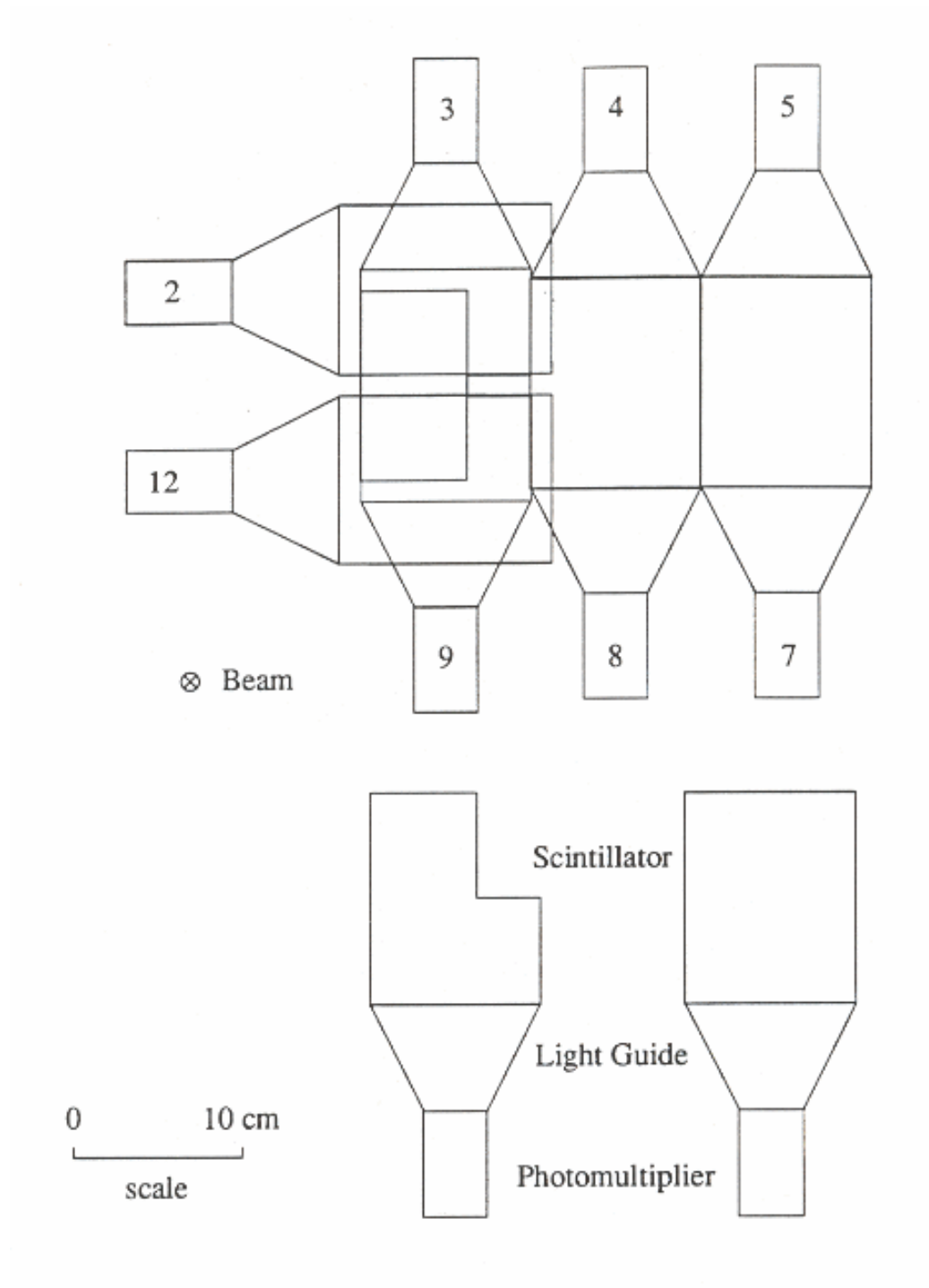
Figure 8: The forward hodoscope (top), and the two types of counters used in it (bottom).
