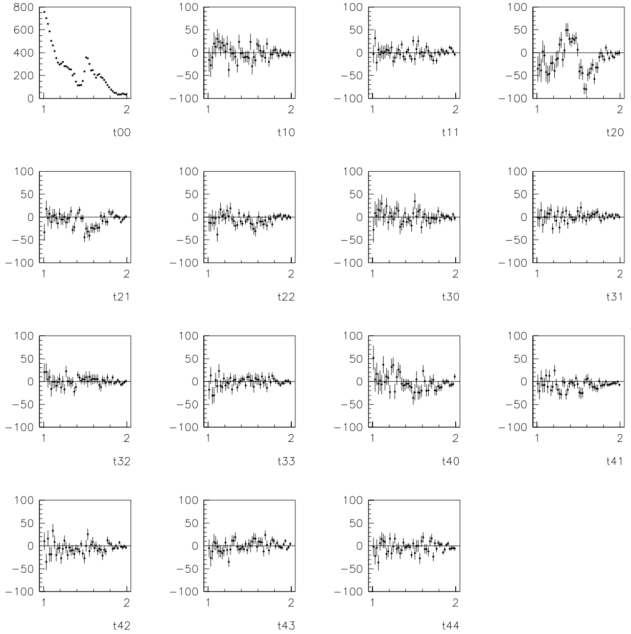
Figure 43: Uncorrected moments t'_{\ell m} for \ell = 0, \dots, 4 , m = 0, \dots, \ell , as a function of the K_s^0 K_s^0 invariant mass ( x -axis).
