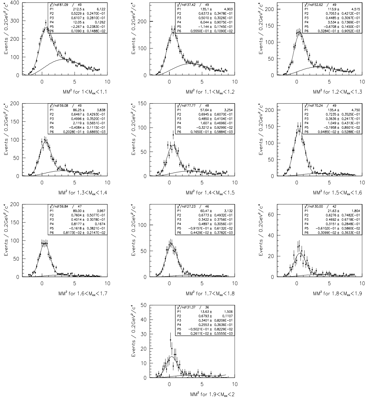
Figure 22: Fit to the missing mass squared peak, in 100 \text{ MeV}/c^2 bins of the K_s^0 K_s^0 invariant mass. As we can see, the number of background events decreases for higher masses.
