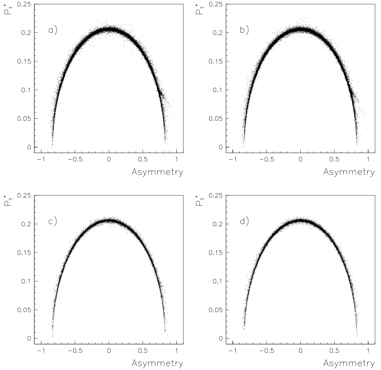
Figure 29: Asymmetry versus P_T^* for the two K_s^0 's in the selected events, (a-b) before kinematical cuts, and (c-d) after the kinematical cuts. We can see how much the sample cleans after these cuts.
