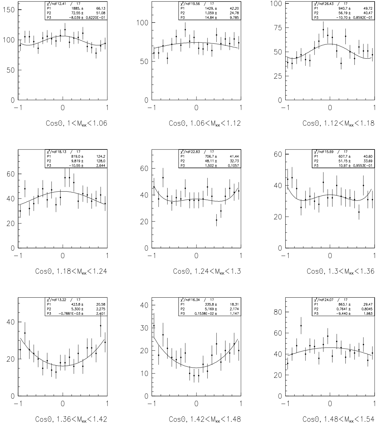
Figure 37: Fits to the \cos\theta distributions using only two waves.
