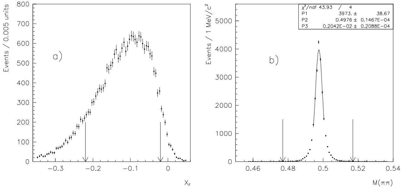
Figure 21: (a) x_F for events that passed the veto-cut, the arrows show the region used for the analysis. (b) \pi^+ \pi^- invariant mass; the cut here was used to remove the tails in mass from PASS2 reconstruction.
