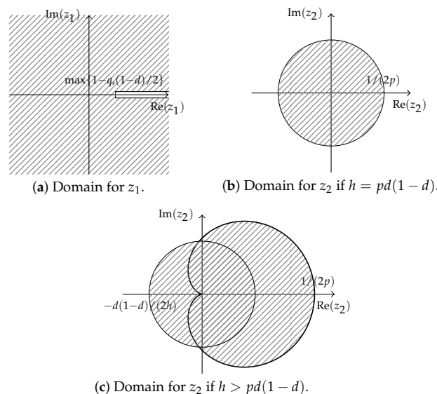
Figure 1. Domains for variables z_1 and z_2 in (6).
