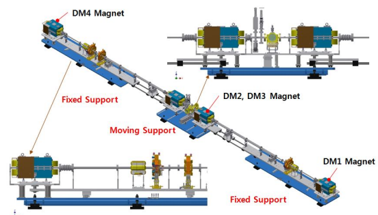
Figure 3: 3D modelling of BC support system.
