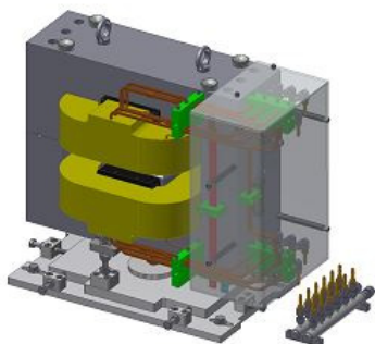
Figure 4: 3D modelling of Dipole Magnet D1.
