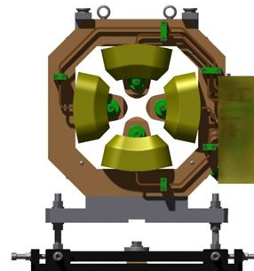
Figure 5: 3D modelling of Quad. Magnet Q11.
