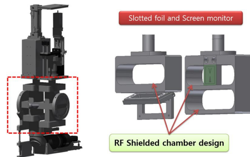
Figure 8: Design of the RF shielded chamber.
