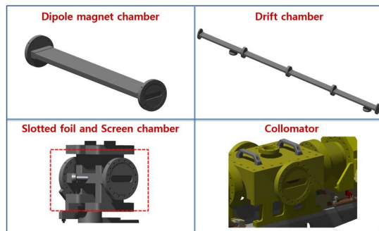
Figure 7: 3D modelling of unified beam chamber.
