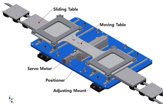
Figure 6: Component of moving support.
