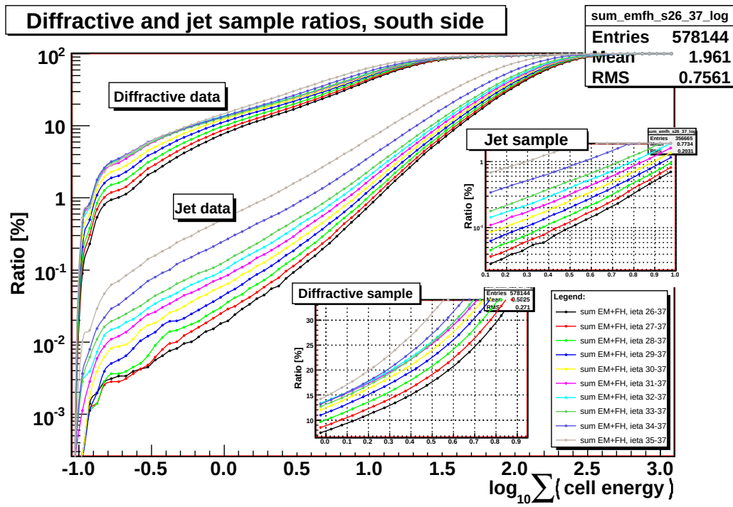
Figure 5.31: The percentage of number of events under a cut (represented by x-axis) to the total number of events for inclusive (in the lower part) and south diffractive (in the upper part) sample. The plots show the energy sums of calorimeter cells in ieta intervals up to 37.
