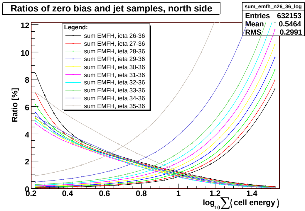
Figure 5.17: The percentage of number of events under/above a cut (which is represented by x-axis) to the total number of events for inclusive (on the right side) and zero bias (on the left side) sample. The ratio is shown under a cut for inclusive sample and above the cut for zero bias sample. The plots show the energy sum of calorimeter cells in ieta intervals up to 36 with LM gap on the north side.
