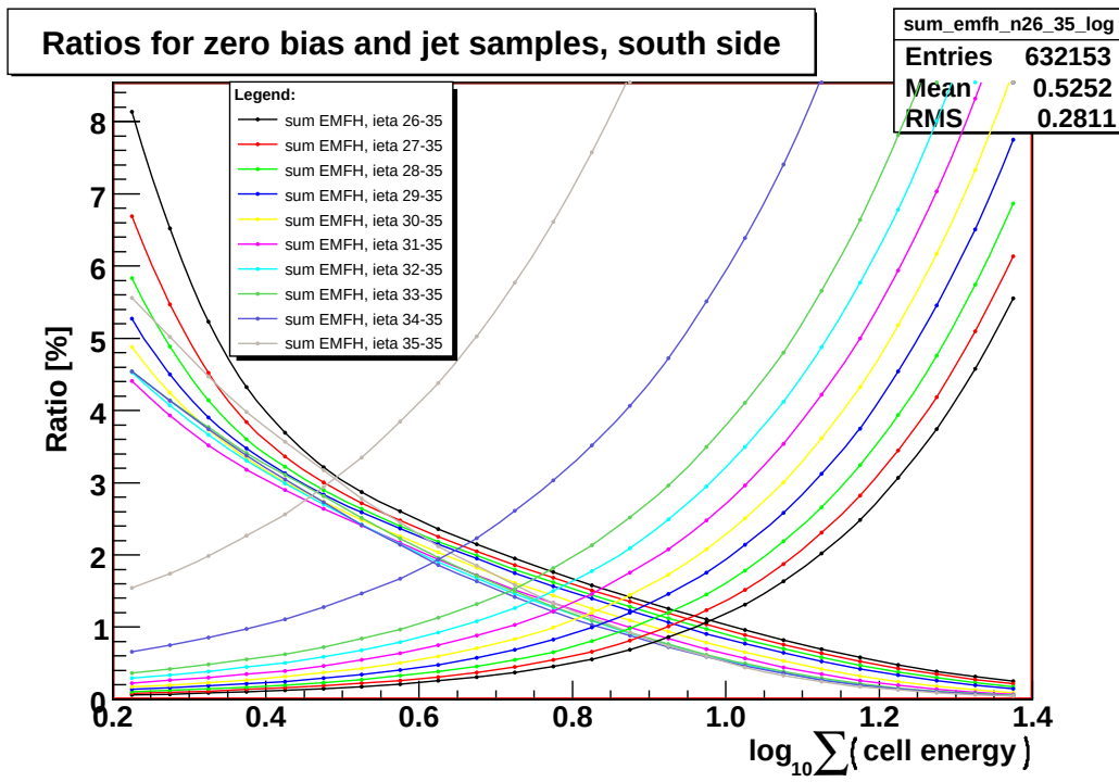
Figure 5.15: The percentage of number of events under/above a cut (which is represented by x-axis) to the total number of events for inclusive (on the right side) and zero bias (on the left side) sample. The ratio is shown under a cut for inclusive sample and above the cut for zero bias sample. The plots show the energy sum of calorimeter cells in ieta intervals up to 35 with LM gap on the south side.
