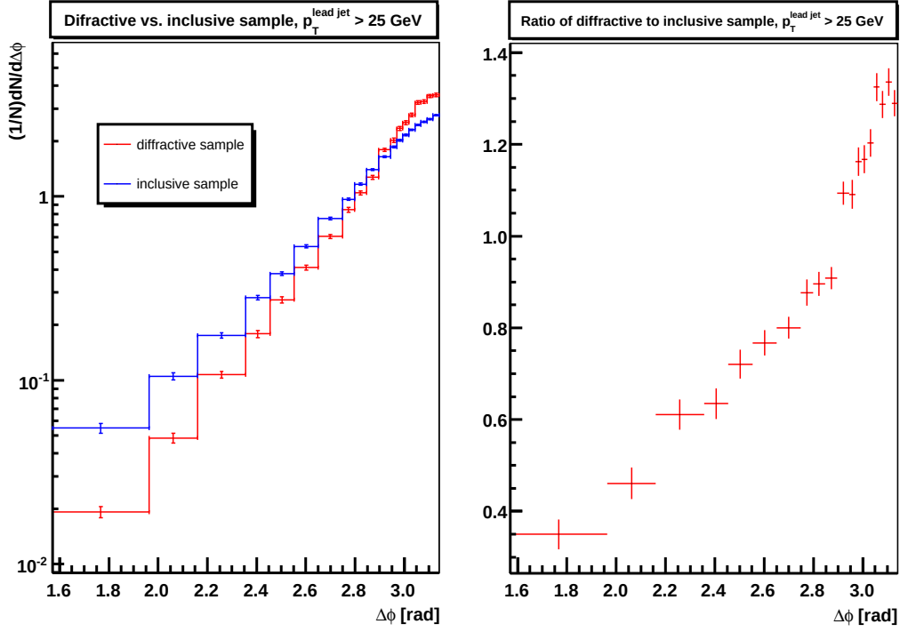
Figure 6.2: Uncorrected \Delta\phi distributions of inclusive and diffractive samples for events with leading jet p_T > 25 \text{ GeV} . On the right, the ratio of the two distributions is given.
