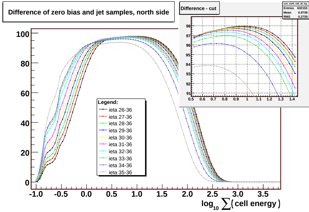
Figure 5.23: F_1 distribution for cell sums within ieta intervals up to 36, north side.
