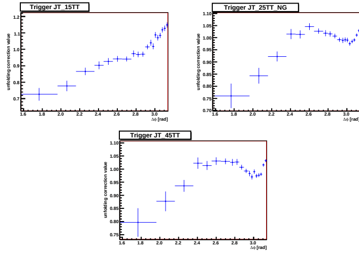
Figure 6.12: Unsmearing corrections of inclusive sample.
