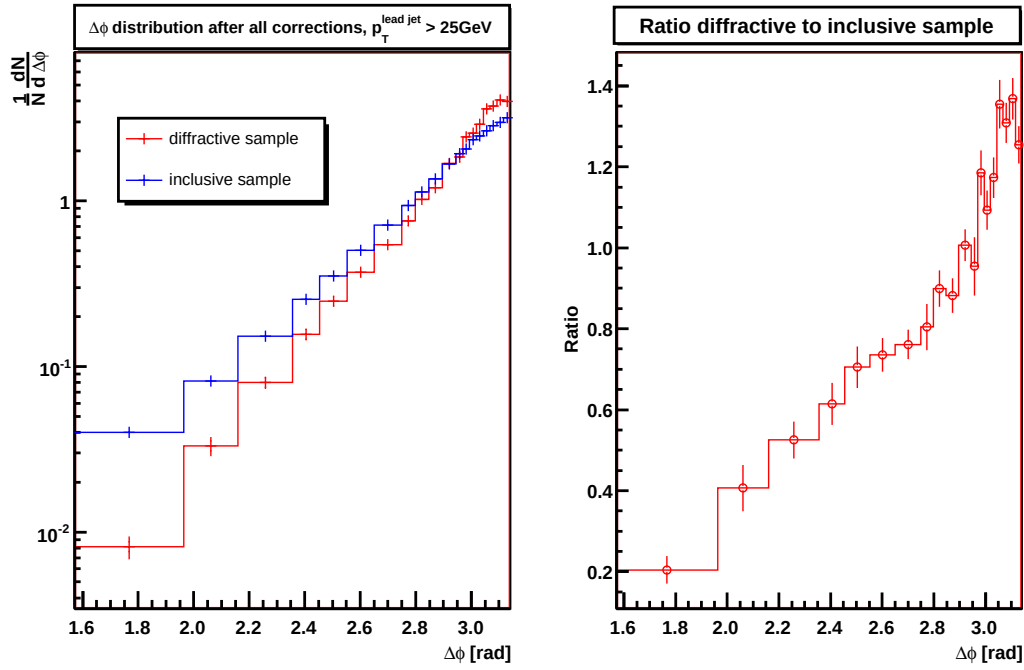
Figure 6.14: Final \Delta\phi distribution after all corrections for jets with p_T > 25\text{GeV} .
