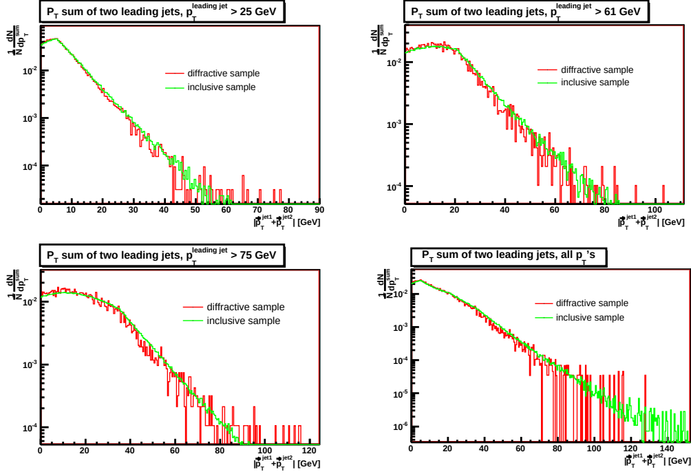
Figure 8.2: A sum of p_T 's of first two leading jets for inclusive and diffractive samples.
