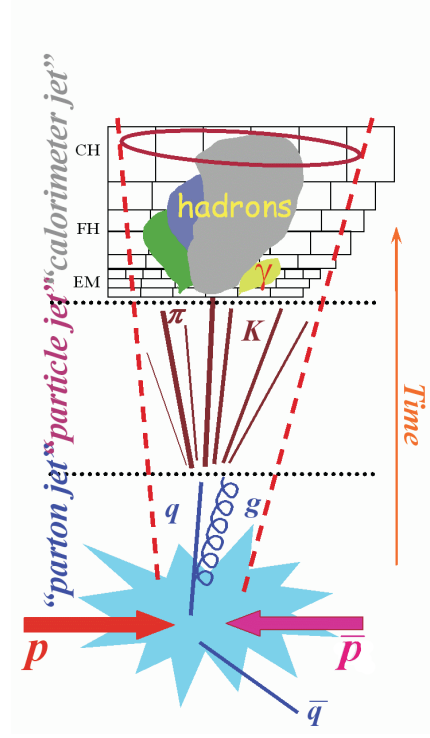
Figure 2.6: Jet propagation through different definition levels.
