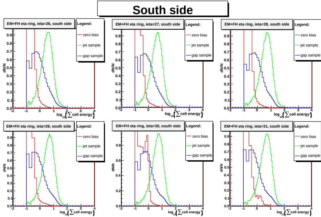
Figure 5.3: Sum of calorimeter cells with a given \eta . Events with LM south turned off.
