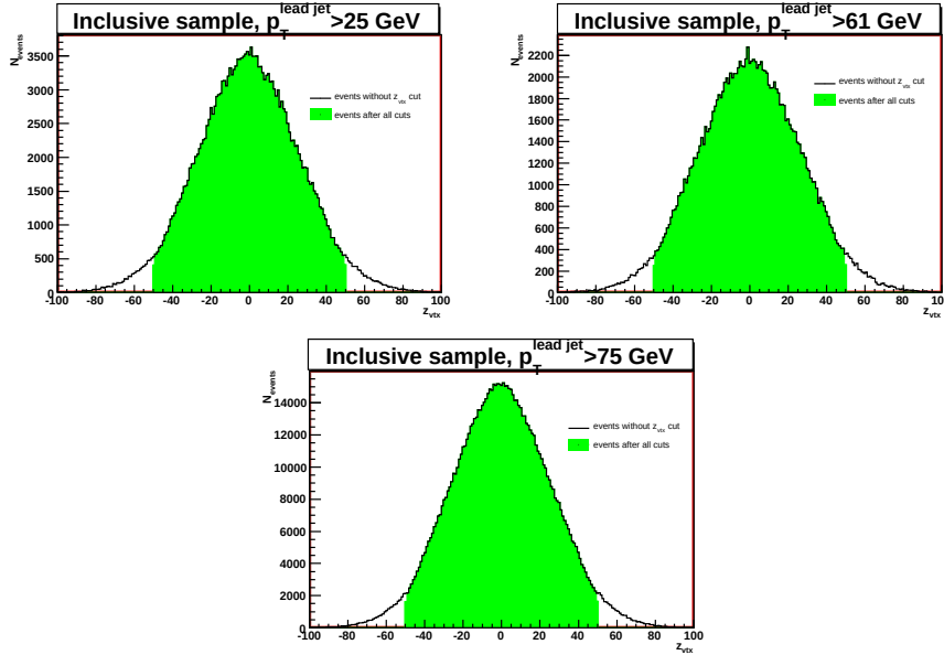
Figure 4.12: Distribution of z-coordinate of primary vertex. Green area shows events after both primary vertex cuts (number of vertices and z cut) for events from inclusive sample. Black curve shows the distribution for inclusive events without any primary vertex cut.
