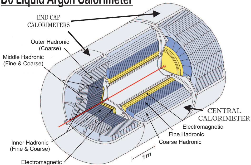
Figure 3.4: D0 calorimeter
