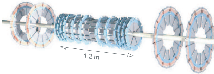
Figure 3.2: D0 tracking system.
