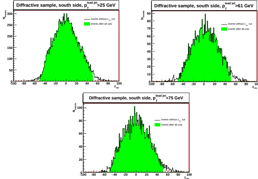
Figure 4.13: Distribution of z-coordinate of primary vertex. Green area shows events after both primary vertex cuts (number of vertices and z cut) for events with gap on the south side of the calorimeter. Black curve shows the distribution for south diffractive events without any primary vertex cut.
