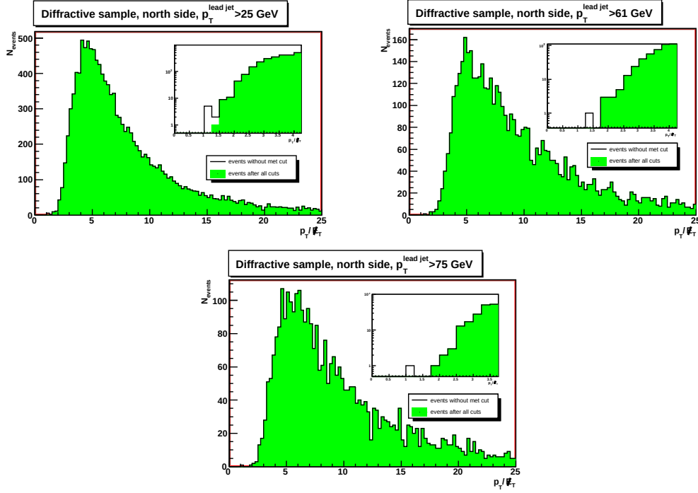
Figure 4.11: Distribution of missing E_T for events with gap on the north side of the calorimeter.
