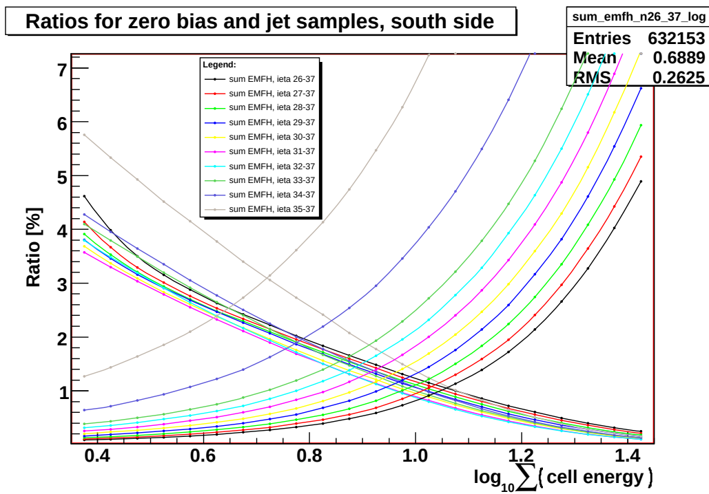
Figure 5.13: The percentage of number of events under/above a cut (which is represented by x-axis) to the total number of events for inclusive (on the right side) and zero bias (on the left side) sample. The ratio is shown under a cut for inclusive sample and above the cut for the noise sample. The plots show the energy sum of calorimeter cells in ieta intervals up to 37 with LM gap on the south side.
