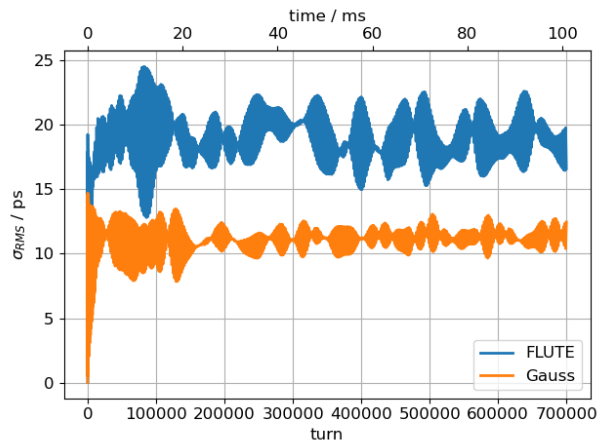
Figure 2: Bunch length \sigma_{STD} .
