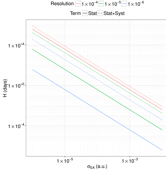
Fig. 1. Required beam time as a function of \hat{A} precision for three different beam current resolutions. Solid lines are obtained for the inherent slope variation \sigma^2[\beta] = \text{s}^{-2} and single polarisation state time h = 15 min, while the dashed lines are for \sigma^2[\beta] = 10^{-15} \text{ s}^{-2} and h_{\text{best}} from Table II.
