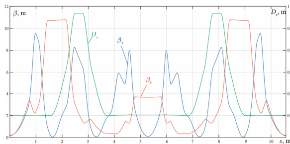
Figure 2: Twiss functions and dispersion.
