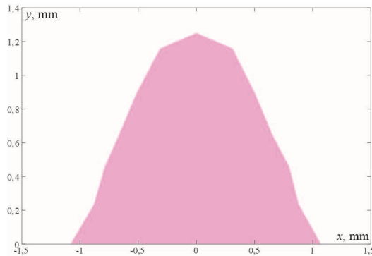
Figure 3: Dynamic aperture (for 1000 turns).
