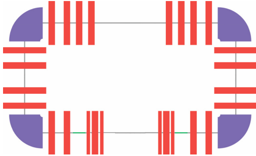
Figure 1: Basic magnet lattice of storage ring.
