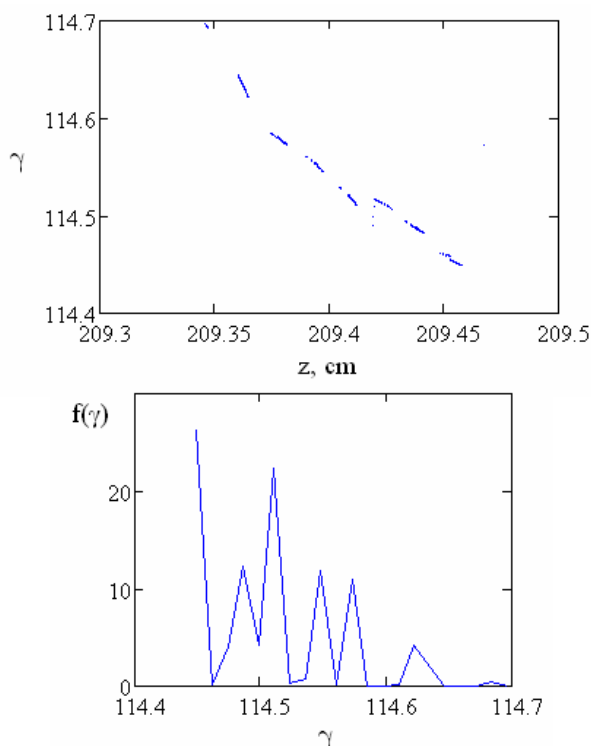
Figure 6: The beam dynamics simulation results for the linac: output bunch phase space (top) and energy spectrum (bottom).
