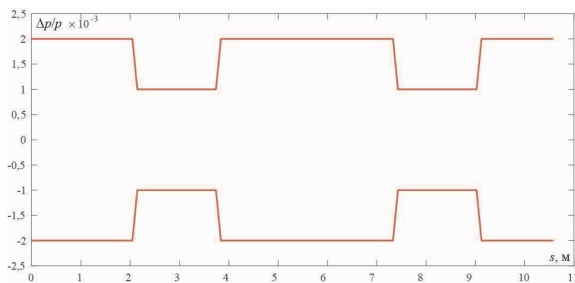
Figure 4: Momentum acceptance ( U_{\text{rf}} = 300 kV).
