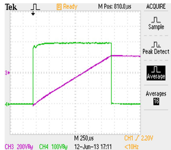
Figure 4: Pulse voltage (green) and regulator voltage (purple) with the regulator, 200 V/div, 250 \mu s/div.
