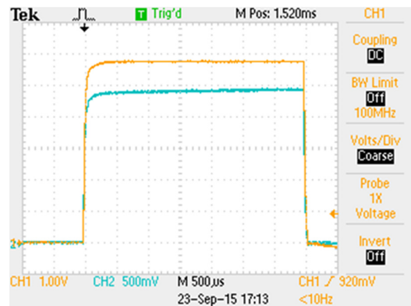
Figure 2: Voltage and current waveforms of the ESS modulator.
