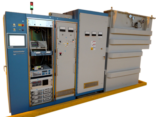
Figure 1: ESS Klystron Test Stand, showing controls and auxiliary supplies in the left cabinet, the high voltage power supply (center-left), the high voltage modulator cabinets (center-right), and transformer (far right).
