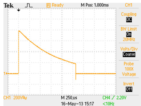
Figure 3: Pulse voltage without the regulator, 200 V/div, 250 \mu s/div.
