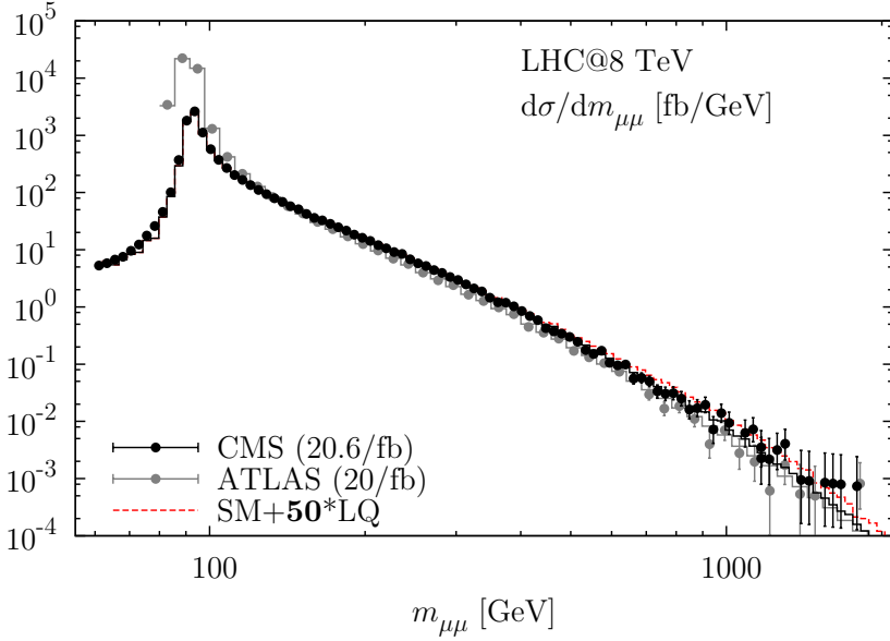
Fig. 10: The contribution of leptoquark t -channel exchange to dilepton spectra compared with CMS (Fig. 2 of Ref. [90]) and ATLAS (Fig. 1 and 2 of Ref. [91]) data and standard-model expectations. The simulated leptoquark contribution in CMS acceptance ( p_{Te} > 35 GeV, p_{T\mu} > 45 GeV, |\eta_\ell| \lesssim 2.5 ) is added to CMS standard-model expectation. The ATLAS acceptance ( p_{Te} > 40 , 30 GeV, p_{T\mu} > 25 GeV, |\eta_\ell| \lesssim 2.5 ) is slightly larger than the CMS one in the \mu\mu channel. Finite efficiencies that would reduce somewhat the leptoquark signal actually seen in detectors are neglected. In the \mu\mu channel the signal is magnified by a factor of 50 to become visible on top of the standard-model expectation.
