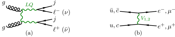
Fig. 9: (a) QCD pair production constraining leptoquark masses for a given branching fraction to leptons (neutrinos) and jets. (b) Contribution of leptoquark t -channel exchange to dileptons. For a fixed mass, it bounds their couplings to fermions.
