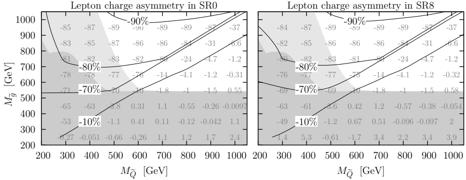
Fig. 21: Lepton charge asymmetry of the same-sign dilepton signal of R-parity violation (electrons or muons only). Full minimal flavour violation is imposed and only \tilde{d}_R and \tilde{g} contributions to the top pair production are included. Excluded regions are shaded (see Fig. 18).
