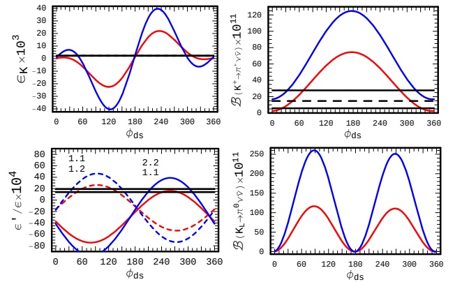
FIG. 3: (a) \varepsilon_K , (b) \mathcal{B}(K^+ \rightarrow \pi^+ \nu \bar{\nu}) , (c) \text{Re}(\varepsilon'/\varepsilon) and (d) \mathcal{B}(K_L \rightarrow \pi^0 \nu \bar{\nu}) vs \phi_{ds} , for r_{ds} = 4 and 6 \times 10^{-4} and m_{t'} = 300 GeV. Larger r_{ds} gives stronger variation, and horizontal bands are current ( 1\sigma ) experimental range [8] (the bound for (d) is outside the plot). For (c), solid (dashed) lines are for R_6 = 2.2 , R_8 = 1.1 ( R_6 = 1.1 , R_8 = 1.2 ).
