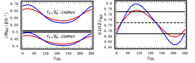
FIG. 4: (a) \Delta m_{B_d} and (b) \sin 2\Phi_{B_d} vs \phi_{db} for r_{db} = 8 and 12 \times 10^{-4} , with V_{td}^* V_{tb} \equiv r_{db} e^{i\phi_{db}} . Larger r_{db} gives stronger variation, and horizontal bands are the experimental range [8].
