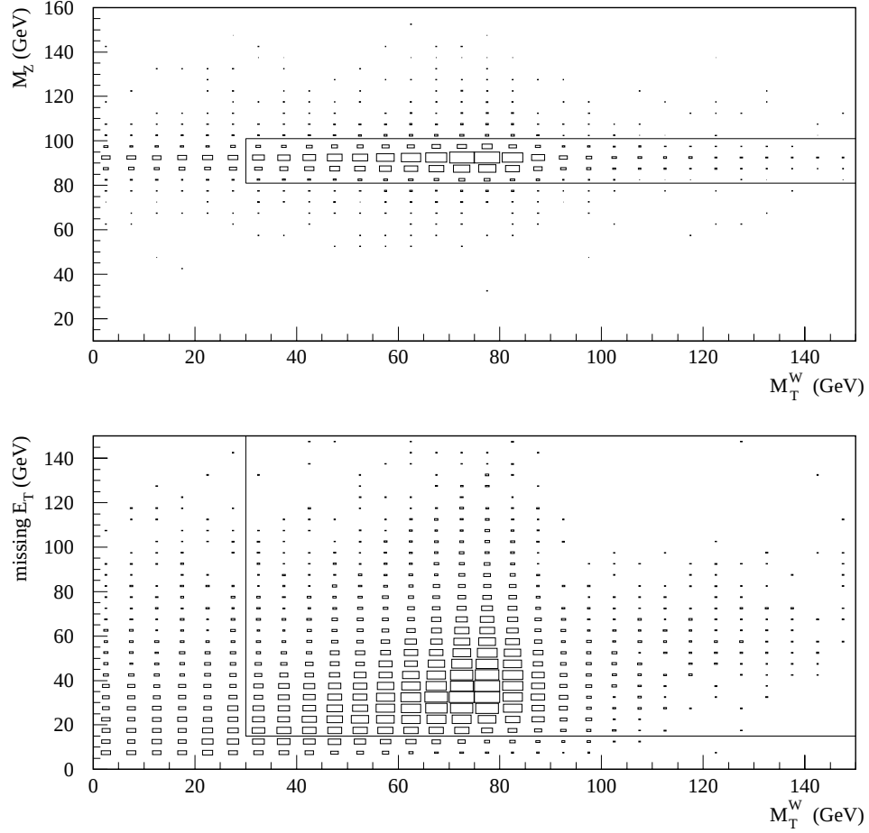
Figure 6.5: Distributions from Zeppenfeld-DIPS Monte Carlo for Standard Model WZ \rightarrow e\bar{\nu}ee signal events after all cuts except mass and \cancel{E}_T have been applied. The lines show where the mass and \cancel{E}_T cuts are applied to data.
