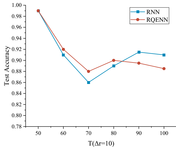
Figure 8. The median of the best test accuracy of RQENN and RNN in different length intervals. Both models are trained for 10 epochs on each interval.
