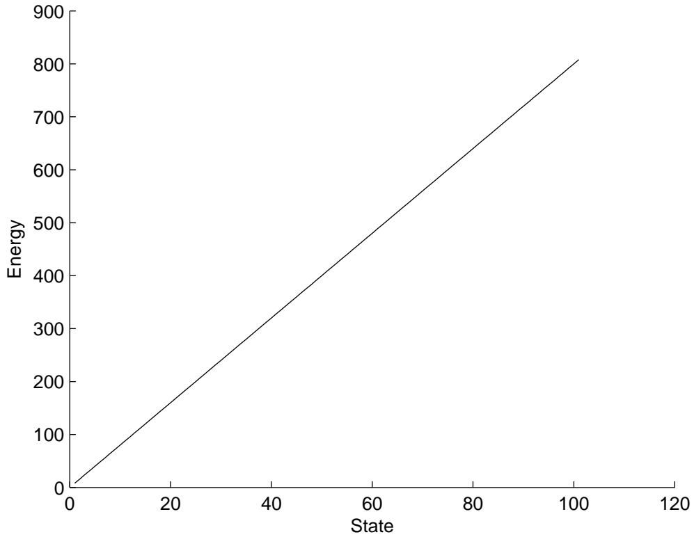
Figure 8.1: Eigenvalue spectrum
