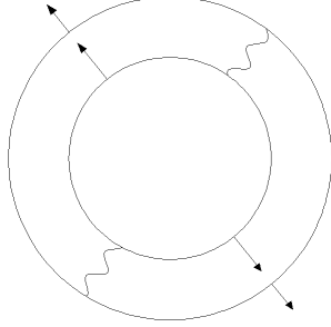
Figure 8.3: Low Energy Modes
