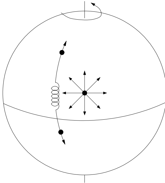
Figure 5.1: Dipole constrained to move on the surface of a Sphere, in the presence of a magnetic monopole
