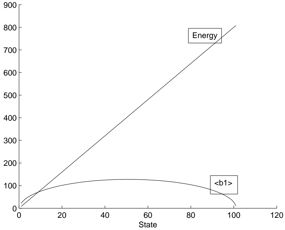
Figure 8.2: Eigenvalue spectrum, and \langle b_1 \rangle
