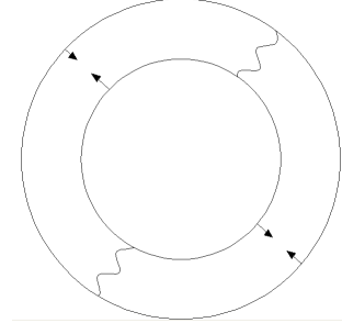
Figure 8.4: High Energy Modes
