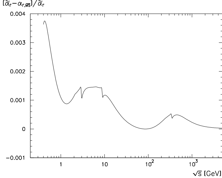
FIG. 7. The relative difference between the calculation of \alpha_{F,q}^{NS}(s) in the analytic extension of the \overline{\text{MS}} scheme and the standard treatment of masses in the \overline{\text{MS}} scheme. The discontinuities are due to the mismatch between the s/m^2 and m^2/s expansions of the functions F and G .
