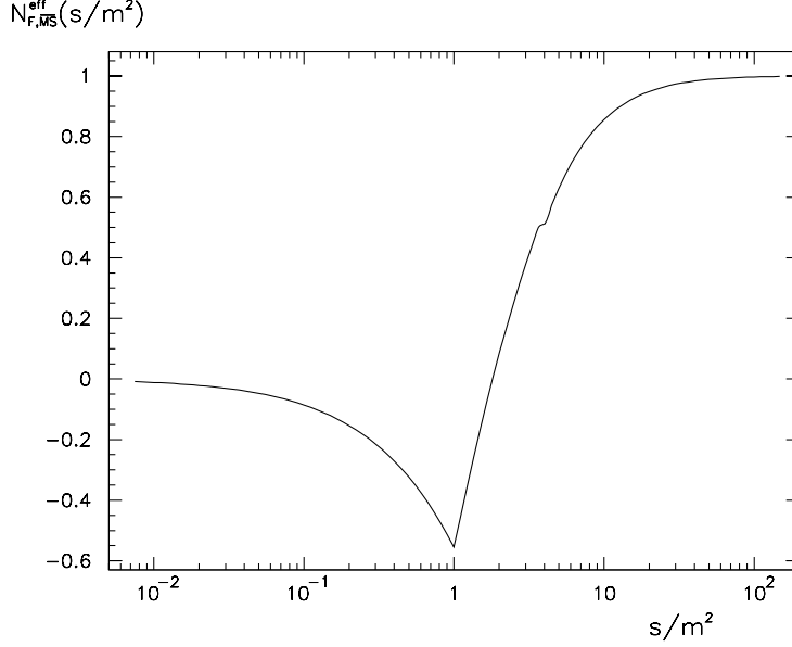
FIG. 6. The effective contribution to N_F in the \alpha_s^2 -coefficient in the standard \overline{MS} scheme from a quark with mass m as a function of s/m^2 (using \mu = \sqrt{s} ). The discontinuity between the two expansions in s/m^2 and m^2/s can be seen at the nonanalytic point s/m^2 = 4 .
