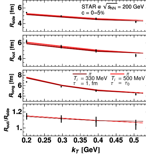
Fig. 2. The pion HBT radii R_{\text{side}} , R_{\text{out}} , R_{\text{long}} , and the ratio R_{\text{out}}/R_{\text{side}} for central collisions. The darker (lighter) lines describe the results with (without) FS+SE. The data from [21].
