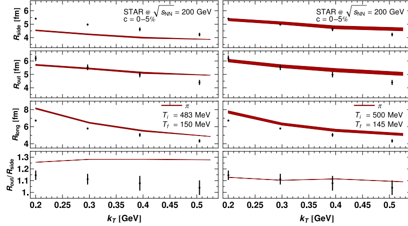
Fig. 1. The pionic HBT radii R_{\text{side}} , R_{\text{out}} , R_{\text{long}} , and the ratio R_{\text{out}}/R_{\text{side}} for central collisions, shown as the functions of the average momentum of the pair and compared to the RHIC Au+Au data [21]. The left part illustrates our best results obtained with the standard Glauber initial conditions [14], while the right part illustrates the results obtained with the Gaussian initial conditions [10].
