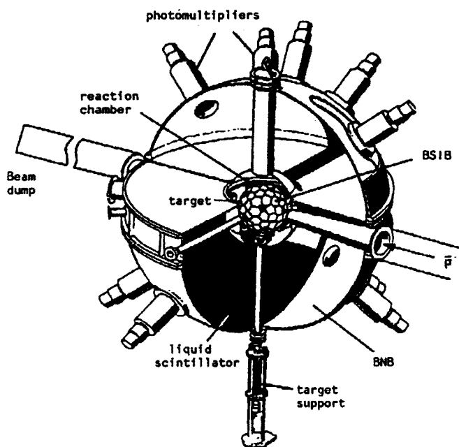
Fig. 9. Schematic drawing of the 4\pi Berlin Neutron Ball (BNB) and the 4\pi Berlin Silicon Ball (BSIB) used during recent PS208 experiment. (From [77]).
